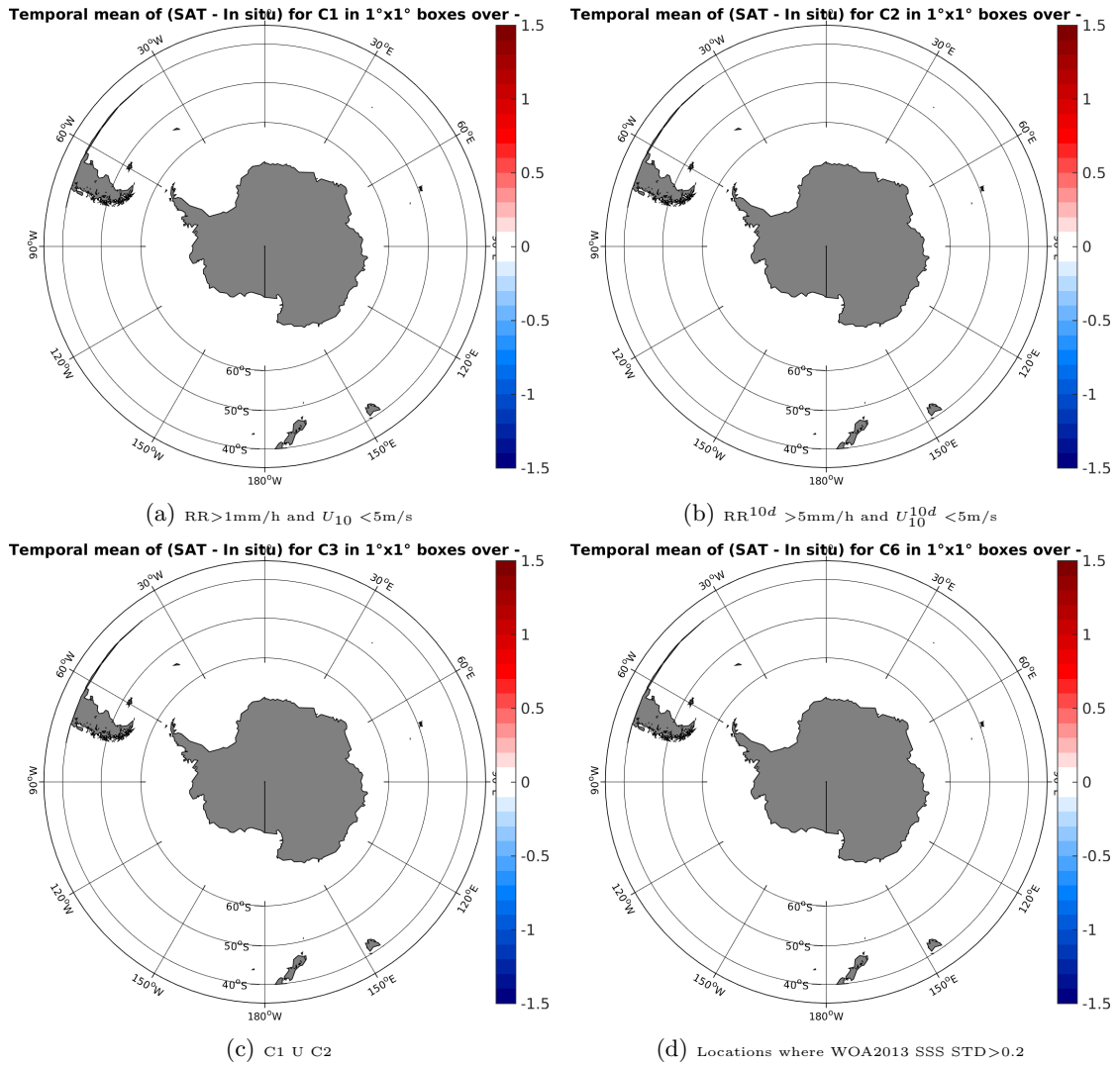
Figure 11: Temporal mean gridded over spatial boxes of size 1^\circ \times 1^\circ of \Delta SSS (SMAP-L2-JPL-V4 - Surface drifters) for 4 different subdatasets corresponding to: RR > 1mm/h and U_{10} < 5\text{m/s} (a), RR^{10d} > 5\text{mm/h} and U_{10}^{10d} < 5\text{m/s} (b), C1 U C2 (c), Locations where WOA2013 SSS STD > 0.2 (d).
