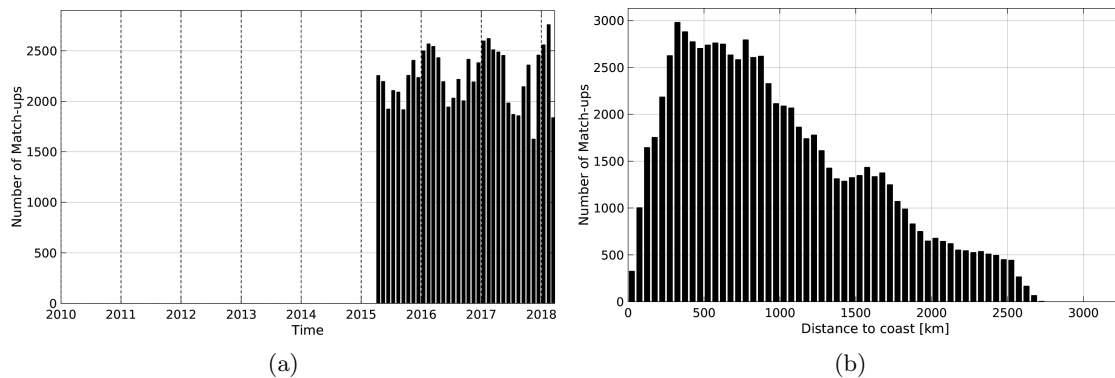
Figure 1: Number of match-ups between Argo and SMAP-L2-JPL-V4 SSS as a function of time (a) and as function of the distance to coast (b) over the Roaring Forties and Furious Fifties Pi-MEP region and for the full satellite product period.
