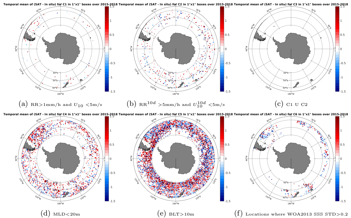
Figure 12: Temporal mean gridded over spatial boxes of size 1^\circ \times 1^\circ of \Delta\text{SSS} (SMAP-L2-JPL-V4 - Argo) for 6 different subdatasets corresponding to: RR > 1\text{mm/h} and U_{10} < 5\text{m/s} (a), RR^{10d} > 5\text{mm/h} and U_{10}^{10d} < 5\text{m/s} (b), C1 U C2 (c), MLD < 20\text{m} (d), BLT > 10\text{m} (e), Locations where WOA2013 SSS STD > 0.2 (f).
