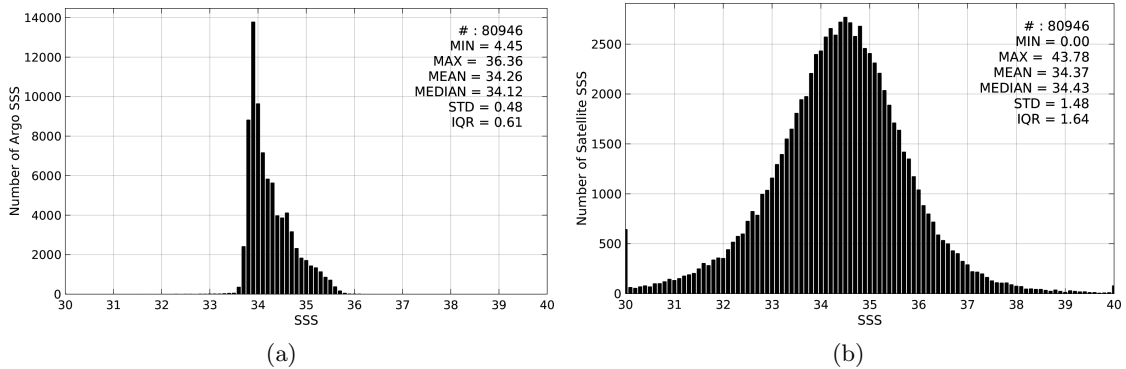
Figure 2: Histograms of SSS from Argo (a) and SMAP-L2-JPL-V4 (b) considering all match-up pairs per bins of 0.1 over the Roaring Forties and Furious Fifties Pi-MEP region and for the full satellite product period.
