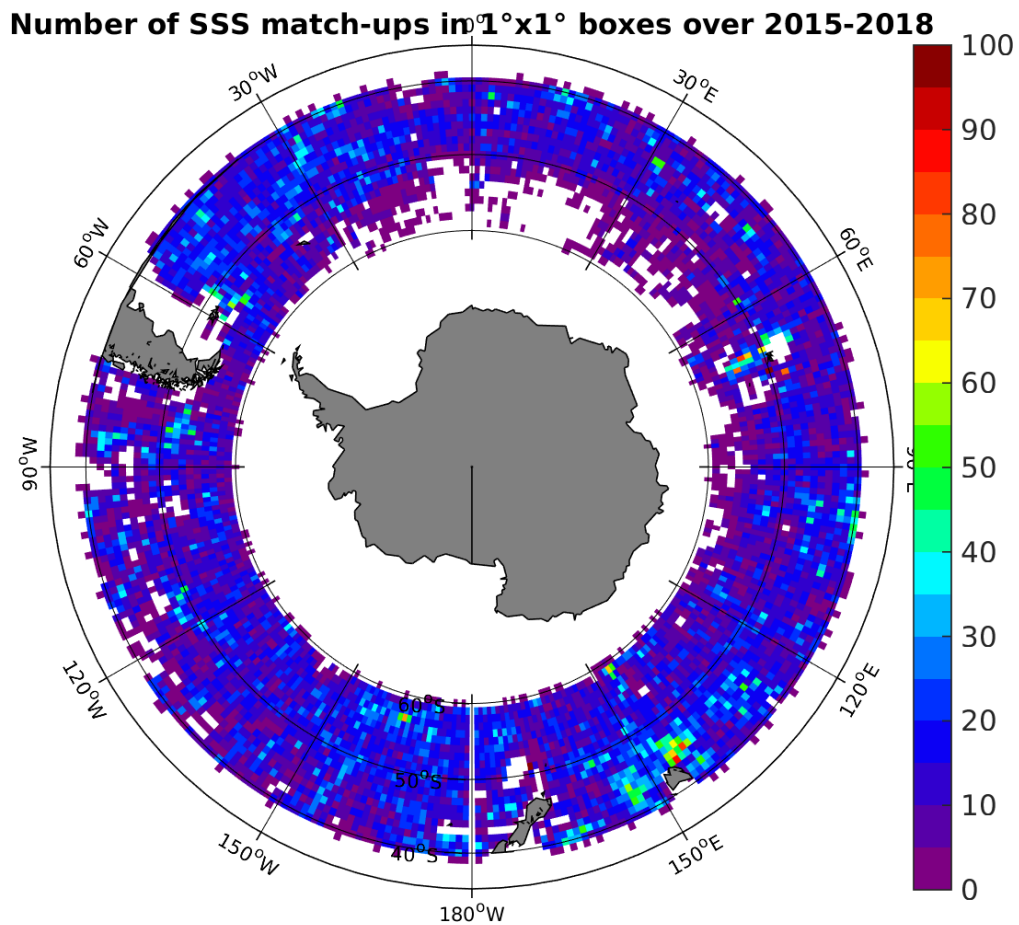
Figure 4: Number of SSS match-ups between Argo SSS and the SMAP-L2-JPL-V4 SSS product for the Roaring Forties and Furious Fifties Pi-MEP region over 1^\circ \times 1^\circ boxes and for the full satellite product period.
