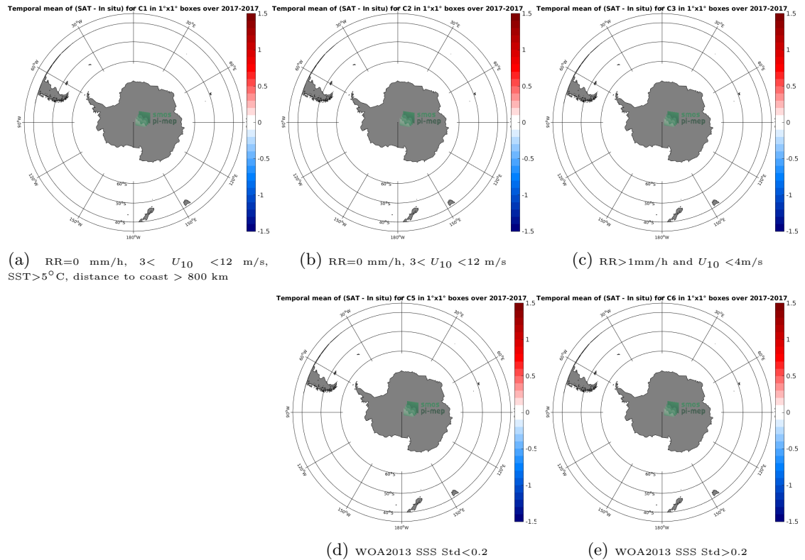
Figure 12: Temporal mean gridded over spatial boxes of size 1^{\circ}\times 1^{\circ} of \Delta SSS (SMAP-L2-JPL-V4.3 - TSG-GOSUD-Research-vessel) for 5 different subdatasets corresponding to: RR=0 mm/h, 3 < U_{10} < 12 m/s, SST > 5^{\circ}\text{C} , distance to coast > 800 km (a), RR=0 mm/h, 3 < U_{10} < 12 m/s (b), RR > 1 mm/h and U_{10} < 4 m/s (c), WOA2013 SSS Std < 0.2 (d), WOA2013 SSS Std > 0.2 (e).
