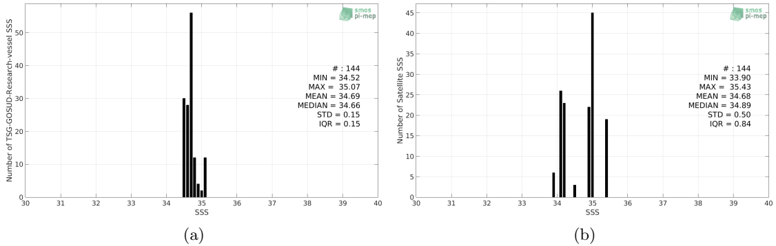
Figure 2: Histograms of SSS from TSG-GOSUD-Research-vessel (a) and SMAP-L2-JPL-V4.3 (b) considering all match-up pairs per bins of 0.1 over the Roaring Forties and Furious Fifties Pi-MEP region and for the full satellite product period.
