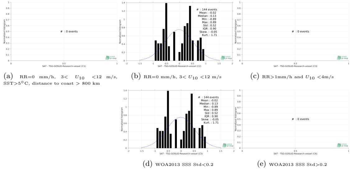
Figure 13: Normalized histogram of \Delta SSS (SMAP-L2-JPL-V4.3 - TSG-GOSUD-Research-vessel) for 5 different subdatasets corresponding to: RR=0 mm/h, 3 < U_{10} < 12 m/s, SST > 5^\circ\text{C} , distance to coast > 800 km (a), RR=0 mm/h, 3 < U_{10} < 12 m/s (b), RR > 1\text{mm/h} and U_{10} < 4\text{m/s} (c), WOA2013 SSS Std < 0.2 (d), WOA2013 SSS Std > 0.2 (e).
