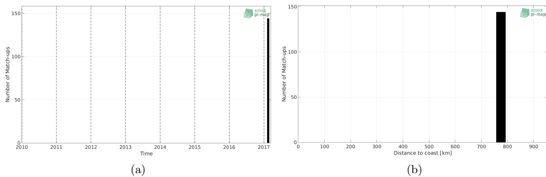
Figure 1: Number of match-ups between TSG-GOSUD-Research-vessel and SMAP-L2-JPL-V4.3 SSS as a function of time (a) and as function of the distance to coast (b) over the Roaring Forties and Furious Fifties Pi-MEP region and for the full satellite product period.
