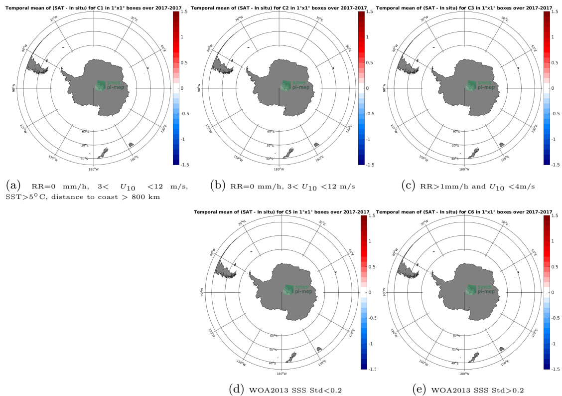
Figure 12: Temporal mean gridded over spatial boxes of size 1^\circ \times 1^\circ of \Delta SSS (SMAP-L2-JPL-V4.3 - TSG-GOSUD-Research-vessel) for 5 different subdatasets corresponding to:RR=0 mm/h, 3 < U_{10} < 12 m/s, SST >5^\circ\text{C} , distance to coast > 800 km (a), RR=0 mm/h, 3 < U_{10} < 12 m/s (b), RR >1 mm/h and U_{10} < 4 m/s (c), WOA2013 SSS Std <0.2 (d), WOA2013 SSS Std >0.2 (e).
