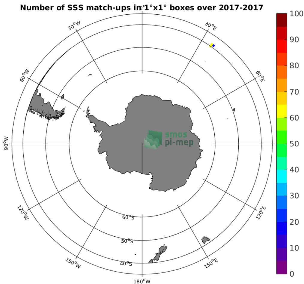
Figure 4: Number of SSS match-ups between TSG-GOSUD-Research-vessel SSS and the SMAP-L2-JPL-V4.3 SSS product for the Roaring Forties and Furious Fifties Pi-MEP region over 1°x1° boxes and for the full satellite product period.
