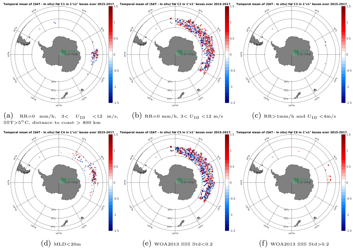
Figure 12: Temporal mean gridded over spatial boxes of size 1^{\circ}\times 1^{\circ} of \Delta\text{SSS} (SMAP-L2-JPL-V4.3 - Sea mammals) for 6 different subdatasets corresponding to:RR=0 mm/h, 3 < U_{10} < 12 m/s, SST >5^{\circ}\text{C} , distance to coast > 800 km (a), RR=0 mm/h, 3 < U_{10} < 12 m/s (b), RR >1 mm/h and U_{10} < 4 m/s (c),MLD <20\text{m} (d),WOA2013 SSS Std <0.2 (e),WOA2013 SSS Std >0.2 (f).
