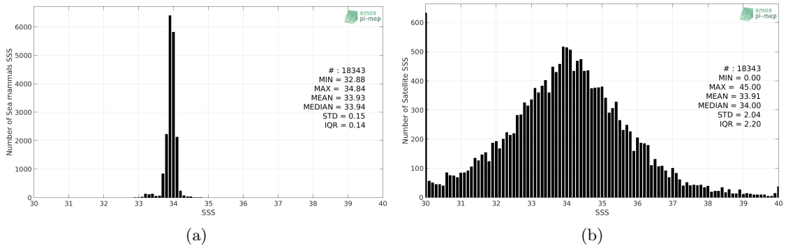
Figure 2: Histograms of SSS from Sea mammals (a) and SMAP-L2-JPL-V4.3 (b) considering all match-up pairs per bins of 0.1 over the Roaring Forties and Furious Fifties Pi-MEP region and for the full satellite product period.
