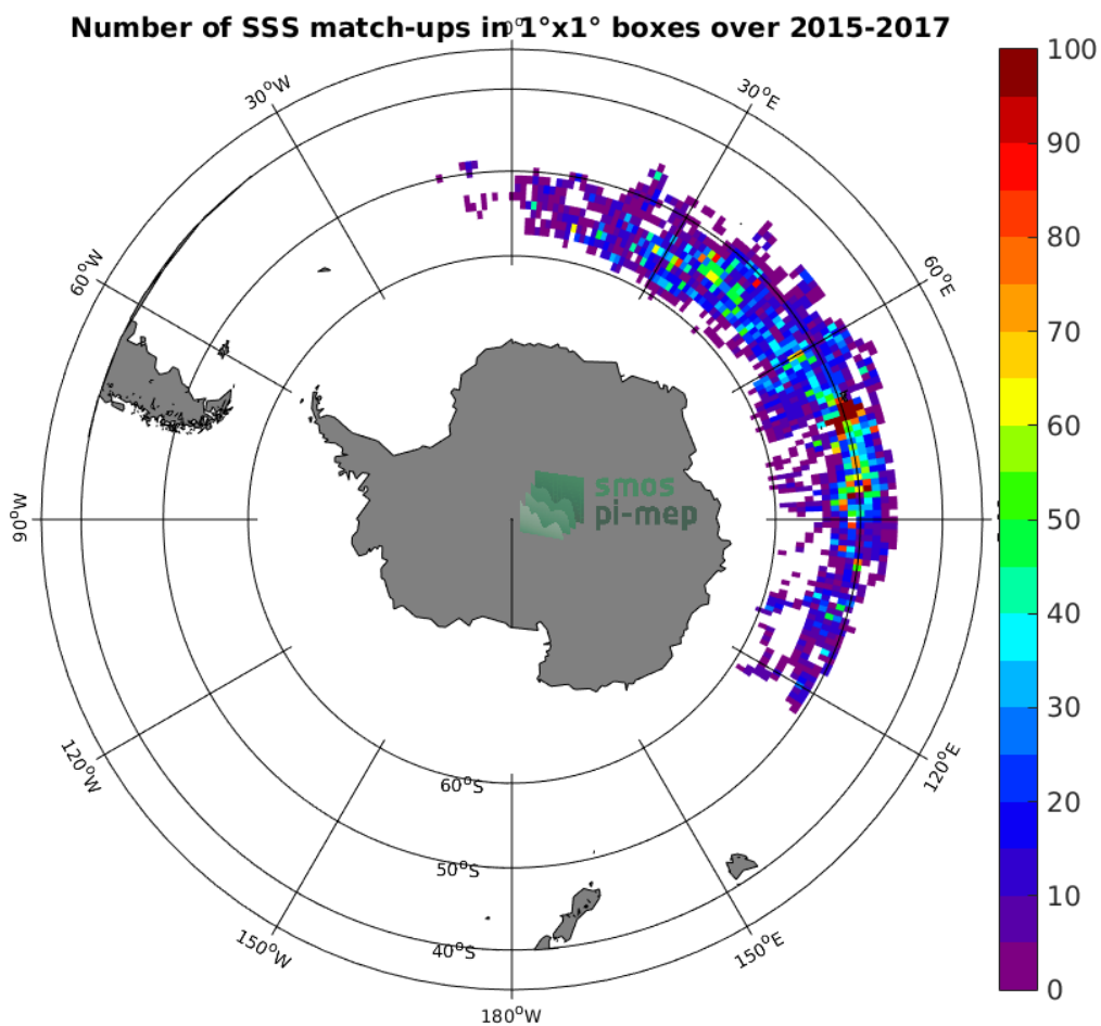
Figure 4: Number of SSS match-ups between Sea mammals SSS and the SMAP-L2-JPL-V4.3 SSS product for the Roaring Forties and Furious Fifties Pi-MEP region over 1°x1° boxes and for the full satellite product period.
