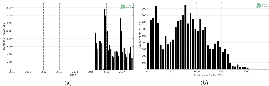
Figure 1: Number of match-ups between Sea mammals and SMAP-L2-JPL-V4.3 SSS as a function of time (a) and as function of the distance to coast (b) over the Roaring Forties and Furious Fifties Pi-MEP region and for the full satellite product period.
