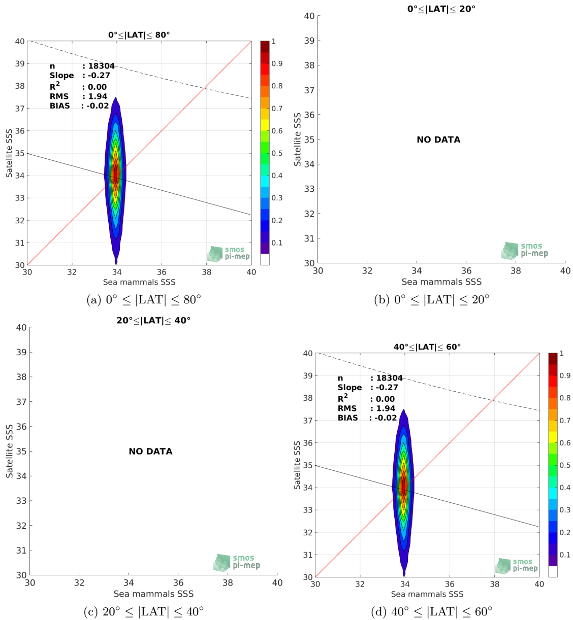
Figure 9: Contour maps of the concentration of SMAP-L2-JPL-V4.3 SSS (y-axis) versus Sea mammals SSS (x-axis) at match-up pairs for different latitude bands. For each plot, the red line shows x=y . The black thin and dashed lines indicate a linear fit through the data cloud and the \pm 95\% confidence levels, respectively. The number match-up pairs n , the slope and R^2 coefficient of the linear fit, the root mean square (RMS) and the mean bias between satellite and in situ data are indicated for each latitude band in each plots.
