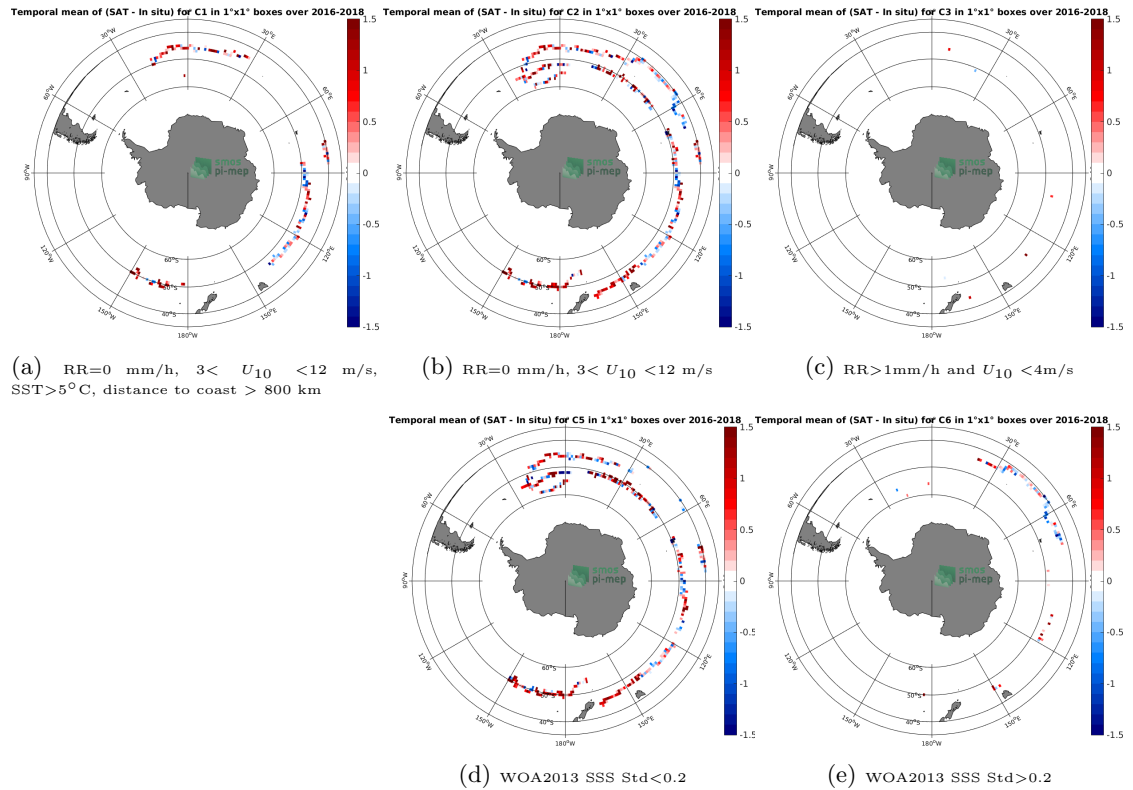
Figure 11: Temporal mean gridded over spatial boxes of size 1^{\circ}\times 1^{\circ} of \Delta\text{SSS} (SMAP-L2-JPL-V4.3 - Surface drifters) for 5 different subdatasets corresponding to:RR=0 mm/h, 3 < U_{10} < 12 m/s, SST >5^{\circ}\text{C} , distance to coast > 800 km (a), RR=0 mm/h, 3 < U_{10} < 12 m/s (b), RR >1 mm/h and U_{10} < 4 m/s (c), WOA2013 SSS Std <0.2 (d), WOA2013 SSS Std >0.2 (e).
