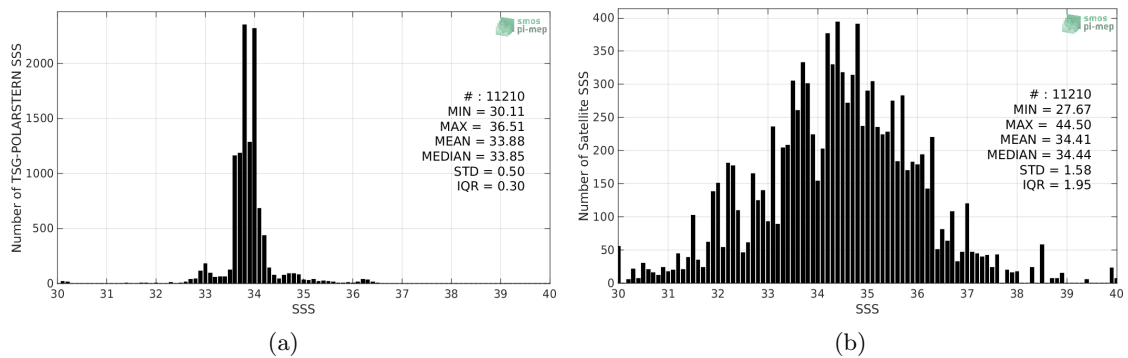
Figure 2: Histograms of SSS from TSG-POLARSTERN (a) and SMAP-L2-JPL-V4.2 (b) considering all match-up pairs per bins of 0.1 over the Roaring Forties and Furious Fifties Pi-MEP region and for the full satellite product period.
