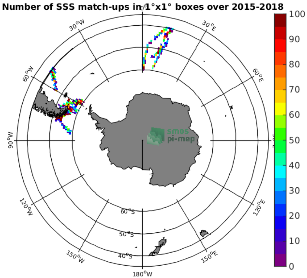
Figure 4: Number of SSS match-ups between TSG-POLARSTERN SSS and the SMAP-L2-JPL-V4.2 SSS product for the Roaring Forties and Furious Fifties Pi-MEP region over 1^\circ \times 1^\circ boxes and for the full satellite product period.
