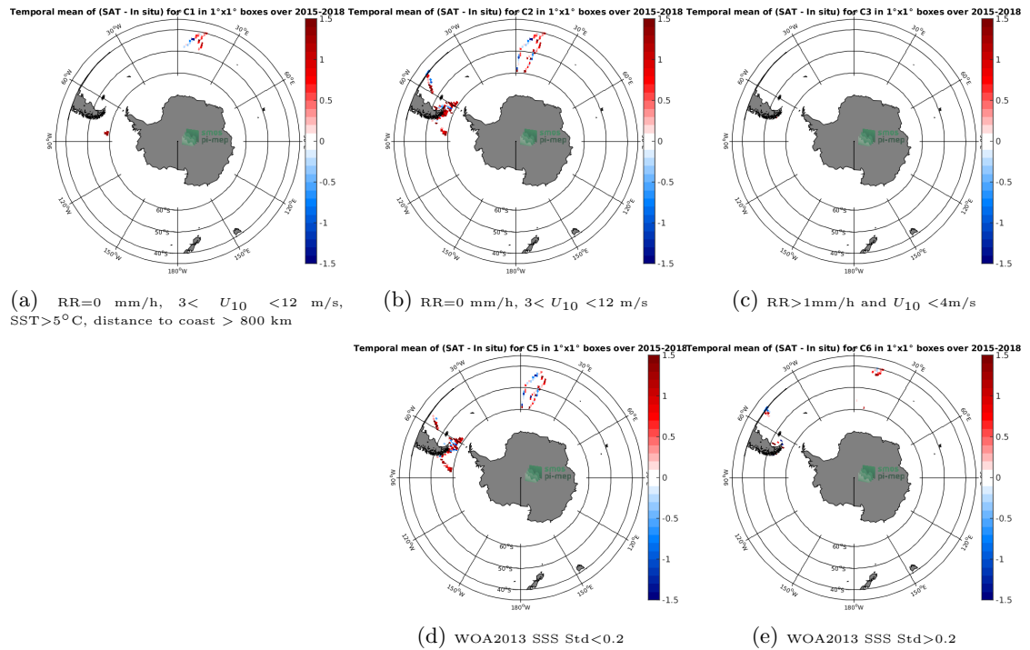
Figure 12: Temporal mean gridded over spatial boxes of size 1^\circ \times 1^\circ of \Delta SSS (SMAP-L2-JPL-V4.2 - TSG-POLARSTERN) for 5 different subdatasets corresponding to: RR=0 mm/h, 3 < U_{10} < 12 m/s, SST > 5^\circ\text{C} , distance to coast > 800 km (a), RR=0 mm/h, 3 < U_{10} < 12 m/s (b), RR > 1 mm/h and U_{10} < 4 m/s (c), WOA2013 SSS Std < 0.2 (d), WOA2013 SSS Std > 0.2 (e).
