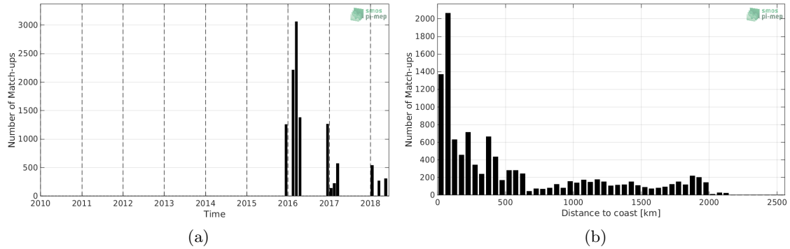
Figure 1: Number of match-ups between TSG-POLARSTERN and SMAP-L2-JPL-V4.2 SSS as a function of time (a) and as function of the distance to coast (b) over the Roaring Forties and Furious Fifties Pi-MEP region and for the full satellite product period.
