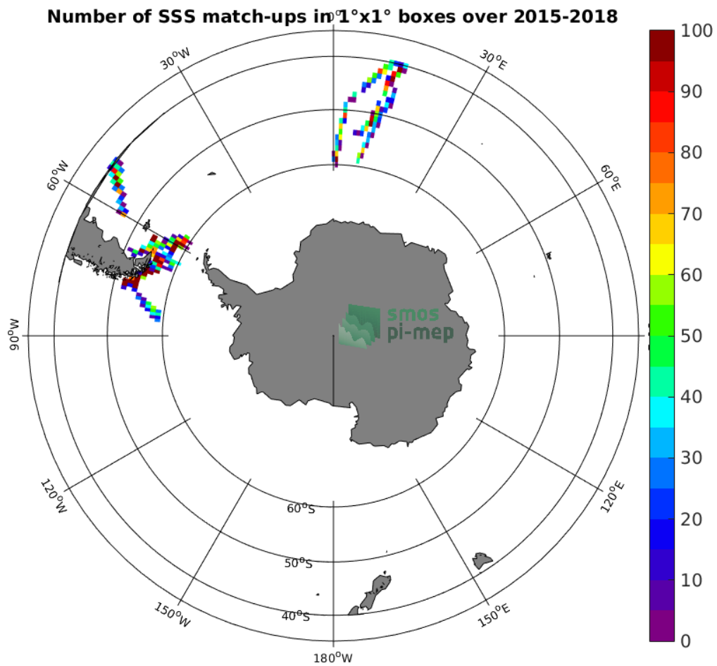
Figure 4: Number of SSS match-ups between TSG-POLARSTERN SSS and the SMAP-L2-JPL-V4.2 SSS product for the Roaring Forties and Furious Fifties Pi-MEP region over 1^\circ \times 1^\circ boxes and for the full satellite product period.
