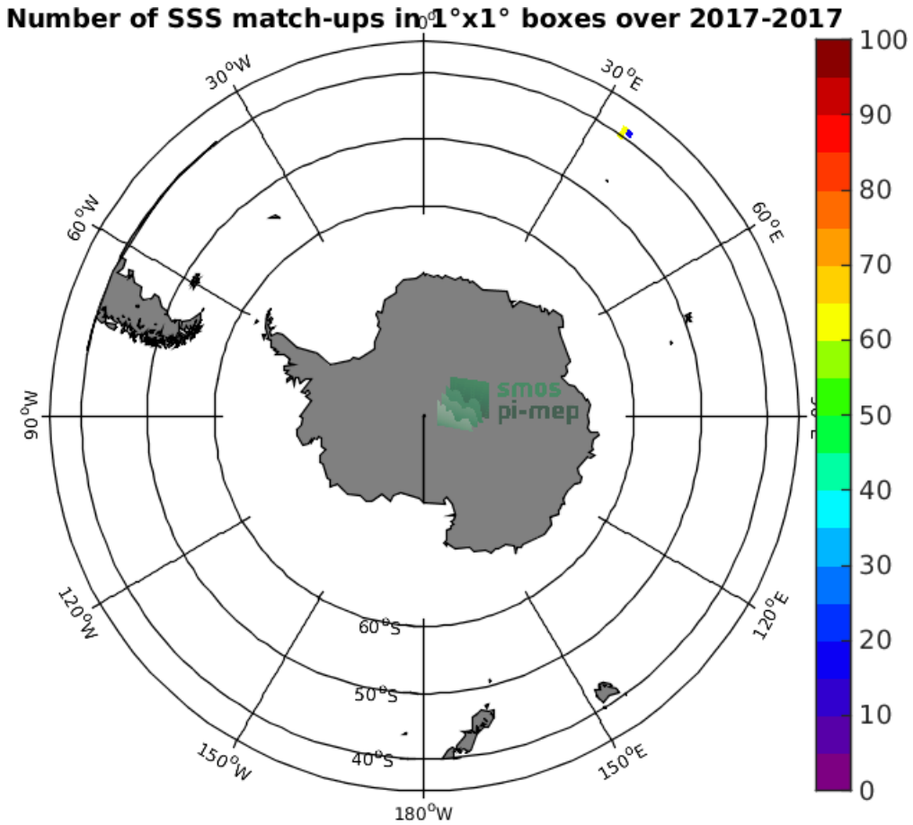
Figure 4: Number of SSS match-ups between TSG-GOSUD-Research-vessel SSS and the SMAP-L2-JPL-V4.2 SSS product for the Roaring Forties and Furious Fifties Pi-MEP region over 1°x1° boxes and for the full satellite product period.
