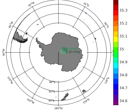
(c) MEAN(TSG-GOSUD-Research-vessel SSS)
