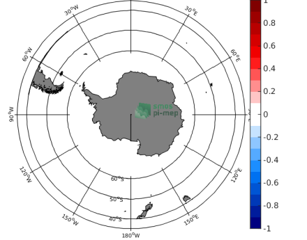
(e) MEAN( \Delta SSS) (Satellite - TSG-GOSUD-Research-vessel)
