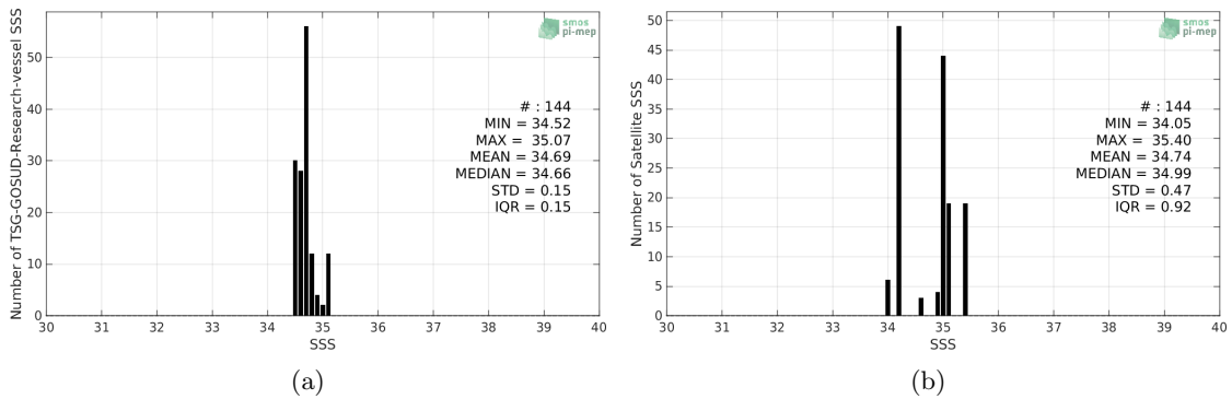
Figure 2: Histograms of SSS from TSG-GOSUD-Research-vessel (a) and SMAP-L2-JPL-V4.2 (b) considering all match-up pairs per bins of 0.1 over the Roaring Forties and Furious Fifties Pi-MEP region and for the full satellite product period.
