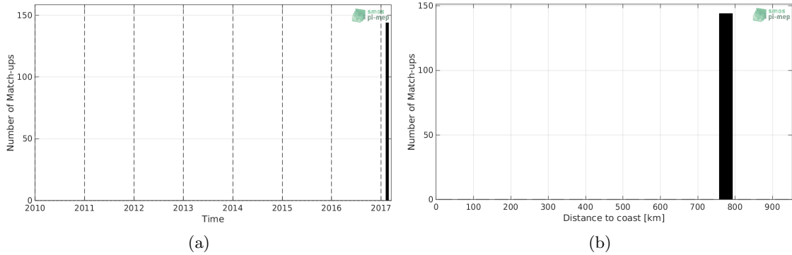
Figure 1: Number of match-ups between TSG-GOSUD-Research-vessel and SMAP-L2-JPL-V4.2 SSS as a function of time (a) and as function of the distance to coast (b) over the Roaring Forties and Furious Fifties Pi-MEP region and for the full satellite product period.
