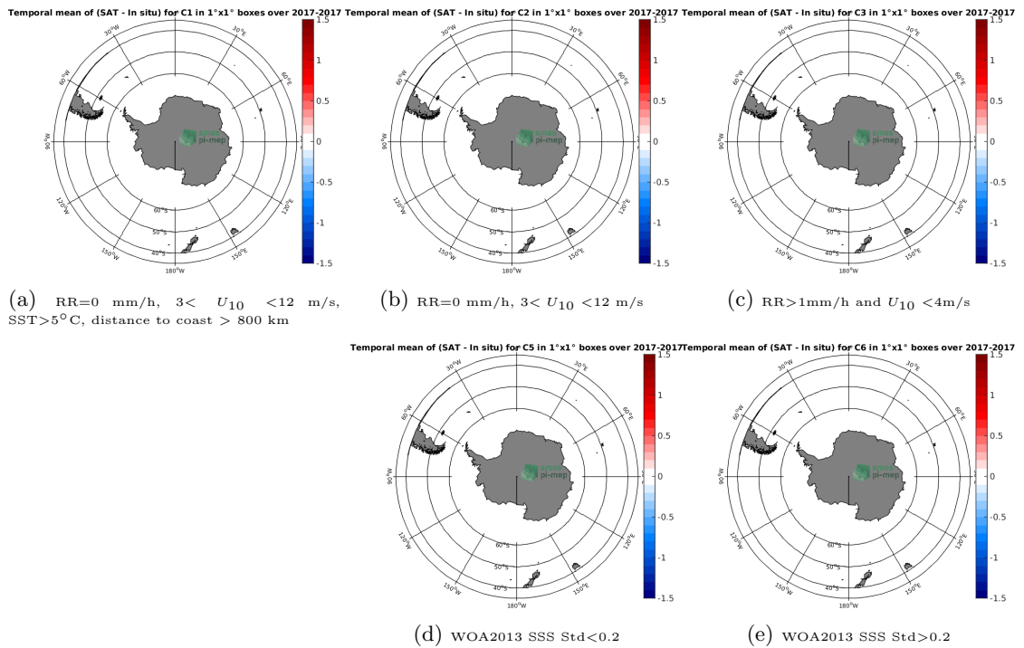
Figure 12: Temporal mean gridded over spatial boxes of size 1^\circ \times 1^\circ of \Delta SSS (SMAP-L2-JPL-V4.2 - TSG-GOSUD-Research-vessel) for 5 different subdatasets corresponding to:RR=0 mm/h, 3 < U_{10} < 12 m/s, SST > 5°C, distance to coast > 800 km (a), RR=0 mm/h, 3 < U_{10} < 12 m/s (b), RR > 1mm/h and U_{10} < 4 m/s (c), WOA2013 SSS Std < 0.2 (d), WOA2013 SSS Std > 0.2 (e).
