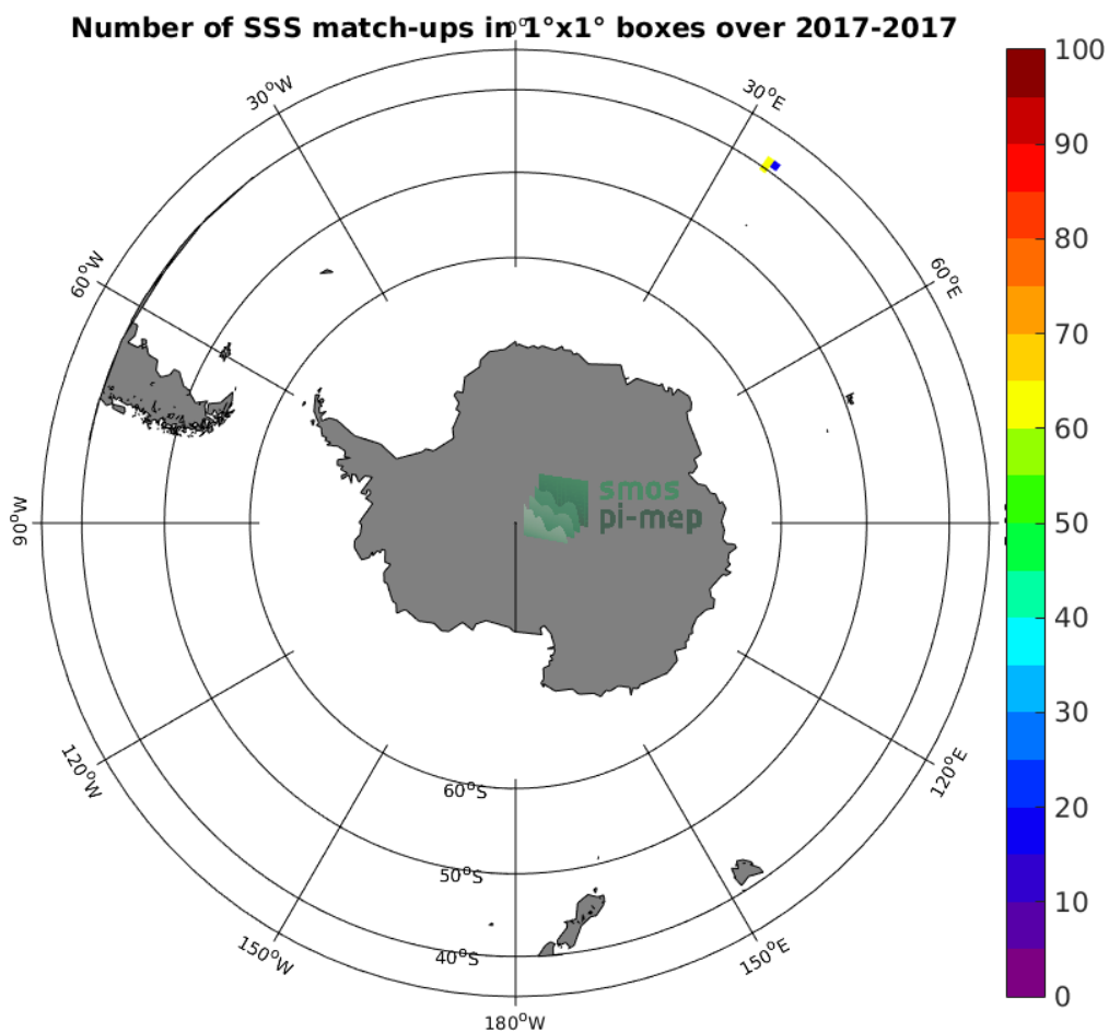
Figure 4: Number of SSS match-ups between TSG-GOSUD-Research-vessel SSS and the SMAP-L2-JPL-V4.2 SSS product for the Roaring Forties and Furious Fifties Pi-MEP region over 1°x1° boxes and for the full satellite product period.
