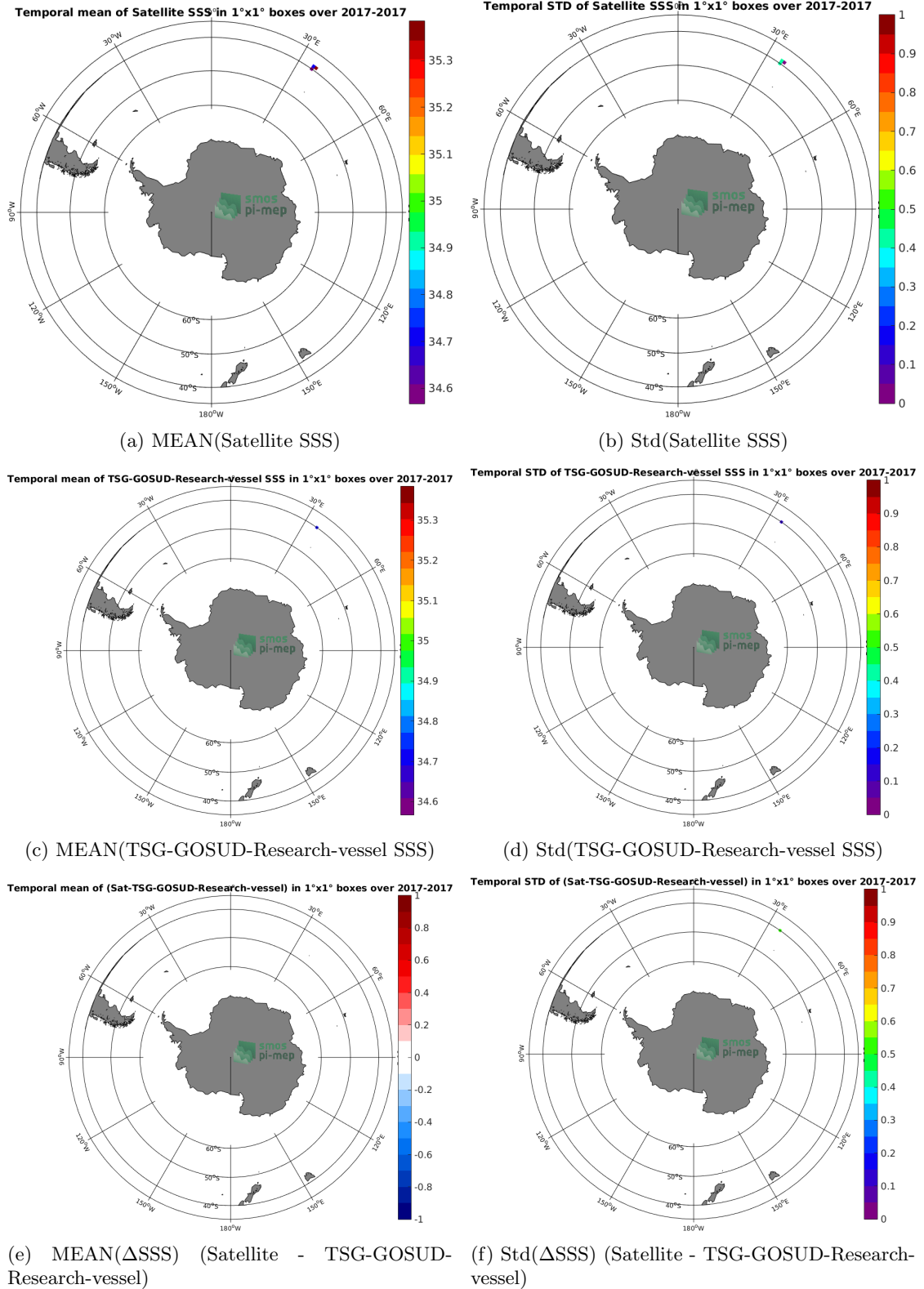
Figure 6: Temporal mean (left) and Std (right) of SSS from SMAP-L2-JPL-V4.2 (top), TSG-GOSUD-Research-vessel (middle), and of \Delta SSS (Satellite - TSG-GOSUD-Research-vessel). Only match-up pairs are used to generate these maps.
