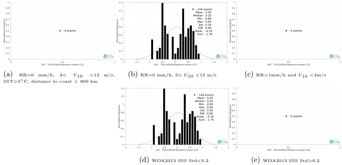
Figure 13: Normalized histogram of \Delta SSS (SMAP-L2-JPL-V4.2 - TSG-GOSUD-Research-vessel) for 5 different subdatasets corresponding to: RR=0 mm/h, 3 < U_{10} < 12 m/s, SST > 5^\circ C , distance to coast > 800 km (a), RR=0 mm/h, 3 < U_{10} < 12 m/s (b), RR > 1 mm/h and U_{10} < 4 m/s (c), WOA2013 SSS Std < 0.2 (d), WOA2013 SSS Std > 0.2 (e).
