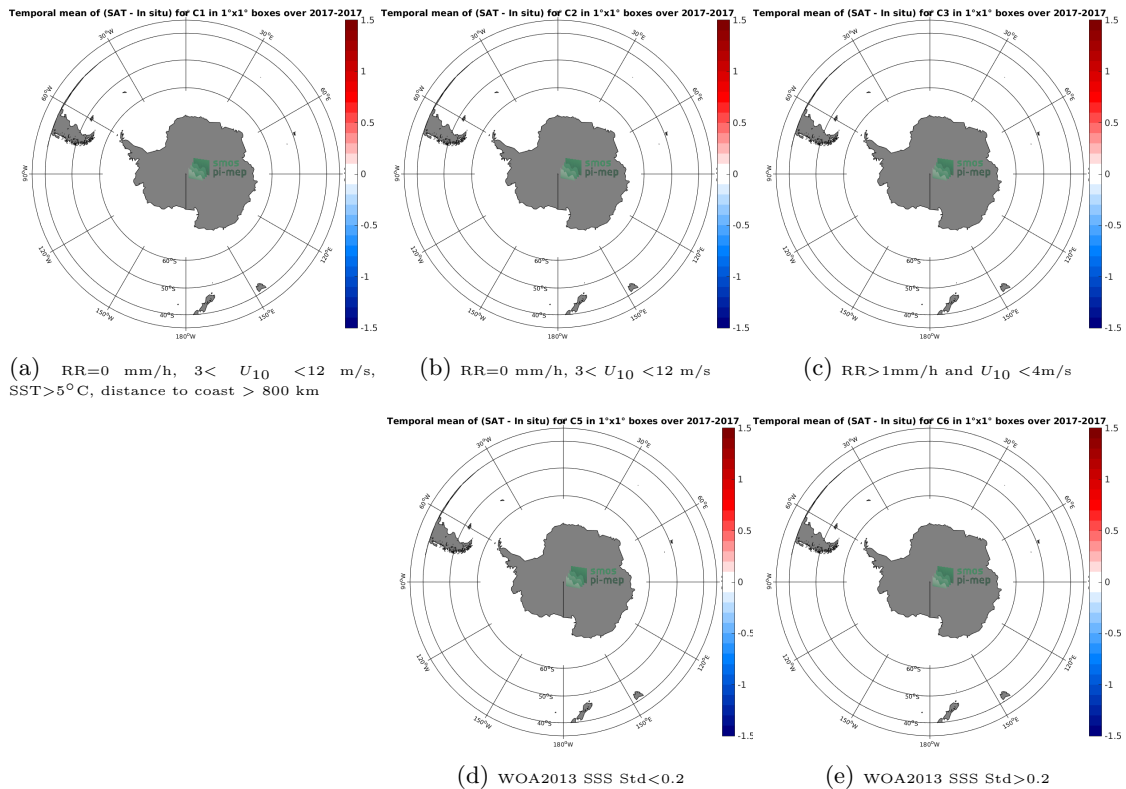
Figure 12: Temporal mean gridded over spatial boxes of size 1^\circ \times 1^\circ of \Delta SSS (SMAP-L2-JPL-V4.2 - TSG-GOSUD-Research-vessel) for 5 different subdatasets corresponding to:RR=0 mm/h, 3 < U_{10} < 12 m/s, SST >5^\circ C, distance to coast > 800 km (a), RR=0 mm/h, 3 < U_{10} < 12 m/s (b), RR >1 mm/h and U_{10} < 4 m/s (c), WOA2013 SSS Std <0.2 (d), WOA2013 SSS Std >0.2 (e).
