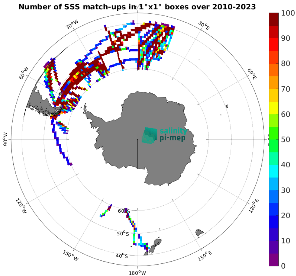
Figure 5: Number of SSS match-ups between TSG (Polarstern) SSS and the ISAS v7 - Monthly (Ifremer-LOPS-CMEMS) SSS product for the Roaring Forties and Furious Fifties Pi-MEP region over 1^{\circ} \times 1^{\circ} boxes and for the full satellite product period.
