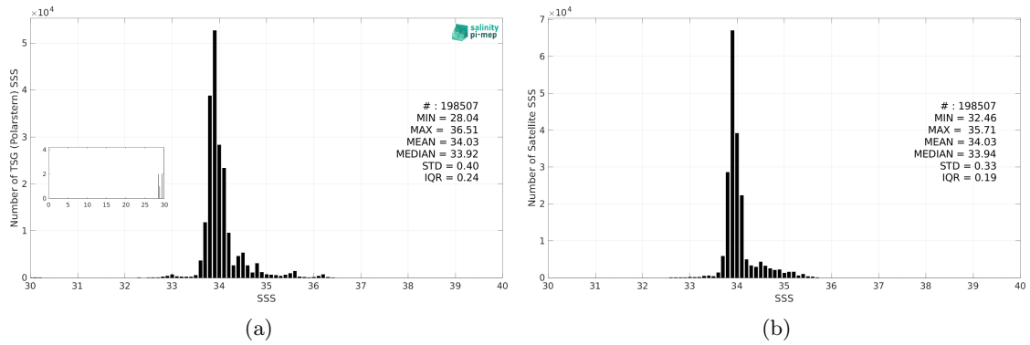
Figure 3: Histograms of SSS from TSG (Polarstern) (a) and ISAS v7 - Monthly (Ifremer-LOPS-CMEMS) (b) considering all match-up pairs per bins of 0.1 over the Roaring Forties and Furious Fifties Pi-MEP region and for the full satellite product period.
