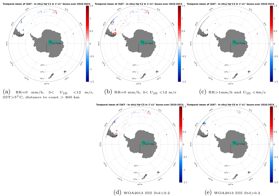
Figure 14: Temporal mean gridded over spatial boxes of size 1^\circ \times 1^\circ of \Delta SSS (ISAS v7 - Monthly (Ifremer-LOPS-CMEMS) - TSG (Polarstern)) for 5 different subdatasets corresponding to: RR=0 mm/h, 3 < U_{10} < 12 m/s, SST > 5^\circ\text{C} , distance to coast > 800 km (a), RR=0 mm/h, 3 < U_{10} < 12 m/s (b), RR > 1 mm/h and U_{10} < 4 m/s (c), WOA2013 SSS Std < 0.2 (d), WOA2013 SSS Std > 0.2 (e).
