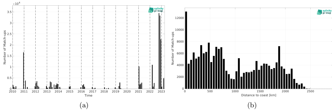
Figure 2: Number of match-ups between TSG (Polarstern) and ISAS v7 - Monthly (Ifremer-LOPS-CMEMS) SSS as a function of time (a) and as function of the distance to coast (b) over the Roaring Forties and Furious Fifties Pi-MEP region and for the full satellite product period.
