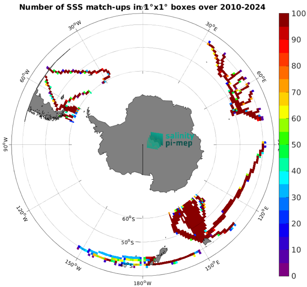
Figure 5: Number of SSS match-ups between TSG (LEGOS-DM) SSS and the ISAS v7 - Monthly (Ifremer-LOPS-CMEMS) SSS product for the Roaring Forties and Furious Fifties Pi-MEP region over 1^\circ \times 1^\circ boxes and for the full satellite product period.
