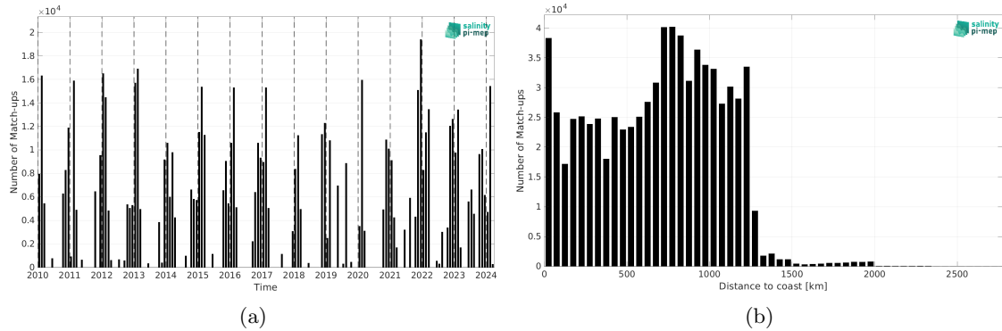
Figure 2: Number of match-ups between TSG (LEGOS-DM) and ISAS v7 - Monthly (Ifremer-LOPS-CMEMS) SSS as a function of time (a) and as function of the distance to coast (b) over the Roaring Forties and Furious Fifties Pi-MEP region and for the full satellite product period.
