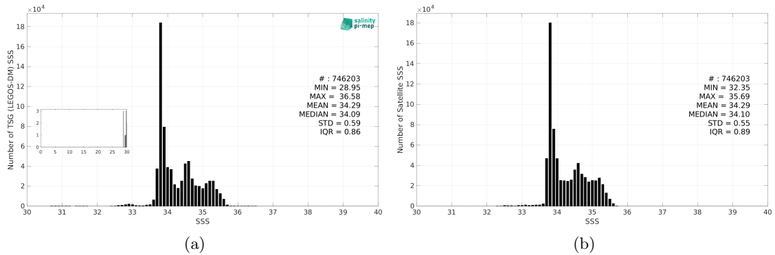
Figure 3: Histograms of SSS from TSG (LEGOS-DM) (a) and ISAS v7 - Monthly (Ifremer-LOPS-CMEMS) (b) considering all match-up pairs per bins of 0.1 over the Roaring Forties and Furious Fifties Pi-MEP region and for the full satellite product period.
