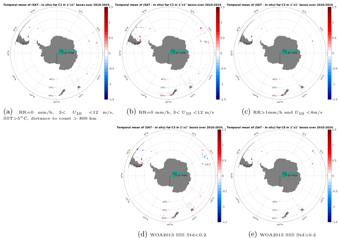
Figure 14: Temporal mean gridded over spatial boxes of size 1^\circ \times 1^\circ of \Delta SSS (ISAS v7 - Monthly (Ifremer-LOPS-CMEMS) - TSG (LEGOS-DM)) for 5 different subdatasets corresponding to: RR=0 mm/h, 3 < U_{10} < 12 m/s, SST > 5^\circ\text{C} , distance to coast > 800 km (a), RR=0 mm/h, 3 < U_{10} < 12 m/s (b), RR > 1 mm/h and U_{10} < 4 m/s (c), WOA2013 SSS Std < 0.2 (d), WOA2013 SSS Std > 0.2 (e).
