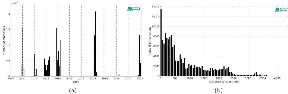
Figure 2: Number of match-ups between TSG (GOSUD-Sailing-ship) and ISAS v7 - Monthly (Ifremer-LOPS-CMEMS) SSS as a function of time (a) and as function of the distance to coast (b) over the Roaring Forties and Furious Fifties Pi-MEP region and for the full satellite product period.
