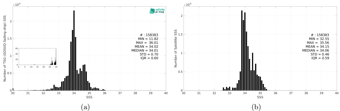
Figure 3: Histograms of SSS from TSG (GOSUD-Sailing-ship) (a) and ISAS v7 - Monthly (Ifremer-LOPS-CMEMS) (b) considering all match-up pairs per bins of 0.1 over the Roaring Forties and Furious Fifties Pi-MEP region and for the full satellite product period.
