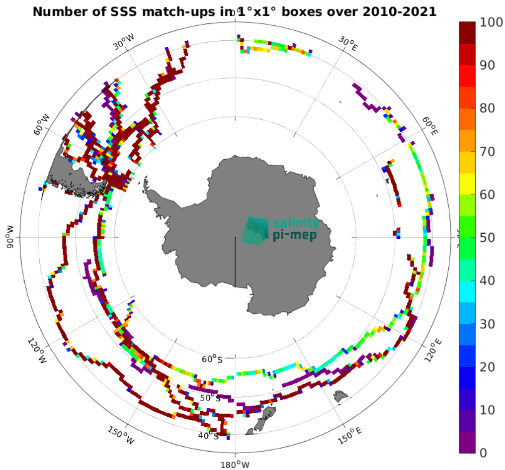
Figure 5: Number of SSS match-ups between TSG (GOSUD-Sailing-ship) SSS and the ISAS v7 - Monthly (Ifremer-LOPS-CMEMS) SSS product for the Roaring Forties and Furious Fifties Pi-MEP region over 1^\circ \times 1^\circ boxes and for the full satellite product period.
