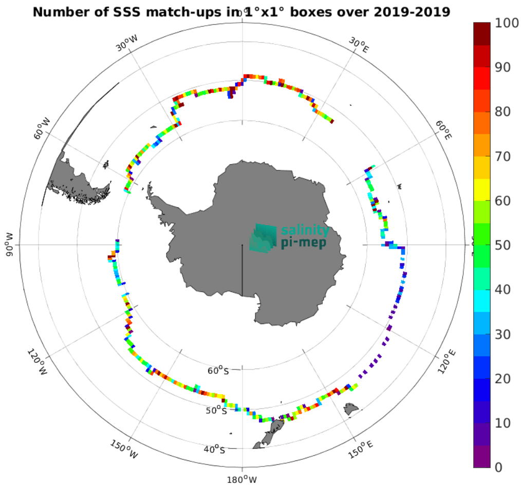
Figure 5: Number of SSS match-ups between Saildrone SSS and the ISAS v7 - Monthly (Ifremer-LOPS-CMEMS) SSS product for the Roaring Forties and Furious Fifties Pi-MEP region over 1^{\circ} \times 1^{\circ} boxes and for the full satellite product period.
