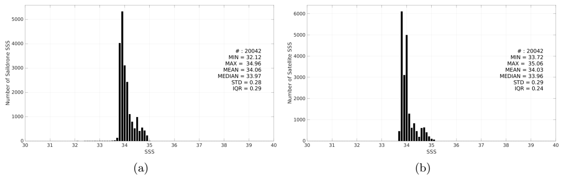
Figure 3: Histograms of SSS from Saildrone (a) and ISAS v7 - Monthly (Ifremer-LOPS-CMEMS) (b) considering all match-up pairs per bins of 0.1 over the Roaring Forties and Furious Fifties Pi-MEP region and for the full satellite product period.
