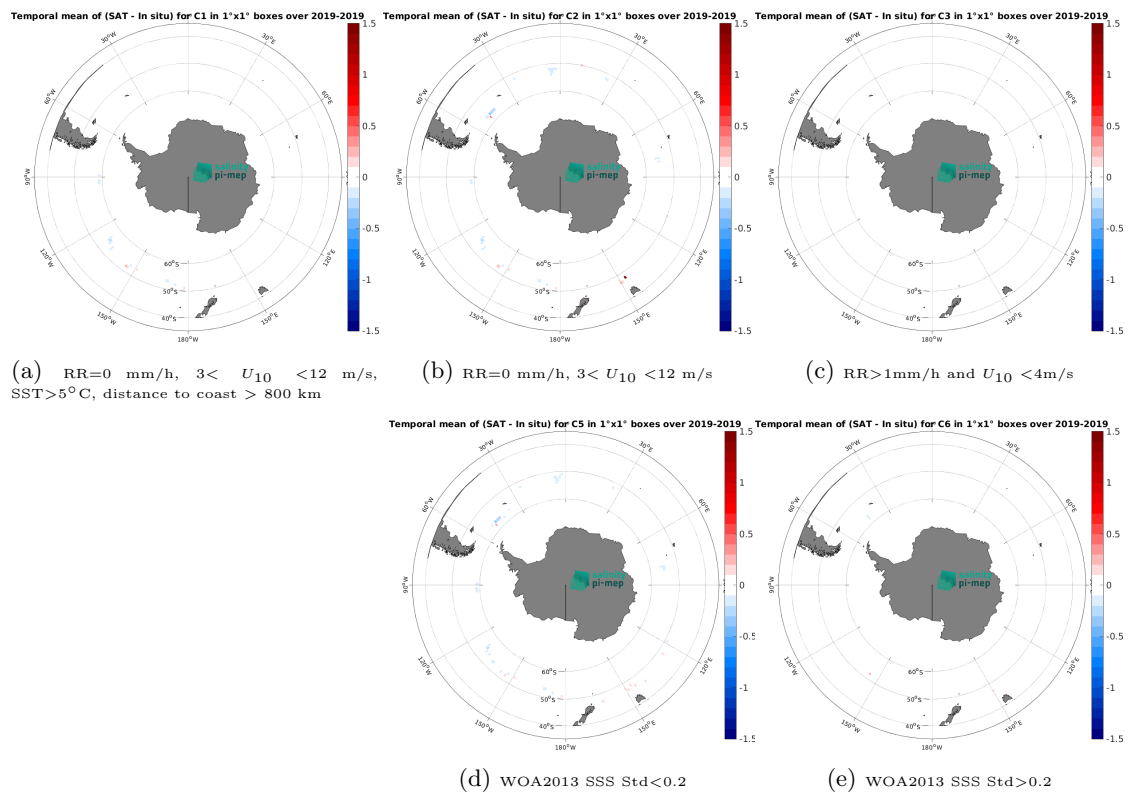
Figure 14: Temporal mean gridded over spatial boxes of size 1^\circ \times 1^\circ of \Delta SSS (ISAS v7 - Monthly (Ifremer-LOPS-CMEMS) - Saifdrone) for 5 different subdatasets corresponding to:RR=0 mm/h, 3 < U_{10} < 12 m/s, SST >5^\circ C, distance to coast > 800 km (a), RR=0 mm/h, 3 < U_{10} < 12 m/s (b), RR >1 mm/h and U_{10} < 4 m/s (c), WOA2013 SSS Std <0.2 (d), WOA2013 SSS Std >0.2 (e).
