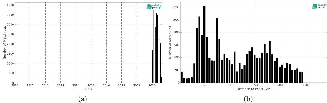
Figure 2: Number of match-ups between Saildrone and ISAS v7 - Monthly (Ifremer-LOPS-CMEMS) SSS as a function of time (a) and as function of the distance to coast (b) over the Roaring Forties and Furious Fifties Pi-MEP region and for the full satellite product period.
