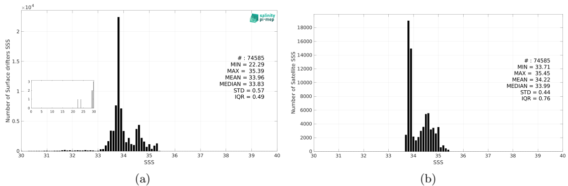
Figure 3: Histograms of SSS from Surface drifters (a) and ISAS v7 - Monthly (Ifremer-LOPS-CMEMS) (b) considering all match-up pairs per bins of 0.1 over the Roaring Forties and Furious Fifties Pi-MEP region and for the full satellite product period.
