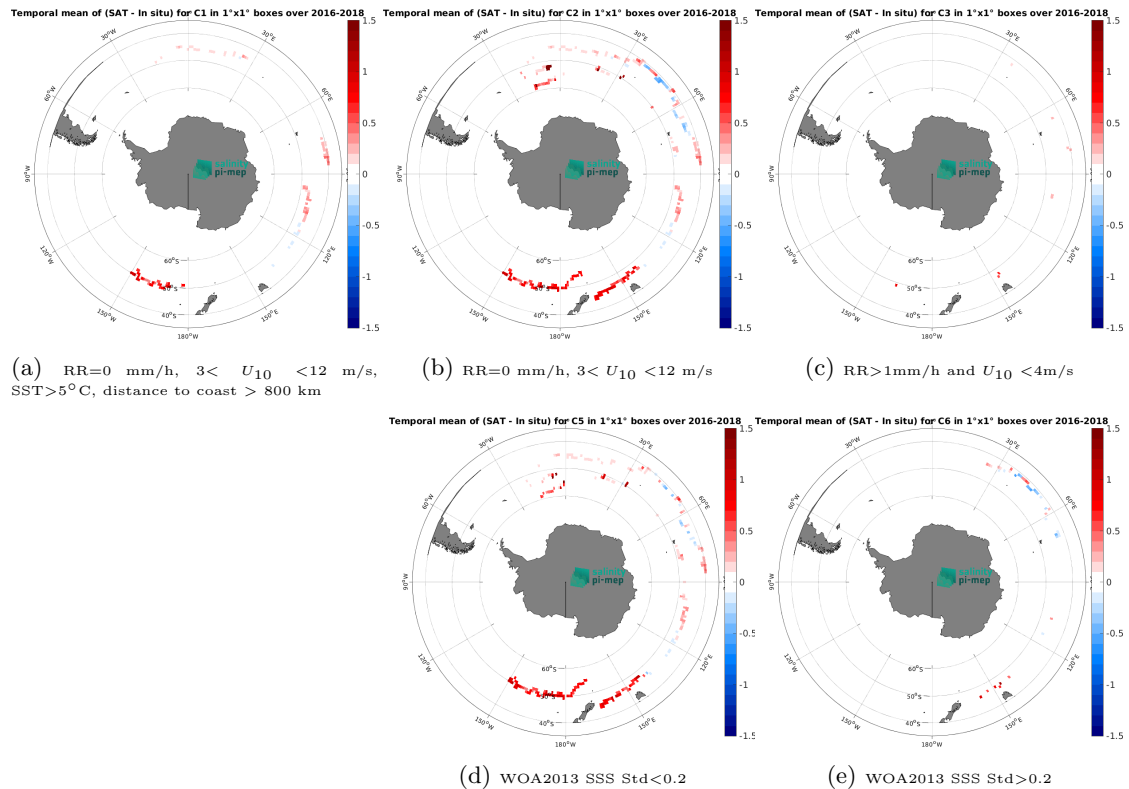
Figure 13: Temporal mean gridded over spatial boxes of size 1^\circ \times 1^\circ of \Delta SSS (ISAS v7 - Monthly (Ifremer-LOPS-CMEMS) - Surface drifters) for 5 different subdatasets corresponding to:RR=0 mm/h, 3 < U_{10} < 12 m/s, SST >5^\circ\text{C} , distance to coast > 800 km (a), RR=0 mm/h, 3 < U_{10} < 12 m/s (b), RR >1 mm/h and U_{10} < 4 m/s (c), WOA2013 SSS Std <0.2 (d), WOA2013 SSS Std >0.2 (e).
