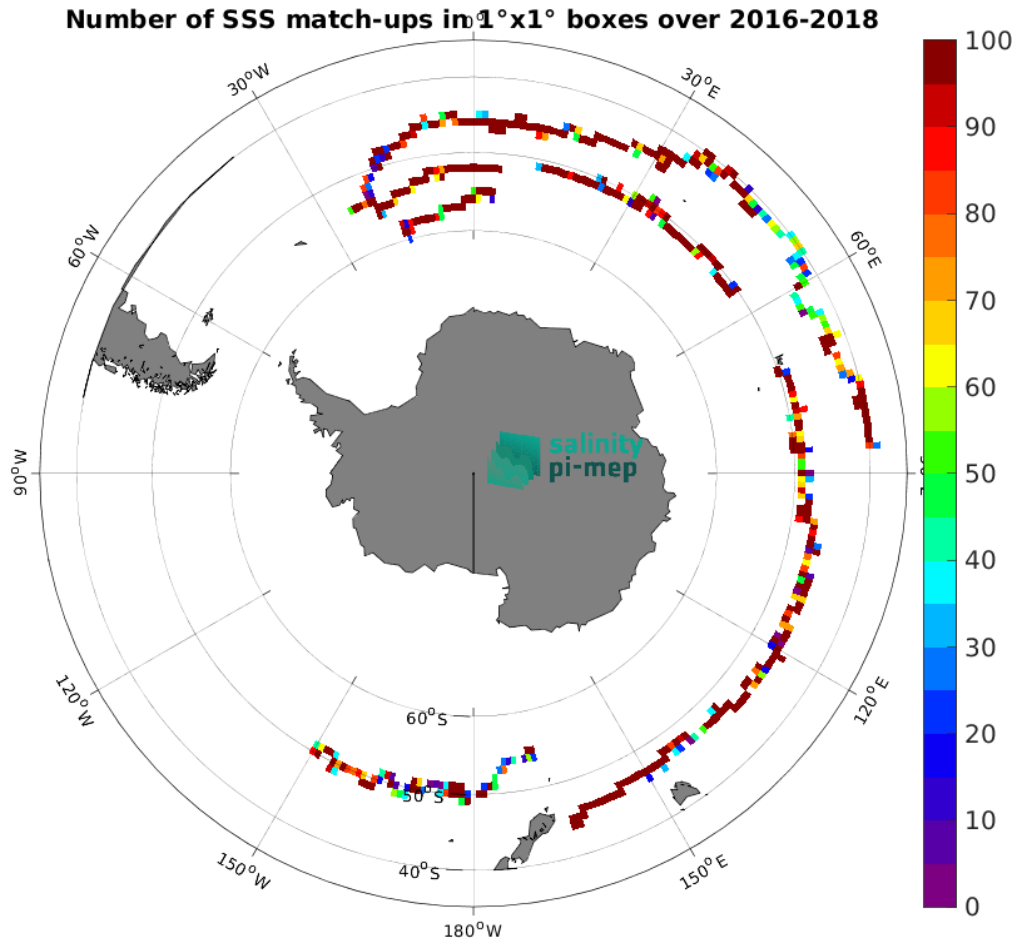
Figure 4: Number of SSS match-ups between Surface drifters SSS and the ISAS v7 - Monthly (Ifremer-LOPS-CMEMS) SSS product for the Roaring Forties and Furious Fifties Pi-MEP region over 1^\circ \times 1^\circ boxes and for the full satellite product period.
