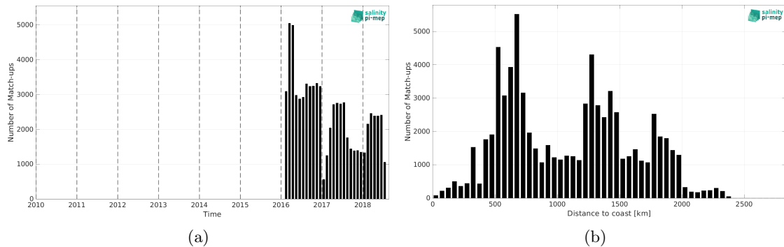
Figure 2: Number of match-ups between Surface drifters and ISAS v7 - Monthly (Ifremer-LOPS-CMEMS) SSS as a function of time (a) and as function of the distance to coast (b) over the Roaring Forties and Furious Fifties Pi-MEP region and for the full satellite product period.
