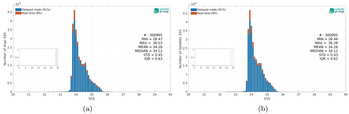
Figure 3: Histograms of SSS from Argo (a) and ISAS v7 - Monthly (Ifremer-LOPS-CMEMS) (b) considering all match-up pairs per bins of 0.1 over the Roaring Forties and Furious Fifties Pi-MEP region and for the full satellite product period.
