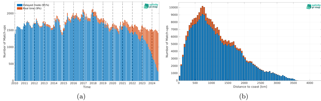
Figure 2: Number of match-ups between Argo and ISAS v7 - Monthly (Ifremer-LOPS-CMEMS) SSS as a function of time (a) and as function of the distance to coast (b) over the Roaring Forties and Furious Fifties Pi-MEP region and for the full satellite product period.
