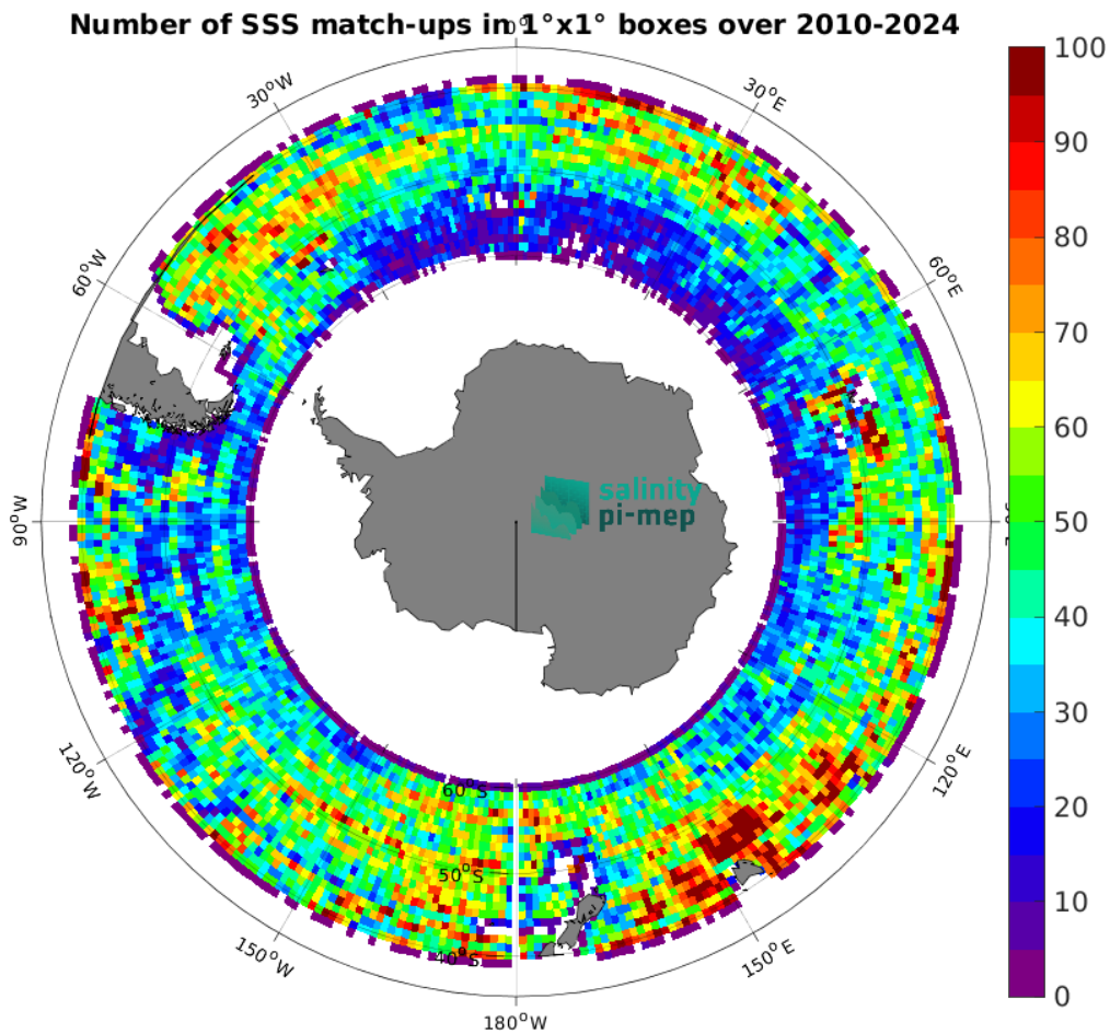
Figure 5: Number of SSS match-ups between Argo SSS and the ISAS v7 - Monthly (Ifremer-LOPS-CMEMS) SSS product for the Roaring Forties and Furious Fifties Pi-MEP region over 1^\circ \times 1^\circ boxes and for the full satellite product period.
