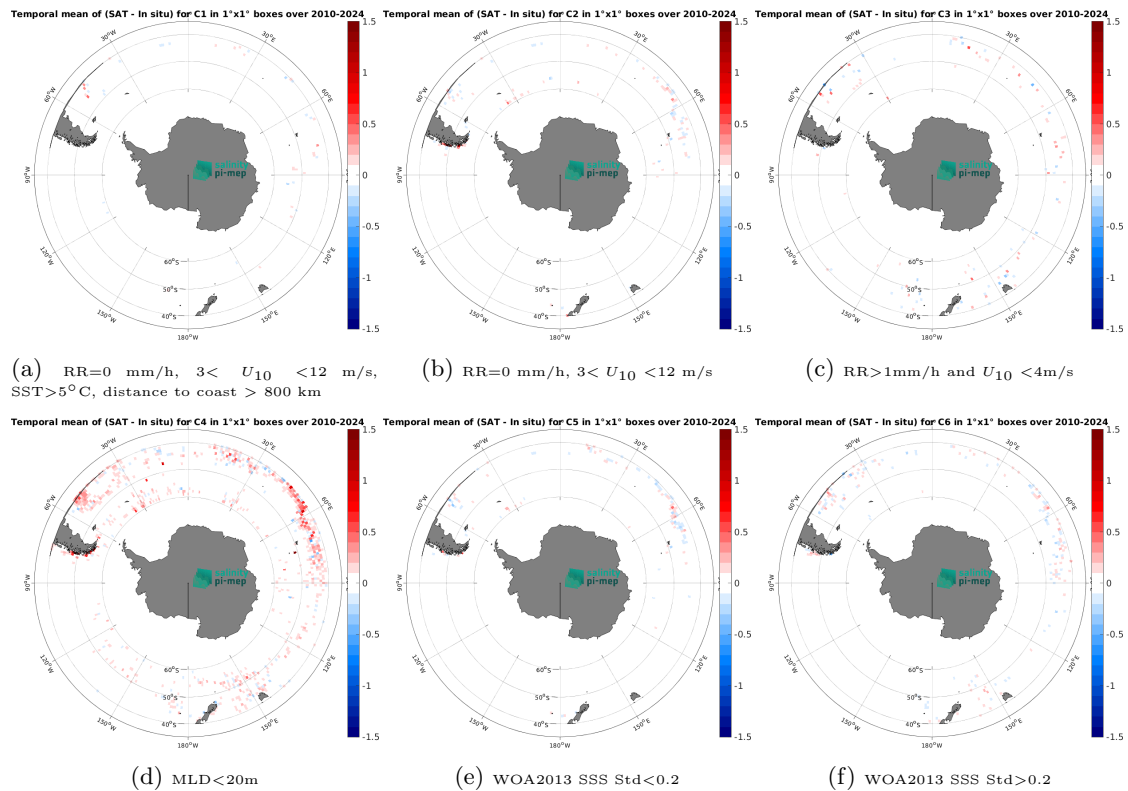
Figure 14: Temporal mean gridded over spatial boxes of size 1^\circ \times 1^\circ of \Delta SSS (ISAS v7 - Monthly (Ifremer-LOPS-CMEMS) - Argo) for 6 different subdatasets corresponding to:RR=0 mm/h, 3 < U_{10} < 12 m/s, SST>5°C, distance to coast > 800 km (a), RR=0 mm/h, 3 < U_{10} < 12 m/s (b), RR>1mm/h and U_{10} < 4 m/s (c),MLD<20m (d),WOA2013 SSS Std<0.2 (e),WOA2013 SSS Std>0.2 (f).
