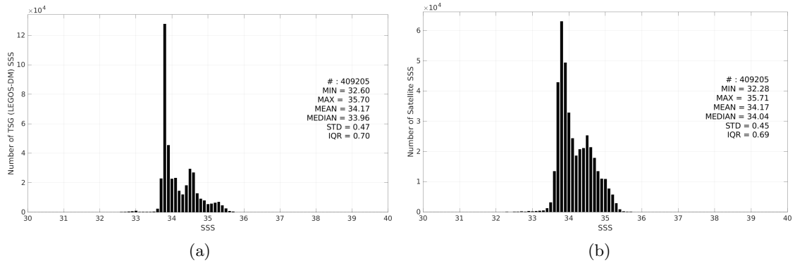
Figure 3: Histograms of SSS from TSG (LEGOS-DM) (a) and CCI SSS L4 POLAR SH Merged-OI v4.41 - 7-day running (ESA) (b) considering all match-up pairs per bins of 0.1 over the Roaring Forties and Furious Fifties Pi-MEP region and for the full satellite product period.
