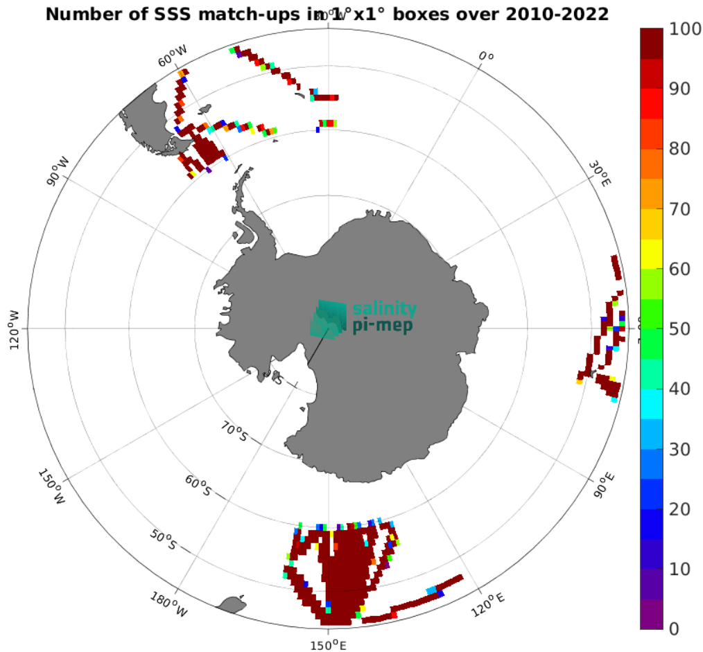
Figure 5: Number of SSS match-ups between TSG (LEGOS-DM) SSS and the CCI SSS L4 POLAR SH Merged-OI v4.41 - 7-day running (ESA) SSS product for the Roaring Forties and Furious Fifties Pi-MEP region over 1^\circ \times 1^\circ boxes and for the full satellite product period.
