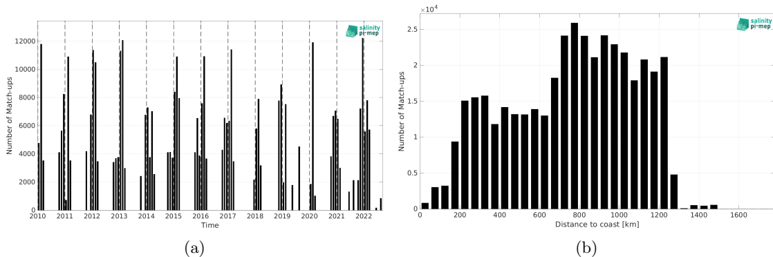
Figure 2: Number of match-ups between TSG (LEGOS-DM) and CCI SSS L4 POLAR SH Merged-OI v4.41 - 7-day running (ESA) SSS as a function of time (a) and as function of the distance to coast (b) over the Roaring Forties and Furious Fifties Pi-MEP region and for the full satellite product period.
