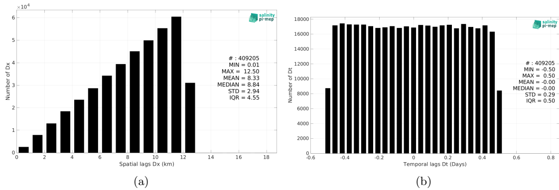
Figure 6: Histograms of the spatial (a) and temporal (b) lags between the location/time of the TSG (LEGOS-DM) measurement and the date of the corresponding CCI SSS L4 POLAR SH Merged-OI v4.41 - 7-day running (ESA) SSS pixel.
