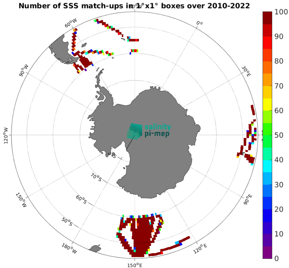
Figure 5: Number of SSS match-ups between TSG (LEGOS-DM) SSS and the CCI SSS L4 POLAR SH Merged-OI v4.41 - 7-day running (ESA) SSS product for the Roaring Forties and Furious Fifties Pi-MEP region over 1^\circ \times 1^\circ boxes and for the full satellite product period.
