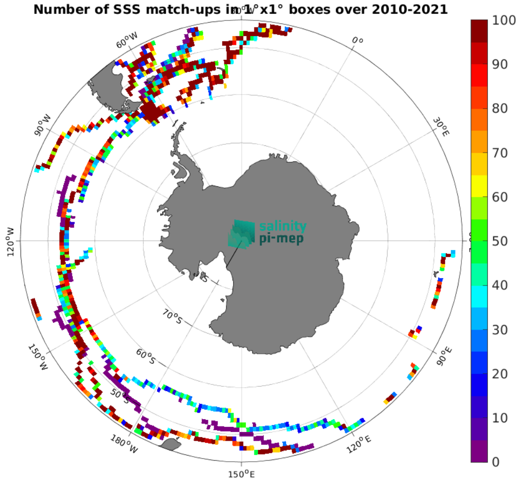
Figure 5: Number of SSS match-ups between TSG (GOSUD-Sailing-ship) SSS and the CCI SSS L4 POLAR SH Merged-OI v4.41 - 7-day running (ESA) SSS product for the Roaring Forties and Furious Fifties Pi-MEP region over 1^\circ \times 1^\circ boxes and for the full satellite product period.
