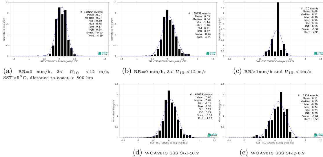
Figure 15: Normalized histogram of \Delta SSS (CCI SSS L4 POLAR SH Merged-OI v4.41 - 7-day running (ESA) - TSG (GOSUD-Sailing-ship)) for 5 different subdatasets corresponding to: RR=0 mm/h, 3 < U_{10} < 12 m/s, SST>5°C, distance to coast > 800 km (a), RR=0 mm/h, 3 < U_{10} < 12 m/s (b), RR>1mm/h and U_{10} < 4 m/s (c), WOA2013 SSS Std<0.2 (d), WOA2013 SSS Std>0.2 (e).
