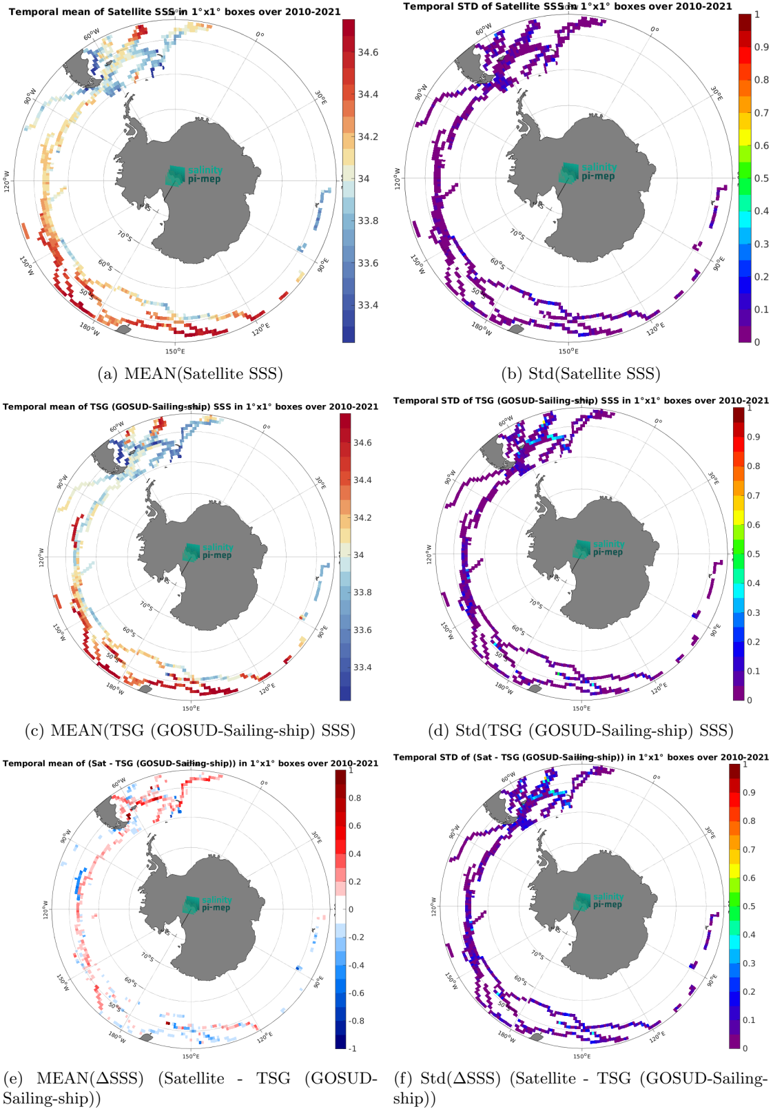
Figure 7: Temporal mean (left) and Std (right) of SSS from CCI SSS L4 POLAR SH Merged-OI v4.41 - 7-day running (ESA) (top), TSG (GOSUD-Sailing-ship) (middle), and of \Delta SSS (Satellite - TSG (GOSUD-Sailing-ship)). Only match-up pairs are used to generate these maps.
