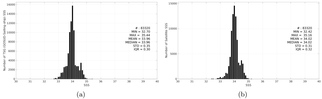
Figure 3: Histograms of SSS from TSG (GOSUD-Sailing-ship) (a) and CCI SSS L4 POLAR SH Merged-OI v4.41 - 7-day running (ESA) (b) considering all match-up pairs per bins of 0.1 over the Roaring Forties and Furious Fifties Pi-MEP region and for the full satellite product period.
