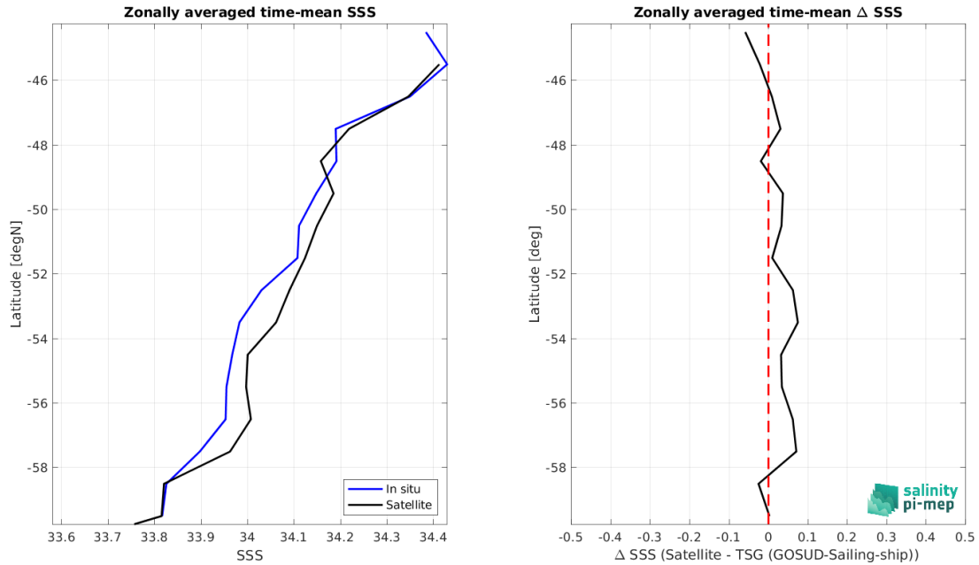
Figure 9: Left panel: Zonal mean SSS from CCI SSS L4 POLAR SH Merged-OI v4.41 - 7-day running (ESA) satellite product (black) and from TSG (GOSUD-Sailing-ship) (blue). Right panel: Zonal mean of \Delta SSS (Satellite - TSG (GOSUD-Sailing-ship)) for all the collected Pi-MEP match-up pairs estimated over the full satellite product period.
