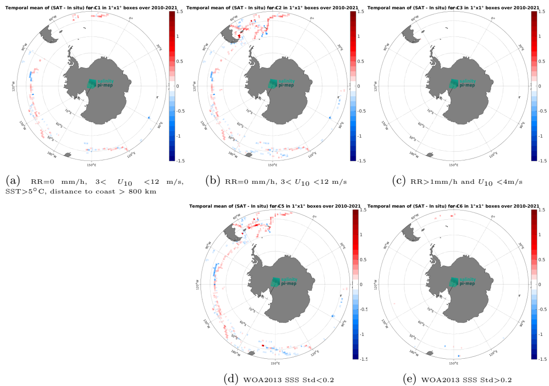
Figure 14: Temporal mean gridded over spatial boxes of size 1^\circ \times 1^\circ of \Delta SSS (CCI SSS L4 POLAR SH Merged-OI v4.41 - 7-day running (ESA) - TSG (GOSUD-Sailing-ship)) for 5 different subdatasets corresponding to:RR=0 mm/h, 3 < U_{10} < 12 m/s, SST >5^\circ C, distance to coast > 800 km (a), RR=0 mm/h, 3 < U_{10} < 12 m/s (b), RR >1 mm/h and U_{10} < 4 m/s (c), WOA2013 SSS Std <0.2 (d), WOA2013 SSS Std >0.2 (e).
