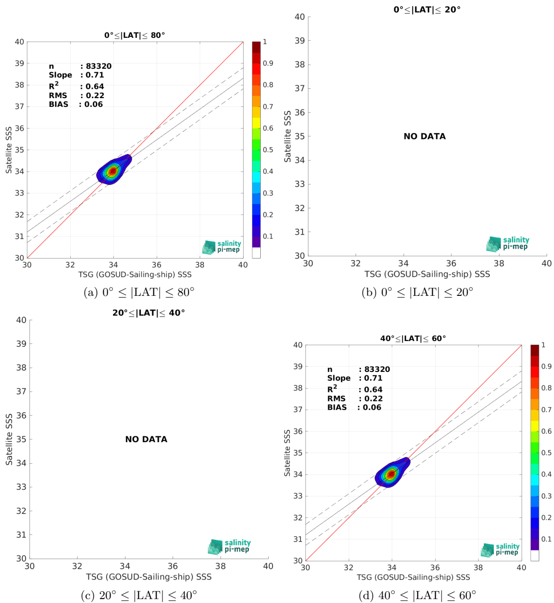
Figure 10: Contour maps of the concentration of CCI SSS L4 POLAR SH Merged-OI v4.41 - 7-day running (ESA) SSS (y-axis) versus TSG (GOSUD-Sailing-ship) SSS (x-axis) at match-up pairs for different latitude bands. For each plot, the red line shows x=y . The black thin and dashed lines indicate a linear fit through the data cloud and the \pm 95\% confidence levels, respectively. The number match-up pairs n , the slope and R^2 coefficient of the linear fit, the root mean square (RMS) and the mean bias between satellite and in situ data are indicated for each latitude band in each plots.
