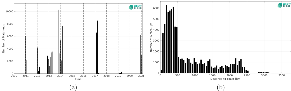
Figure 2: Number of match-ups between TSG (GOSUD-Sailing-ship) and CCI SSS L4 POLAR SH Merged-OI v4.41 - 7-day running (ESA) SSS as a function of time (a) and as function of the distance to coast (b) over the Roaring Forties and Furious Fifties Pi-MEP region and for the full satellite product period.
