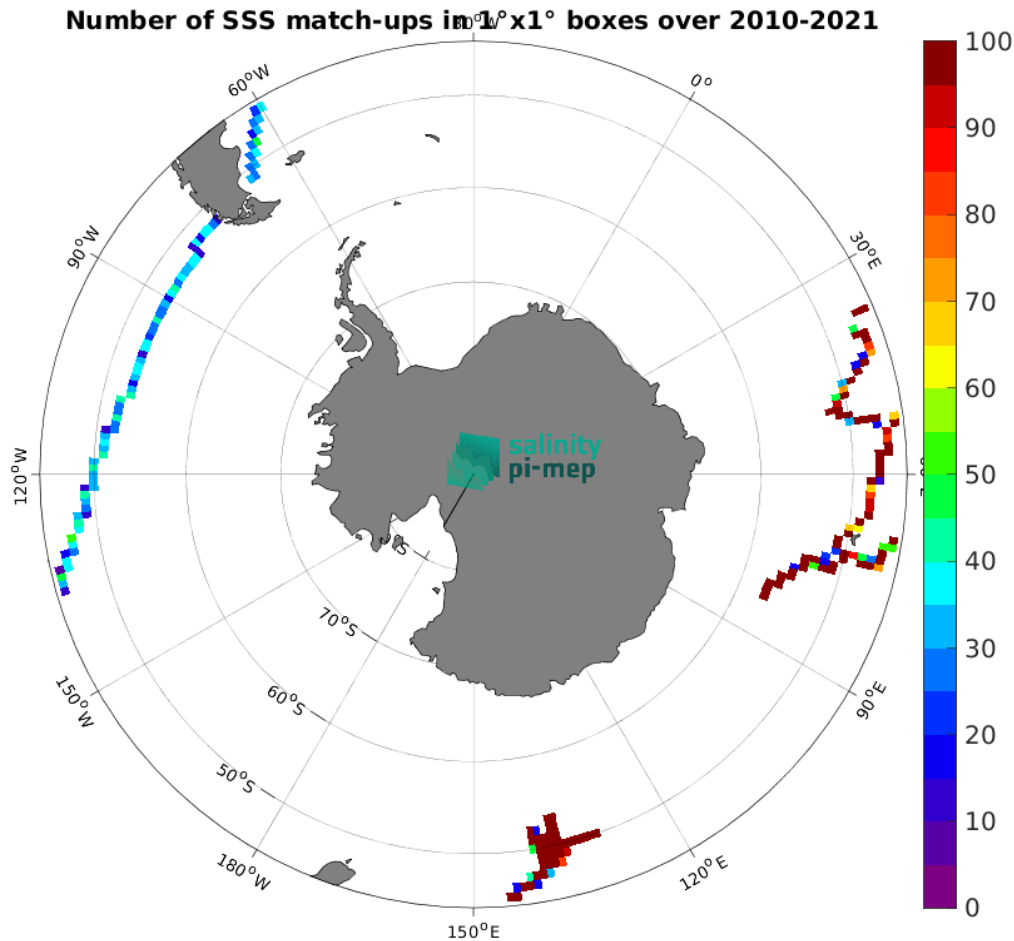
Figure 5: Number of SSS match-ups between TSG (GOSUD-Research-vessel) SSS and the CCI SSS L4 POLAR SH Merged-OI v4.41 - 7-day running (ESA) SSS product for the Roaring Forties and Furious Fifties Pi-MEP region over 1^\circ \times 1^\circ boxes and for the full satellite product period.
