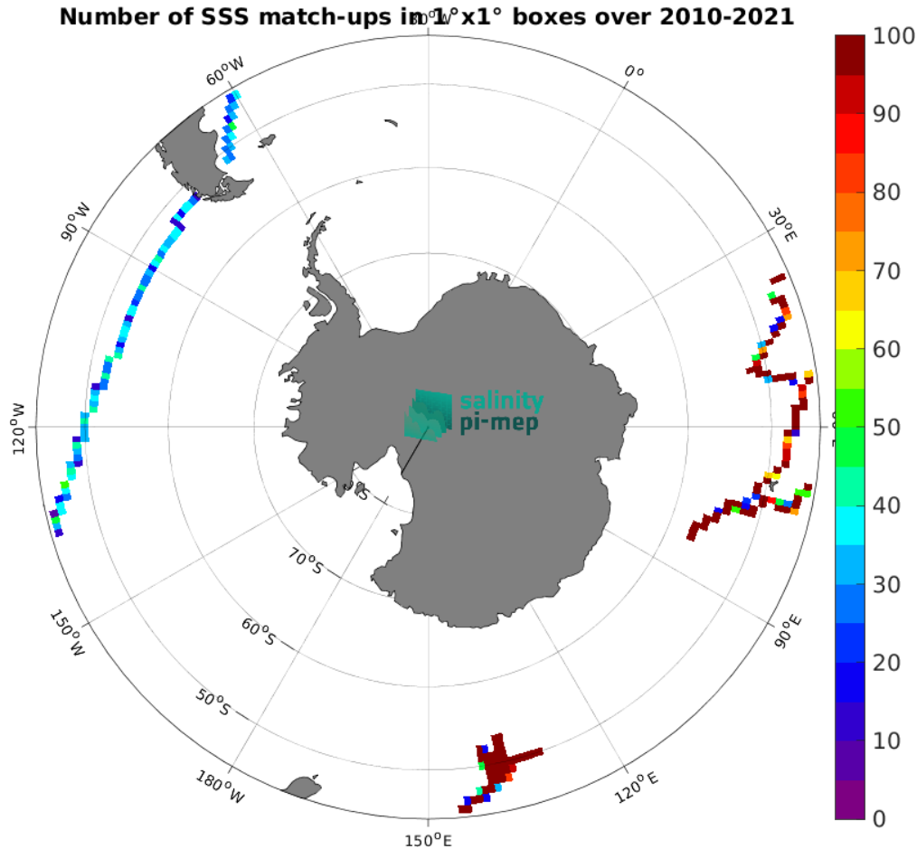
Figure 5: Number of SSS match-ups between TSG (GOSUD-Research-vessel) SSS and the CCI SSS L4 POLAR SH Merged-OI v4.41 - 7-day running (ESA) SSS product for the Roaring Forties and Furious Fifties Pi-MEP region over 1^\circ \times 1^\circ boxes and for the full satellite product period.
