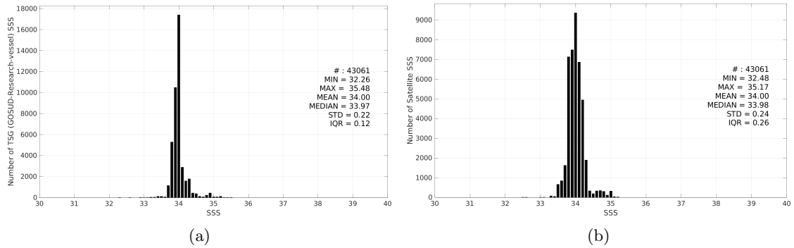
Figure 3: Histograms of SSS from TSG (GOSUD-Research-vessel) (a) and CCI SSS L4 POLAR SH Merged-OI v4.41 - 7-day running (ESA) (b) considering all match-up pairs per bins of 0.1 over the Roaring Forties and Furious Fifties Pi-MEP region and for the full satellite product period.
