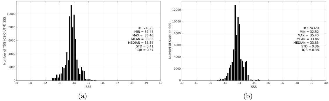
Figure 3: Histograms of SSS from TSG (CSIC-UTM) (a) and CCI SSS L4 POLAR SH Merged-OI v4.41 - 7-day running (ESA) (b) considering all match-up pairs per bins of 0.1 over the Roaring Forties and Furious Fifties Pi-MEP region and for the full satellite product period.
