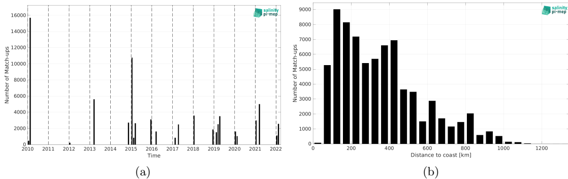
Figure 2: Number of match-ups between TSG (CSIC-UTM) and CCI SSS L4 POLAR SH Merged-OI v4.41 - 7-day running (ESA) SSS as a function of time (a) and as function of the distance to coast (b) over the Roaring Forties and Furious Fifties Pi-MEP region and for the full satellite product period.
