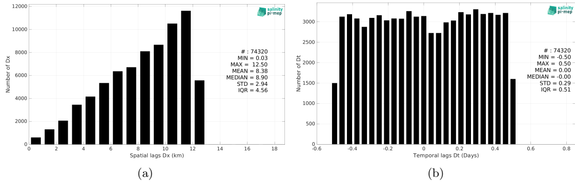
Figure 6: Histograms of the spatial (a) and temporal (b) lags between the location/time of the TSG (CSIC-UTM) measurement and the date of the corresponding CCI SSS L4 POLAR SH Merged-OI v4.41 - 7-day running (ESA) SSS pixel.
