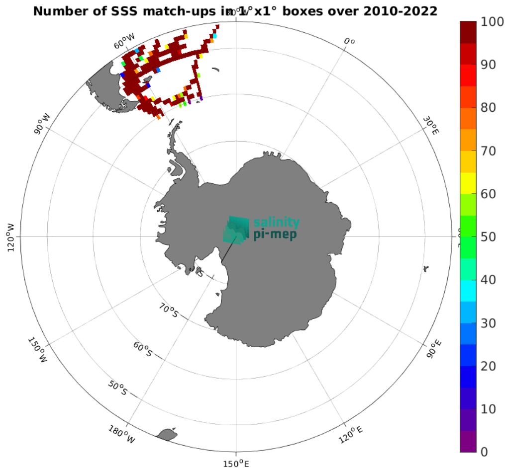
Figure 5: Number of SSS match-ups between TSG (CSIC-UTM) SSS and the CCI SSS L4 POLAR SH Merged-OI v4.41 - 7-day running (ESA) SSS product for the Roaring Forties and Furious Fifties Pi-MEP region over 1^\circ \times 1^\circ boxes and for the full satellite product period.
