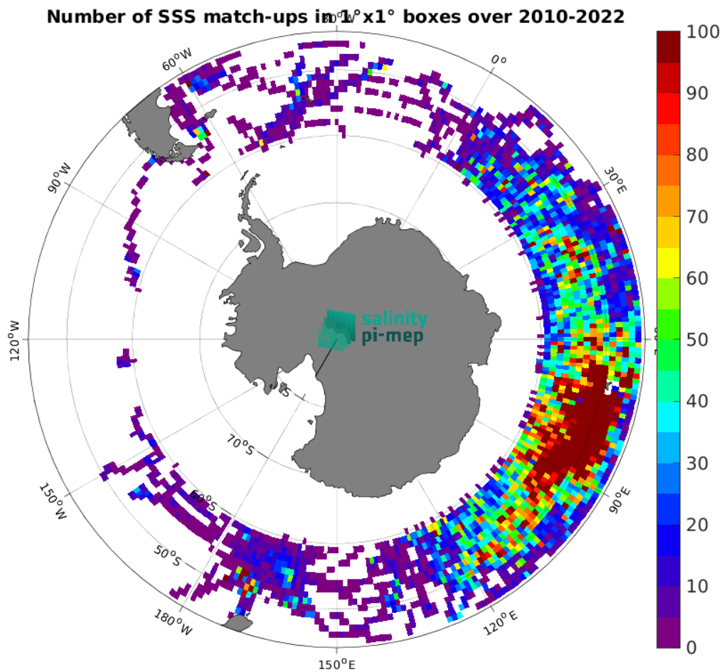
Figure 5: Number of SSS match-ups between Marine mammals SSS and the CCI SSS L4 POLAR SH Merged-OI v4.41 - 7-day running (ESA) SSS product for the Roaring Forties and Furious Fifties Pi-MEP region over 1^\circ \times 1^\circ boxes and for the full satellite product period.
