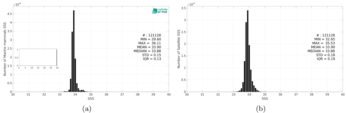
Figure 3: Histograms of SSS from Marine mammals (a) and CCI SSS L4 POLAR SH Merged-OI v4.41 - 7-day running (ESA) (b) considering all match-up pairs per bins of 0.1 over the Roaring Forties and Furious Fifties Pi-MEP region and for the full satellite product period.
