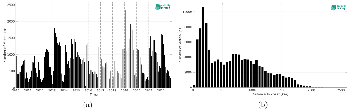
Figure 2: Number of match-ups between Marine mammals and CCI SSS L4 POLAR SH Merged-OI v4.41 - 7-day running (ESA) SSS as a function of time (a) and as function of the distance to coast (b) over the Roaring Forties and Furious Fifties Pi-MEP region and for the full satellite product period.
