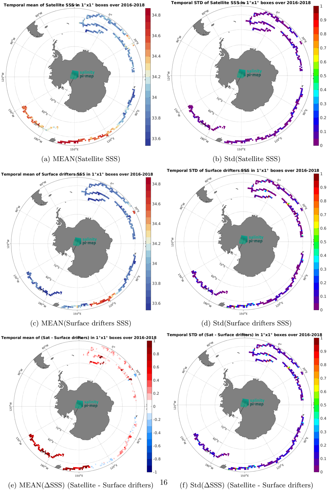
Figure 6: Temporal mean (left) and Std (right) of SSS from CCI SSS L4 POLAR SH Merged-OI v4.41 - 7-day running (ESA) (top), Surface drifters (middle), and of \Delta SSS (Satellite - Surface drifters). Only match-up pairs are used to generate these maps.
