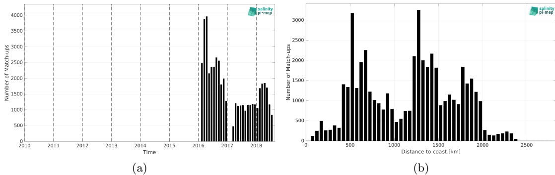
Figure 2: Number of match-ups between Surface drifters and CCI SSS L4 POLAR SH Merged-OI v4.41 - 7-day running (ESA) SSS as a function of time (a) and as function of the distance to coast (b) over the Roaring Forties and Furious Fifties Pi-MEP region and for the full satellite product period.
