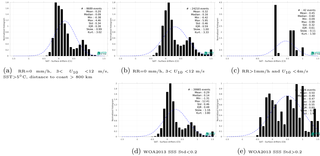
Figure 14: Normalized histogram of \Delta SSS (CCI SSS L4 POLAR SH Merged-OI v4.41 - 7-day running (ESA) - Surface drifters) for 5 different subdatasets corresponding to: RR=0 mm/h, 3 < U_{10} < 12 m/s, SST > 5°C, distance to coast > 800 km (a), RR=0 mm/h, 3 < U_{10} < 12 m/s (b), RR > 1mm/h and U_{10} < 4 m/s (c), WOA2013 SSS Std < 0.2 (d), WOA2013 SSS Std > 0.2 (e).
