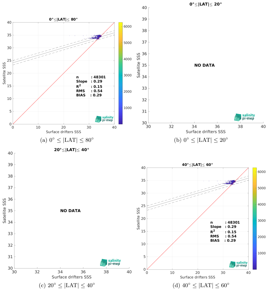
Figure 9: Contour maps of the concentration of CCI SSS L4 POLAR SH Merged-OI v4.41 - 7-day running (ESA) SSS (y-axis) versus Surface drifters SSS (x-axis) at match-up pairs for different latitude bands. For each plot, the red line shows x=y . The black thin and dashed lines indicate a linear fit through the data cloud and the \pm 95\% confidence levels, respectively. The number match-up pairs n , the slope and R^2 coefficient of the linear fit, the root mean square (RMS) and the mean bias between satellite and in situ data are indicated for each latitude band in each plots.
