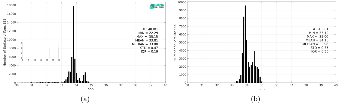
Figure 3: Histograms of SSS from Surface drifters (a) and CCI SSS L4 POLAR SH Merged-OI v4.41 - 7-day running (ESA) (b) considering all match-up pairs per bins of 0.1 over the Roaring Forties and Furious Fifties Pi-MEP region and for the full satellite product period.
