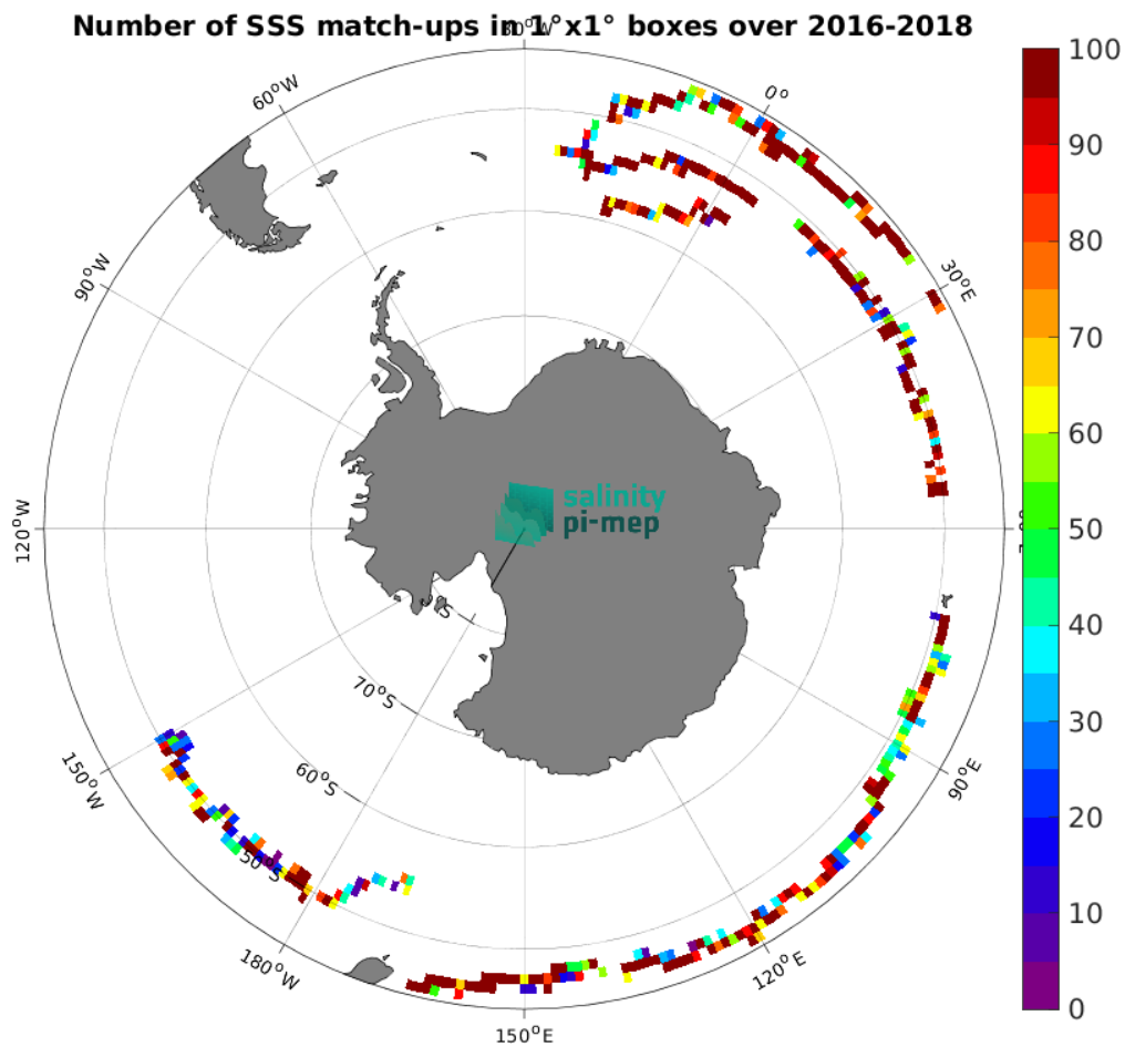
Figure 4: Number of SSS match-ups between Surface drifters SSS and the CCI SSS L4 POLAR SH Merged-OI v4.41 - 7-day running (ESA) SSS product for the Roaring Forties and Furious Fifties Pi-MEP region over 1^\circ \times 1^\circ boxes and for the full satellite product period.
