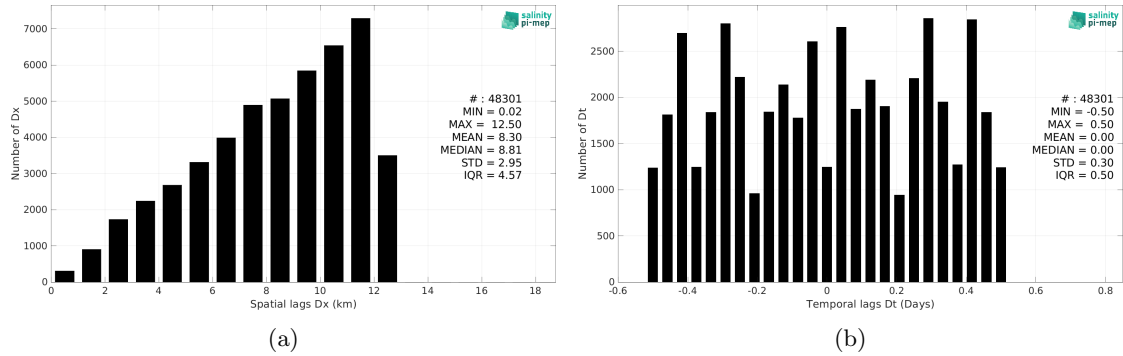
Figure 5: Histograms of the spatial (a) and temporal (b) lags between the location/time of the Surface drifters measurement and the date of the corresponding CCI SSS L4 POLAR SH Merged-OI v4.41 - 7-day running (ESA) SSS pixel.
