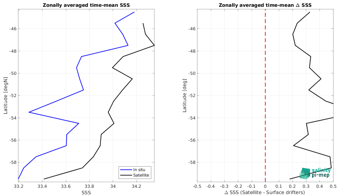
Figure 8: Left panel: Zonal mean SSS from CCI SSS L4 POLAR SH Merged-OI v4.41 - 7-day running (ESA) satellite product (black) and from Surface drifters (blue). Right panel: Zonal mean of \Delta SSS (Satellite - Surface drifters) for all the collected Pi-MEP match-up pairs estimated over the full satellite product period.
