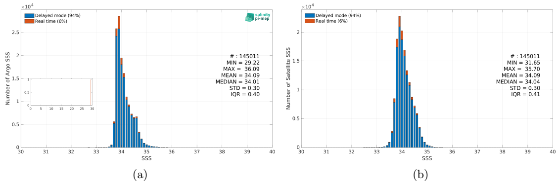
Figure 3: Histograms of SSS from Argo (a) and CCI SSS L4 POLAR SH Merged-OI v4.41 - 7-day running (ESA) (b) considering all match-up pairs per bins of 0.1 over the Roaring Forties and Furious Fifties Pi-MEP region and for the full satellite product period.
