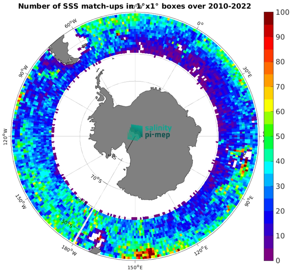
Figure 5: Number of SSS match-ups between Argo SSS and the CCI SSS L4 POLAR SH Merged-OI v4.41 - 7-day running (ESA) SSS product for the Roaring Forties and Furious Fifties Pi-MEP region over 1^\circ \times 1^\circ boxes and for the full satellite product period.
