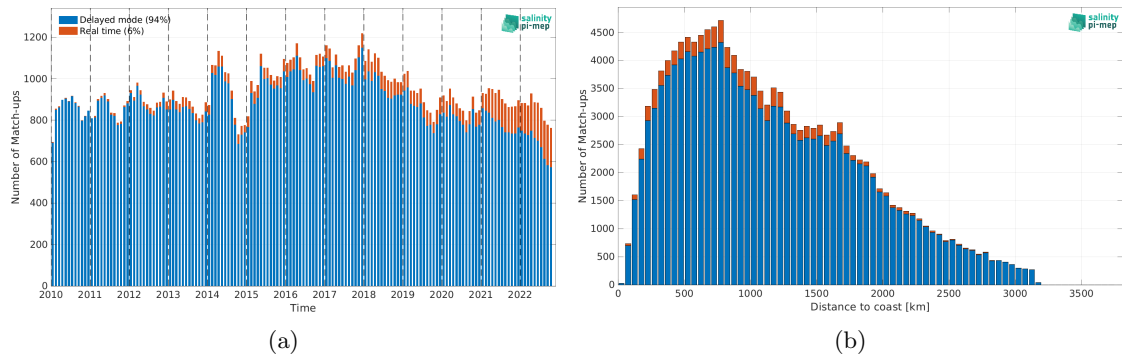
Figure 2: Number of match-ups between Argo and CCI SSS L4 POLAR SH Merged-OI v4.41 - 7-day running (ESA) SSS as a function of time (a) and as function of the distance to coast (b) over the Roaring Forties and Furious Fifties Pi-MEP region and for the full satellite product period.
