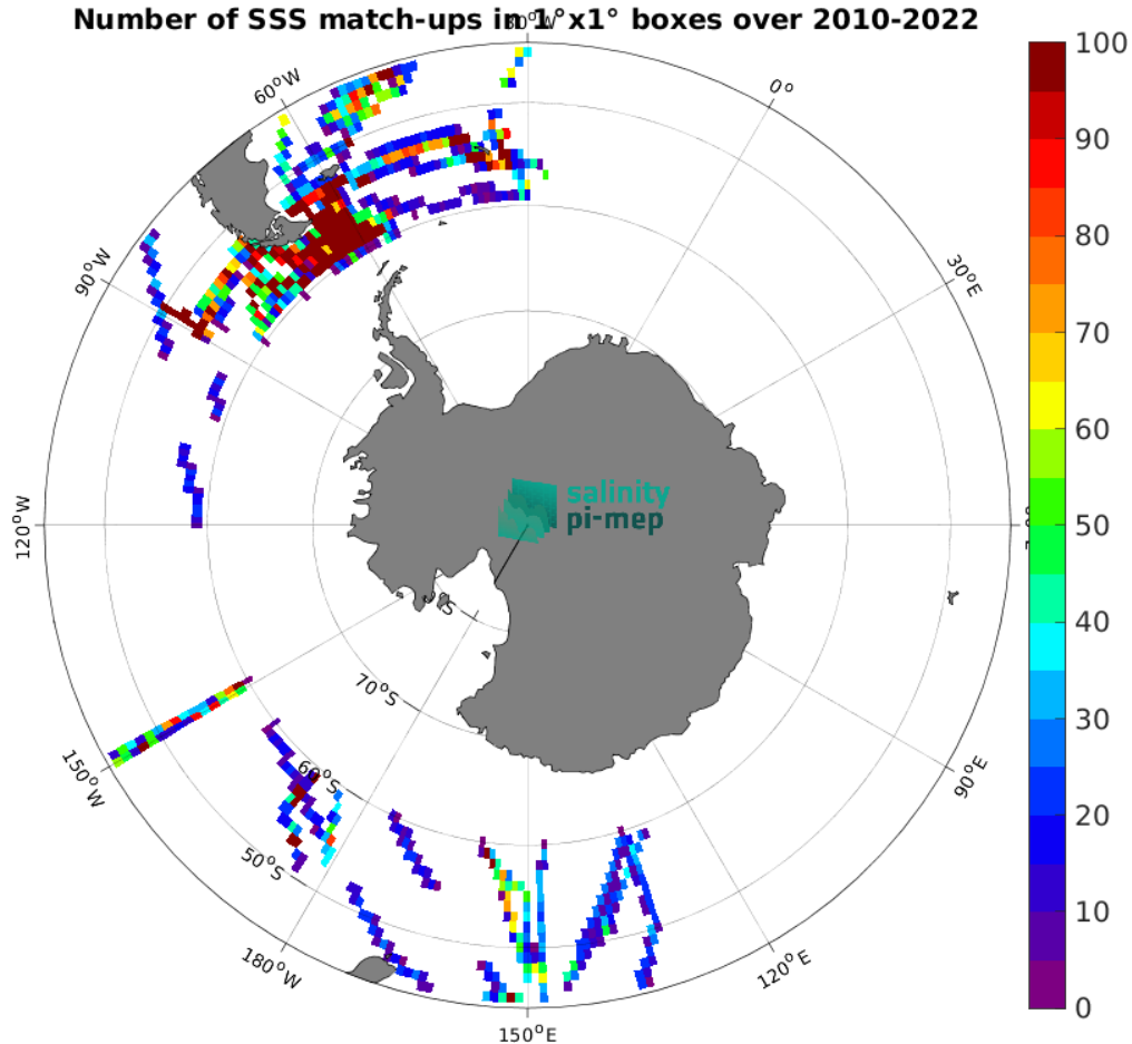
Figure 5: Number of SSS match-ups between TSG (SAMOS) SSS and the CCI SSS L4 POLAR SH Merged-OI v4.41 - 30-day running (ESA) SSS product for the Roaring Forties and Furious Fifties Pi-MEP region over 1^\circ \times 1^\circ boxes and for the full satellite product period.
