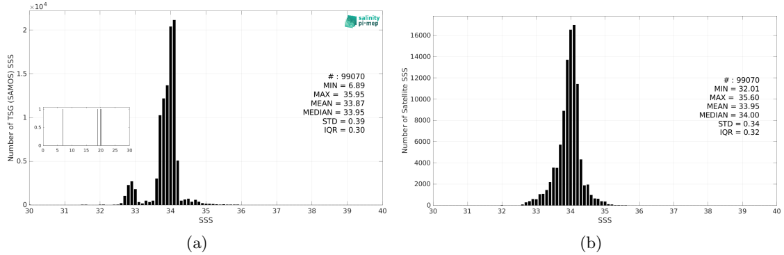
Figure 3: Histograms of SSS from TSG (SAMOS) (a) and CCI SSS L4 POLAR SH Merged-OI v4.41 - 30-day running (ESA) (b) considering all match-up pairs per bins of 0.1 over the Roaring Forties and Furious Fifties Pi-MEP region and for the full satellite product period.
