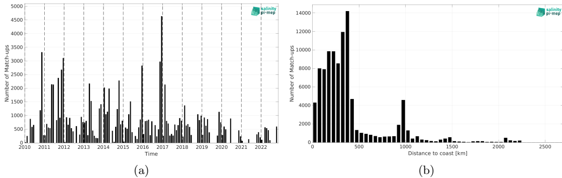
Figure 2: Number of match-ups between TSG (SAMOS) and CCI SSS L4 POLAR SH Merged-OI v4.41 - 30-day running (ESA) SSS as a function of time (a) and as function of the distance to coast (b) over the Roaring Forties and Furious Fifties Pi-MEP region and for the full satellite product period.
