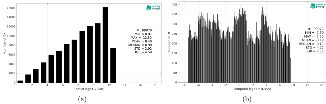
Figure 6: Histograms of the spatial (a) and temporal (b) lags between the location/time of the TSG (SAMOS) measurement and the date of the corresponding CCI SSS L4 POLAR SH Merged-OI v4.41 - 30-day running (ESA) SSS pixel.
