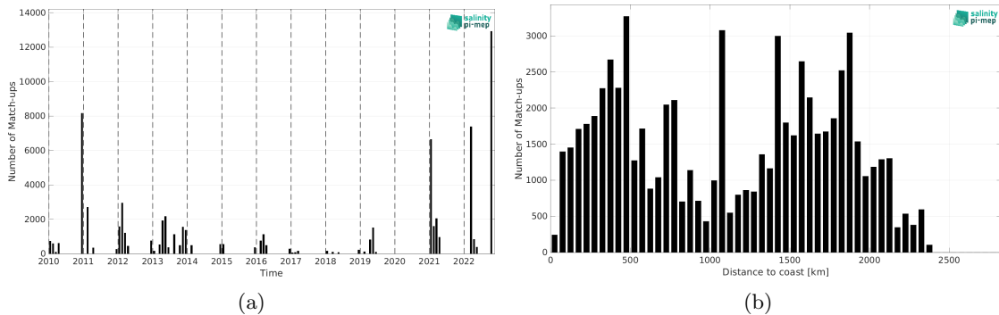
Figure 2: Number of match-ups between TSG (Polarstern) and CCI SSS L4 POLAR SH Merged-OI v4.41 - 30-day running (ESA) SSS as a function of time (a) and as function of the distance to coast (b) over the Roaring Forties and Furious Fifties Pi-MEP region and for the full satellite product period.
