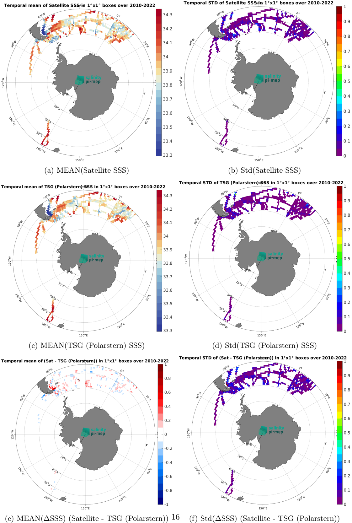
Figure 7: Temporal mean (left) and Std (right) of SSS from CCI SSS L4 POLAR SH Merged-OI v4.41 - 30-day running (ESA) (top), TSG (Polarstern) (middle), and of \Delta SSS (Satellite - TSG (Polarstern)). Only match-up pairs are used to generate these maps.
