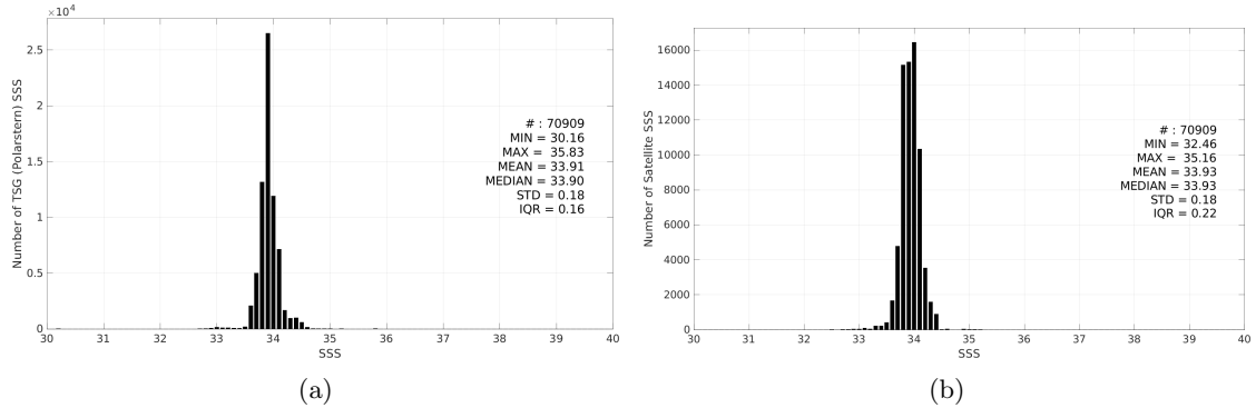
Figure 3: Histograms of SSS from TSG (Polarstern) (a) and CCI SSS L4 POLAR SH Merged-OI v4.41 - 30-day running (ESA) (b) considering all match-up pairs per bins of 0.1 over the Roaring Forties and Furious Fifties Pi-MEP region and for the full satellite product period.
