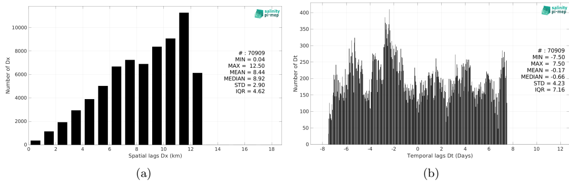
Figure 6: Histograms of the spatial (a) and temporal (b) lags between the location/time of the TSG (Polarstern) measurement and the date of the corresponding CCI SSS L4 POLAR SH Merged-OI v4.41 - 30-day running (ESA) SSS pixel.
