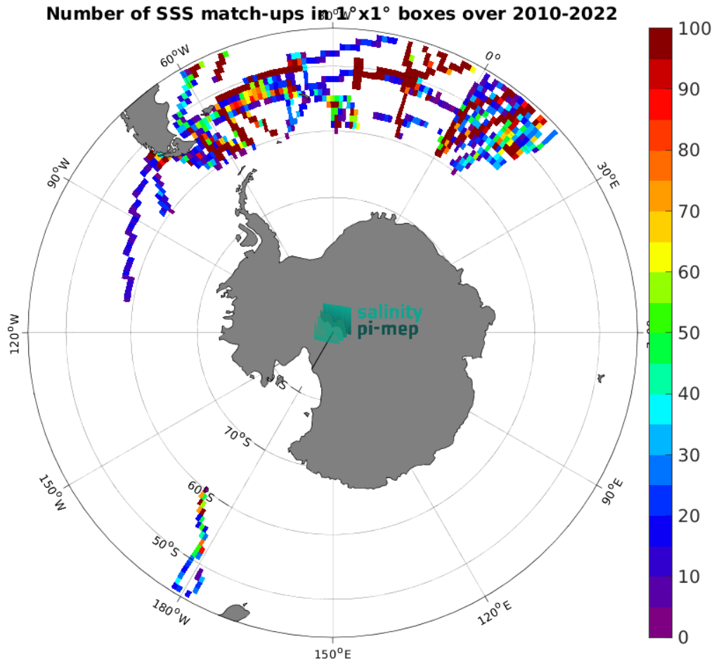
Figure 5: Number of SSS match-ups between TSG (Polarstern) SSS and the CCI SSS L4 POLAR SH Merged-OI v4.41 - 30-day running (ESA) SSS product for the Roaring Forties and Furious Fifties Pi-MEP region over 1^\circ \times 1^\circ boxes and for the full satellite product period.
