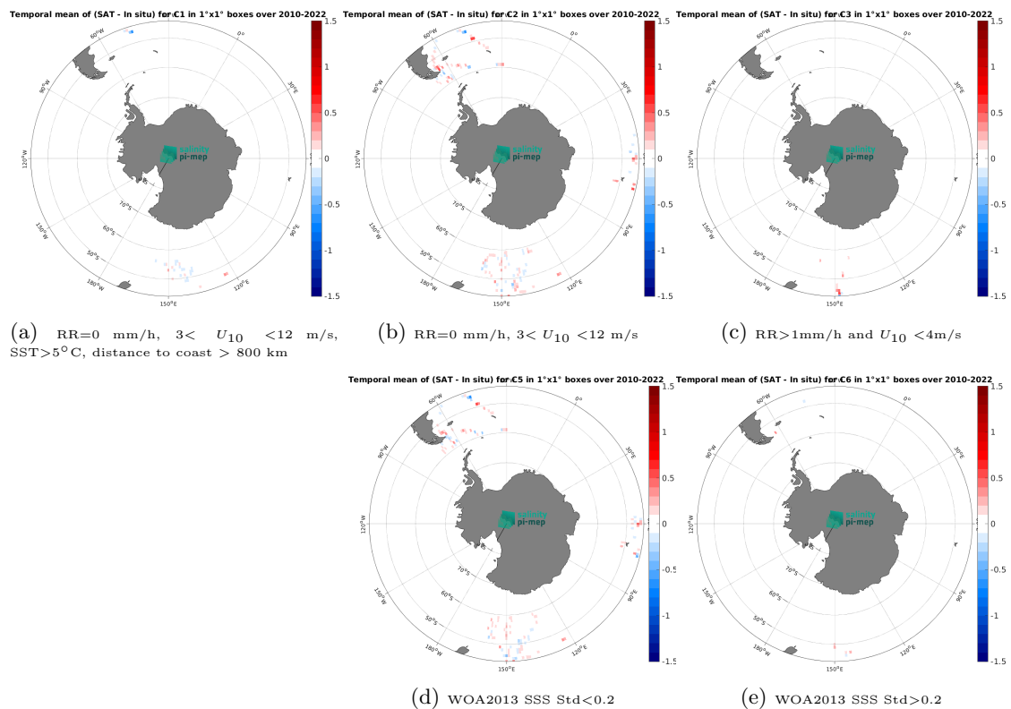
Figure 14: Temporal mean gridded over spatial boxes of size 1^\circ \times 1^\circ of \Delta SSS (CCI SSS L4 POLAR SH Merged-OI v4.41 - 30-day running (ESA) - TSG (LEGOS-DM)) for 5 different subdatasets corresponding to:RR=0 mm/h, 3 < U_{10} < 12 m/s, SST >5^\circ\text{C} , distance to coast > 800 km (a), RR=0 mm/h, 3 < U_{10} < 12 m/s (b), RR >1 mm/h and U_{10} < 4 m/s (c), WOA2013 SSS Std <0.2 (d), WOA2013 SSS Std >0.2 (e).
