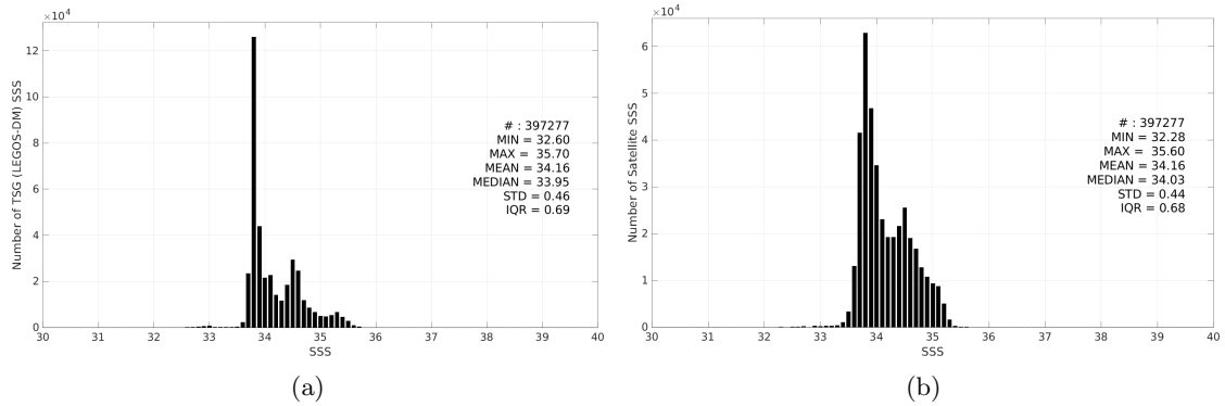
Figure 3: Histograms of SSS from TSG (LEGOS-DM) (a) and CCI SSS L4 POLAR SH Merged-OI v4.41 - 30-day running (ESA) (b) considering all match-up pairs per bins of 0.1 over the Roaring Forties and Furious Fifties Pi-MEP region and for the full satellite product period.
