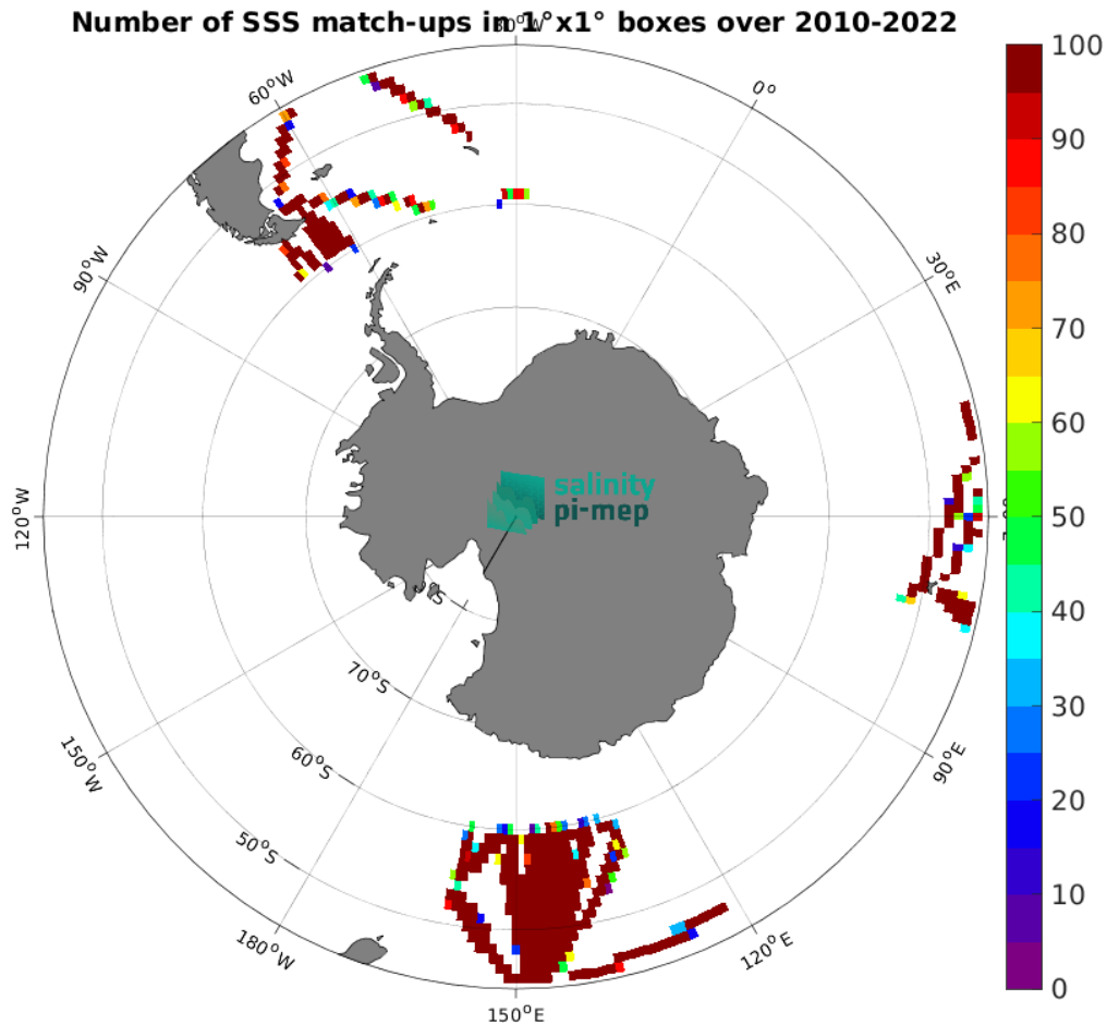
Figure 5: Number of SSS match-ups between TSG (LEGOS-DM) SSS and the CCI SSS L4 POLAR SH Merged-OI v4.41 - 30-day running (ESA) SSS product for the Roaring Forties and Furious Fifties Pi-MEP region over 1^\circ \times 1^\circ boxes and for the full satellite product period.
