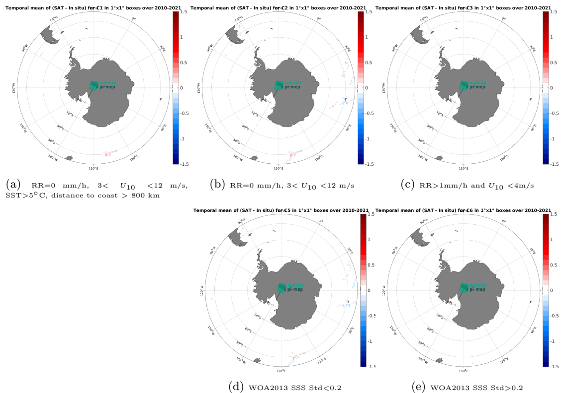
Figure 14: Temporal mean gridded over spatial boxes of size 1^\circ \times 1^\circ of \Delta\text{SSS} (CCI SSS L4 POLAR SH Merged-OI v4.41 - 30-day running (ESA) - TSG (GOSUD-Research-vessel)) for 5 different subdatasets corresponding to:RR=0 mm/h, 3 < U_{10} < 12 m/s, SST>5°C, distance to coast > 800 km (a), RR=0 mm/h, 3 < U_{10} < 12 m/s (b), RR>1mm/h and U_{10} < 4 m/s (c), WOA2013 SSS Std<0.2 (d), WOA2013 SSS Std>0.2 (e).
