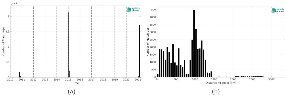
Figure 2: Number of match-ups between TSG (GOSUD-Research-vessel) and CCI SSS L4 POLAR SH Merged-OI v4.41 - 30-day running (ESA) SSS as a function of time (a) and as function of the distance to coast (b) over the Roaring Forties and Furious Fifties Pi-MEP region and for the full satellite product period.
