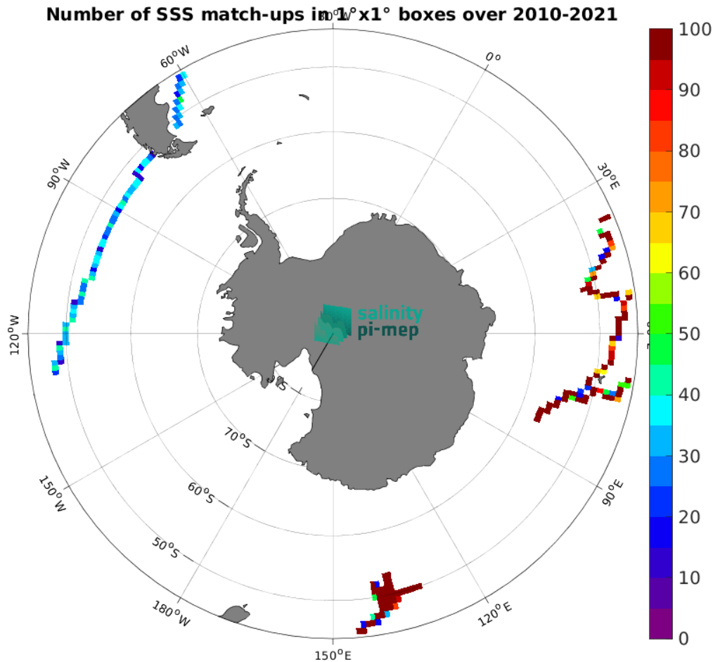
Figure 5: Number of SSS match-ups between TSG (GOSUD-Research-vessel) SSS and the CCI SSS L4 POLAR SH Merged-OI v4.41 - 30-day running (ESA) SSS product for the Roaring Forties and Furious Fifties Pi-MEP region over 1^\circ \times 1^\circ boxes and for the full satellite product period.
