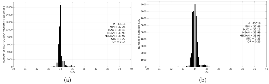
Figure 3: Histograms of SSS from TSG (GOSUD-Research-vessel) (a) and CCI SSS L4 POLAR SH Merged-OI v4.41 - 30-day running (ESA) (b) considering all match-up pairs per bins of 0.1 over the Roaring Forties and Furious Fifties Pi-MEP region and for the full satellite product period.
