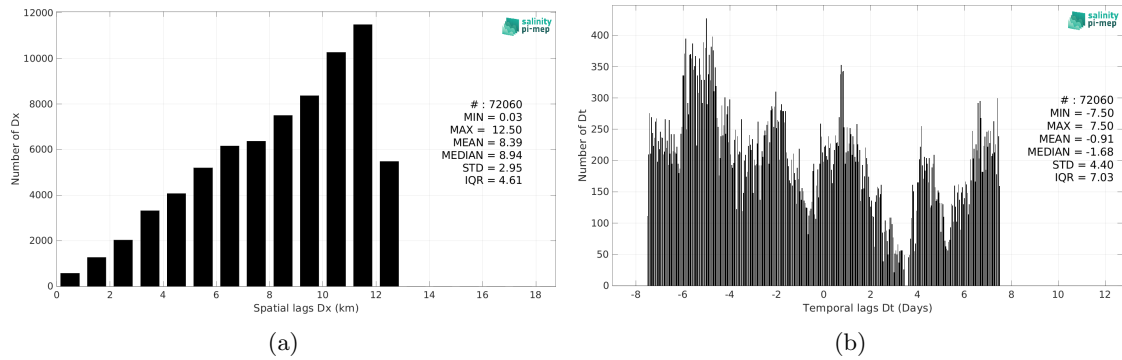
Figure 6: Histograms of the spatial (a) and temporal (b) lags between the location/time of the TSG (CSIC-UTM) measurement and the date of the corresponding CCI SSS L4 POLAR SH Merged-OI v4.41 - 30-day running (ESA) SSS pixel.
