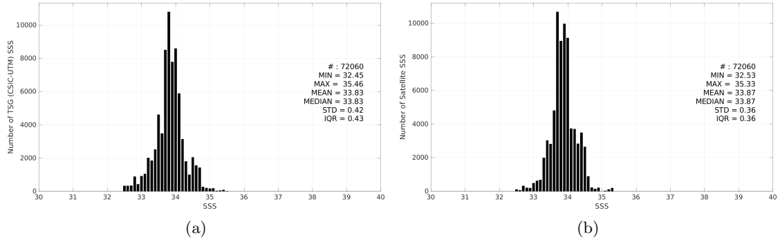
Figure 3: Histograms of SSS from TSG (CSIC-UTM) (a) and CCI SSS L4 POLAR SH Merged-OI v4.41 - 30-day running (ESA) (b) considering all match-up pairs per bins of 0.1 over the Roaring Forties and Furious Fifties Pi-MEP region and for the full satellite product period.
