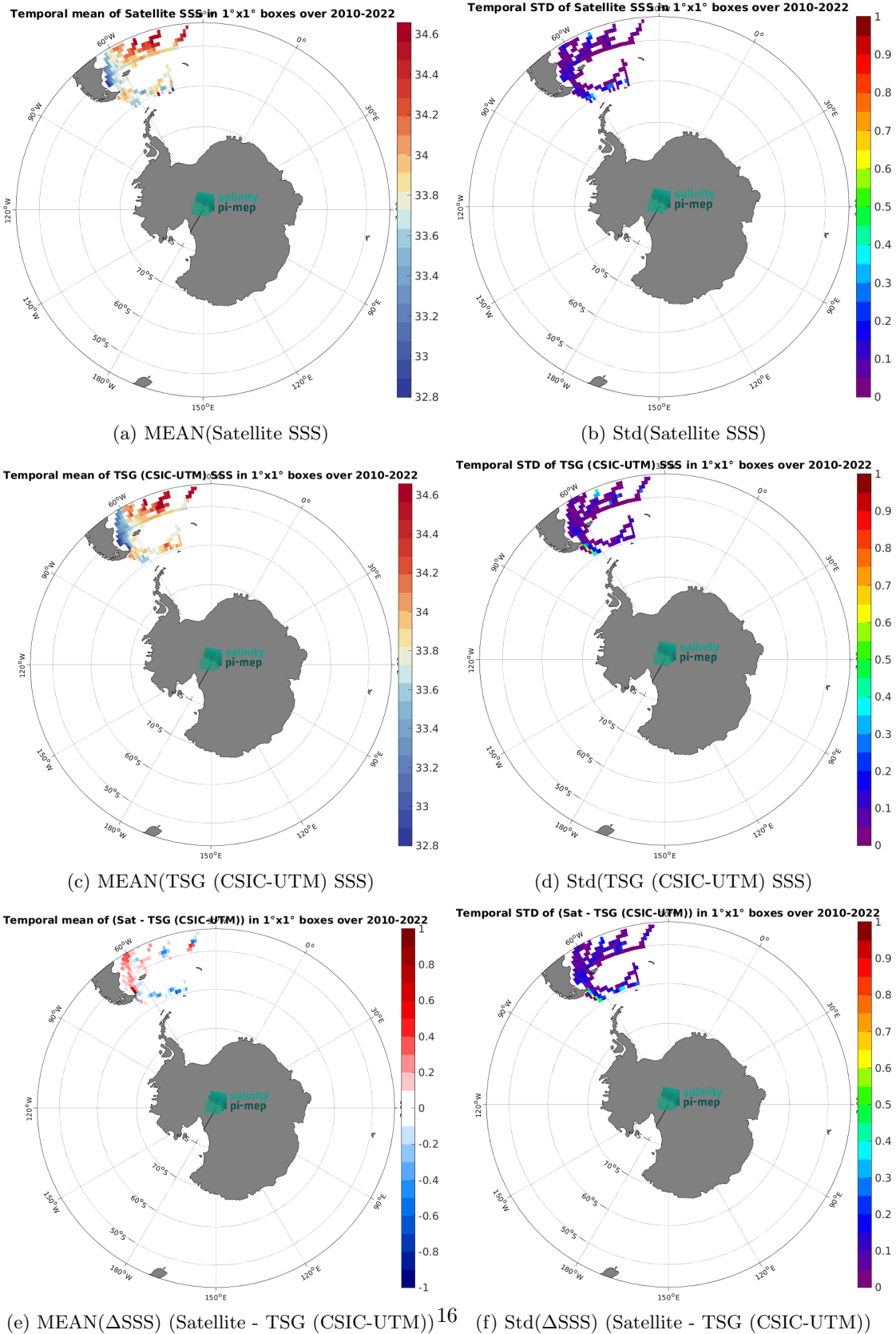
Figure 7: Temporal mean (left) and Std (right) of SSS from CCI SSS L4 POLAR SH Merged-OI v4.41 - 30-day running (ESA) (top), TSG (CSIC-UTM) (middle), and of \Delta SSS (Satellite - TSG (CSIC-UTM)). Only match-up pairs are used to generate these maps.
