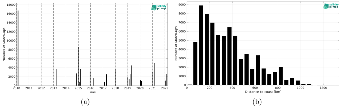
Figure 2: Number of match-ups between TSG (CSIC-UTM) and CCI SSS L4 POLAR SH Merged-OI v4.41 - 30-day running (ESA) SSS as a function of time (a) and as function of the distance to coast (b) over the Roaring Forties and Furious Fifties Pi-MEP region and for the full satellite product period.
