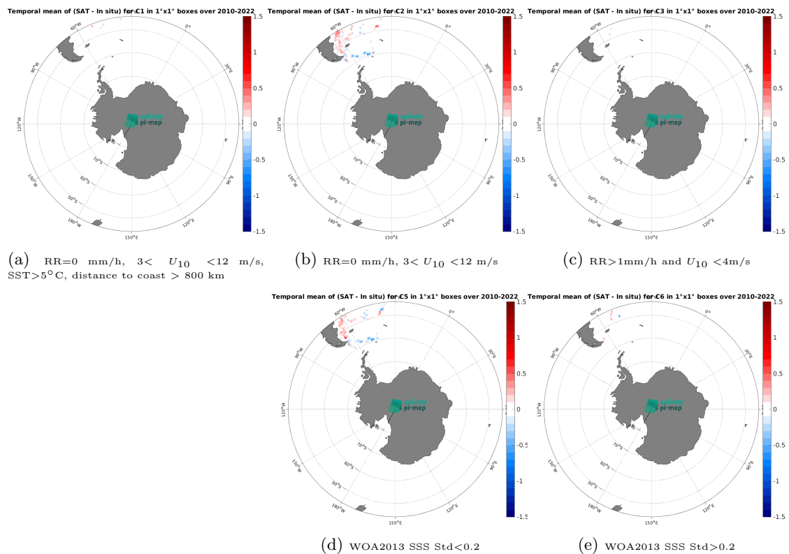
Figure 14: Temporal mean gridded over spatial boxes of size 1^\circ \times 1^\circ of \Delta SSS (CCI SSS L4 POLAR SH Merged-OI v4.41 - 30-day running (ESA) - TSG (CSIC-UTM)) for 5 different subdatasets corresponding to:RR=0 mm/h, 3 < U_{10} < 12 m/s, SST >5^\circ C, distance to coast > 800 km (a), RR=0 mm/h, 3 < U_{10} < 12 m/s (b), RR >1 mm/h and U_{10} < 4 m/s (c), WOA2013 SSS Std <0.2 (d), WOA2013 SSS Std >0.2 (e).
