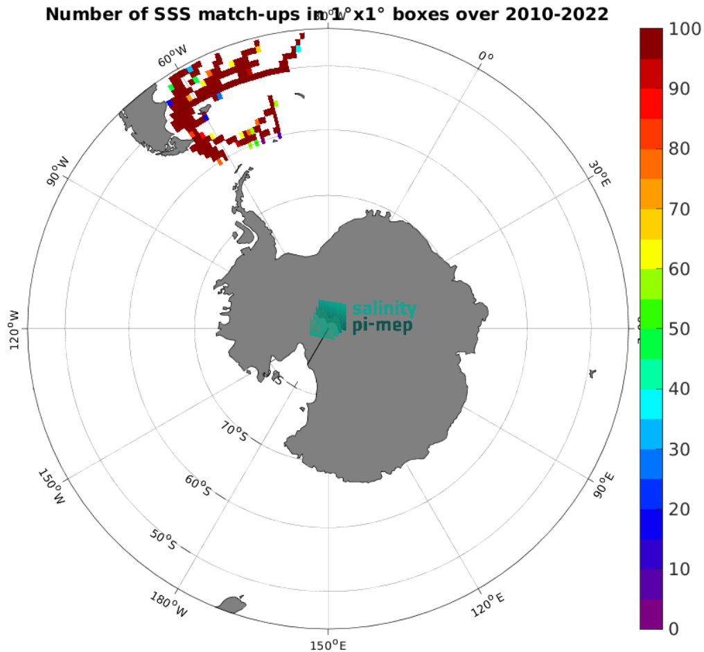
Figure 5: Number of SSS match-ups between TSG (CSIC-UTM) SSS and the CCI SSS L4 POLAR SH Merged-OI v4.41 - 30-day running (ESA) SSS product for the Roaring Forties and Furious Fifties Pi-MEP region over 1^\circ \times 1^\circ boxes and for the full satellite product period.
