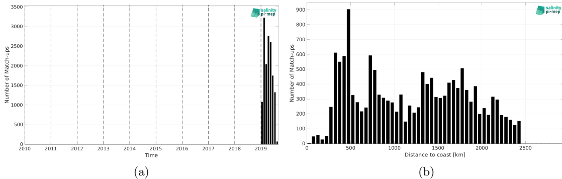
Figure 2: Number of match-ups between Saildrone and CCI SSS L4 POLAR SH Merged-OI v4.41 - 30-day running (ESA) SSS as a function of time (a) and as function of the distance to coast (b) over the Roaring Forties and Furious Fifties Pi-MEP region and for the full satellite product period.
