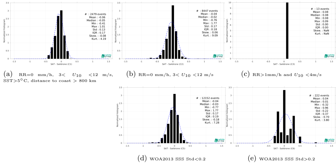
Figure 15: Normalized histogram of \Delta SSS (CCI SSS L4 POLAR SH Merged-OI v4.41 - 30-day running (ESA) - Saldrone) for 5 different subdatasets corresponding to: RR=0 mm/h, 3 < U_{10} < 12 m/s, SST > 5°C, distance to coast > 800 km (a), RR=0 mm/h, 3 < U_{10} < 12 m/s (b), RR > 1mm/h and U_{10} < 4 m/s (c), WOA2013 SSS Std < 0.2 (d), WOA2013 SSS Std > 0.2 (e).
