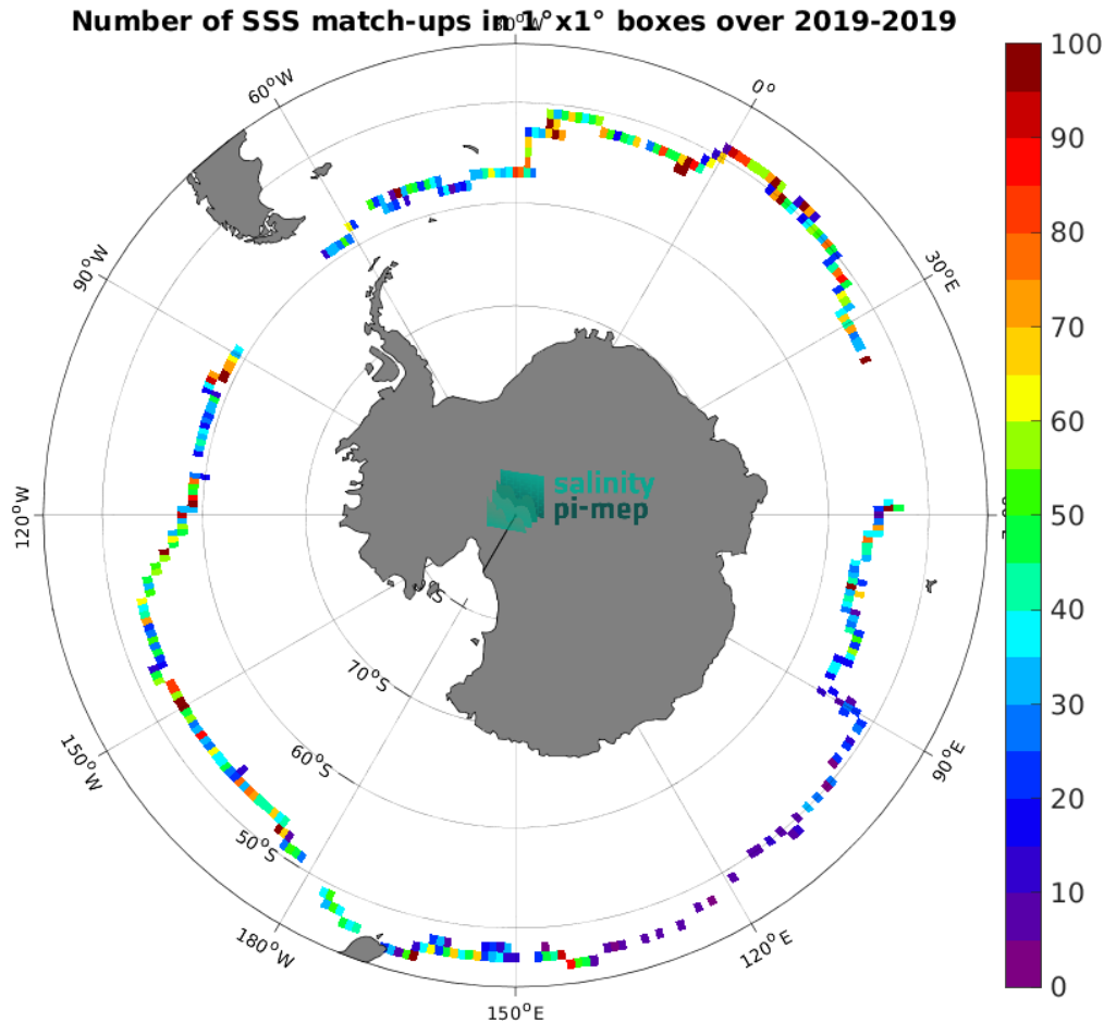
Figure 5: Number of SSS match-ups between Saildrone SSS and the CCI SSS L4 POLAR SH Merged-OI v4.41 - 30-day running (ESA) SSS product for the Roaring Forties and Furious Fifties Pi-MEP region over 1^\circ \times 1^\circ boxes and for the full satellite product period.
