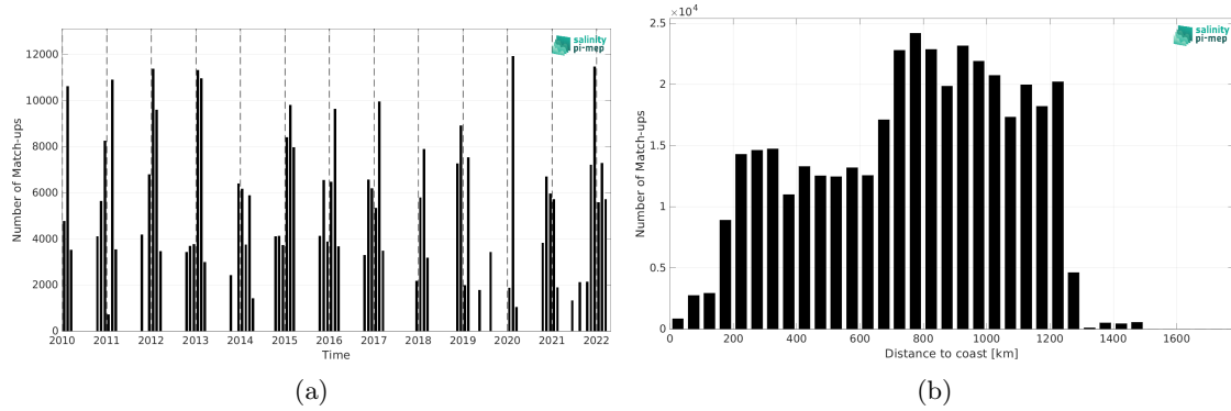
Figure 1: Number of match-ups between TSG (LEGOS-DM) and CCI SSS L4 POLAR SH Merged-OI v4.4 - 7-day running (ESA) SSS as a function of time (a) and as function of the distance to coast (b) over the Roaring Forties and Furious Fifties Pi-MEP region and for the full satellite product period.
