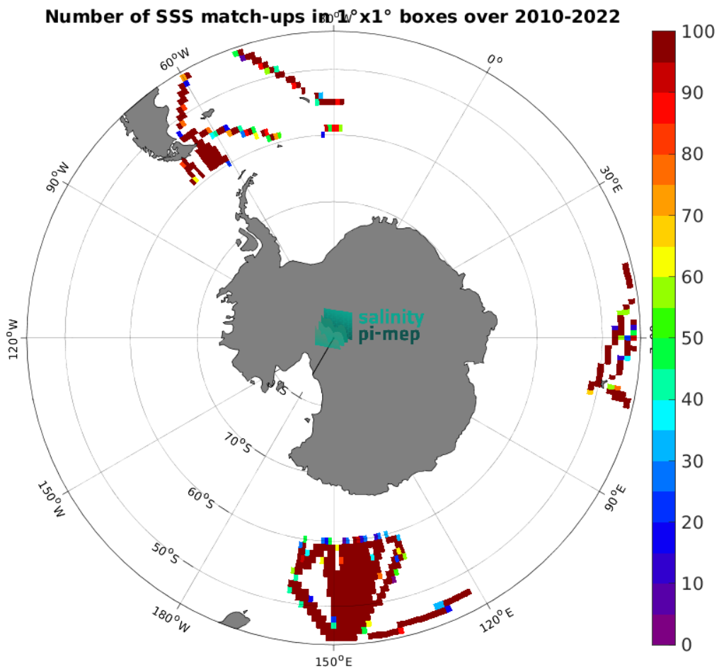
Figure 4: Number of SSS match-ups between TSG (LEGOS-DM) SSS and the CCI SSS L4 POLAR SH Merged-OI v4.4 - 7-day running (ESA) SSS product for the Roaring Forties and Furious Fifties Pi-MEP region over 1^\circ \times 1^\circ boxes and for the full satellite product period.
