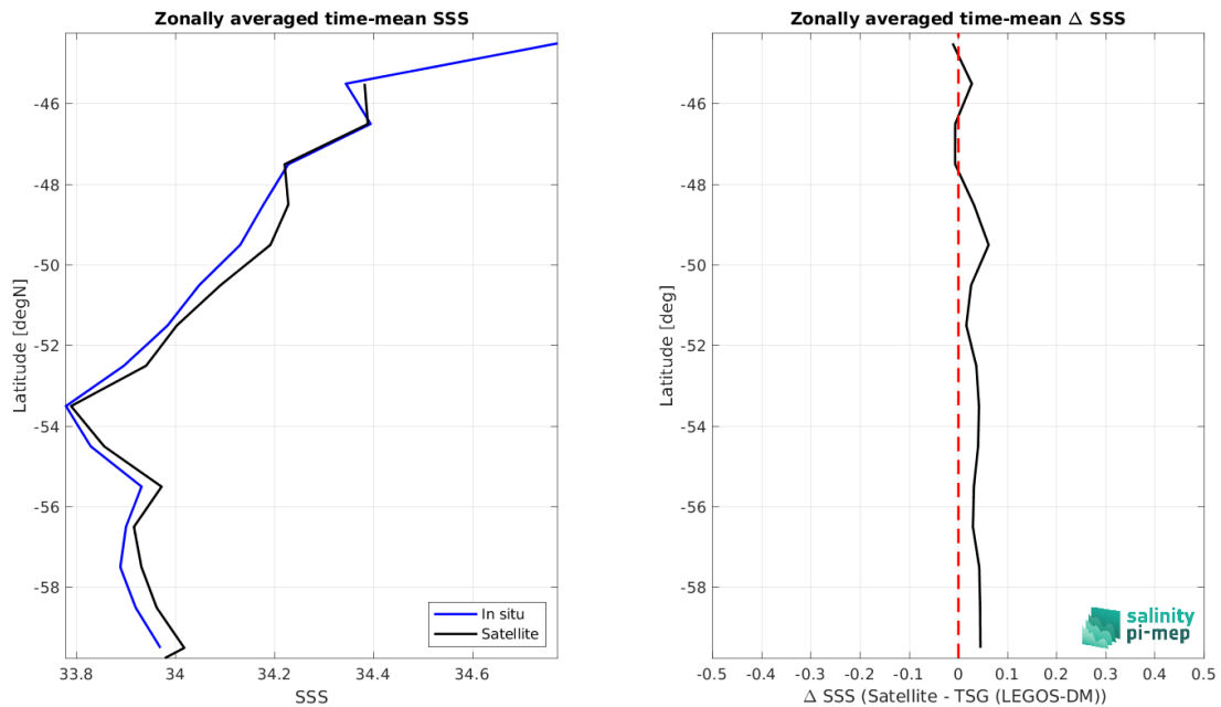
Figure 8: Left panel: Zonal mean SSS from CCI SSS L4 POLAR SH Merged-OI v4.4 - 7-day running (ESA) satellite product (black) and from TSG (LEGOS-DM) (blue). Right panel: Zonal mean of \Delta SSS (Satellite - TSG (LEGOS-DM)) for all the collected Pi-MEP match-up pairs estimated over the full satellite product period.
