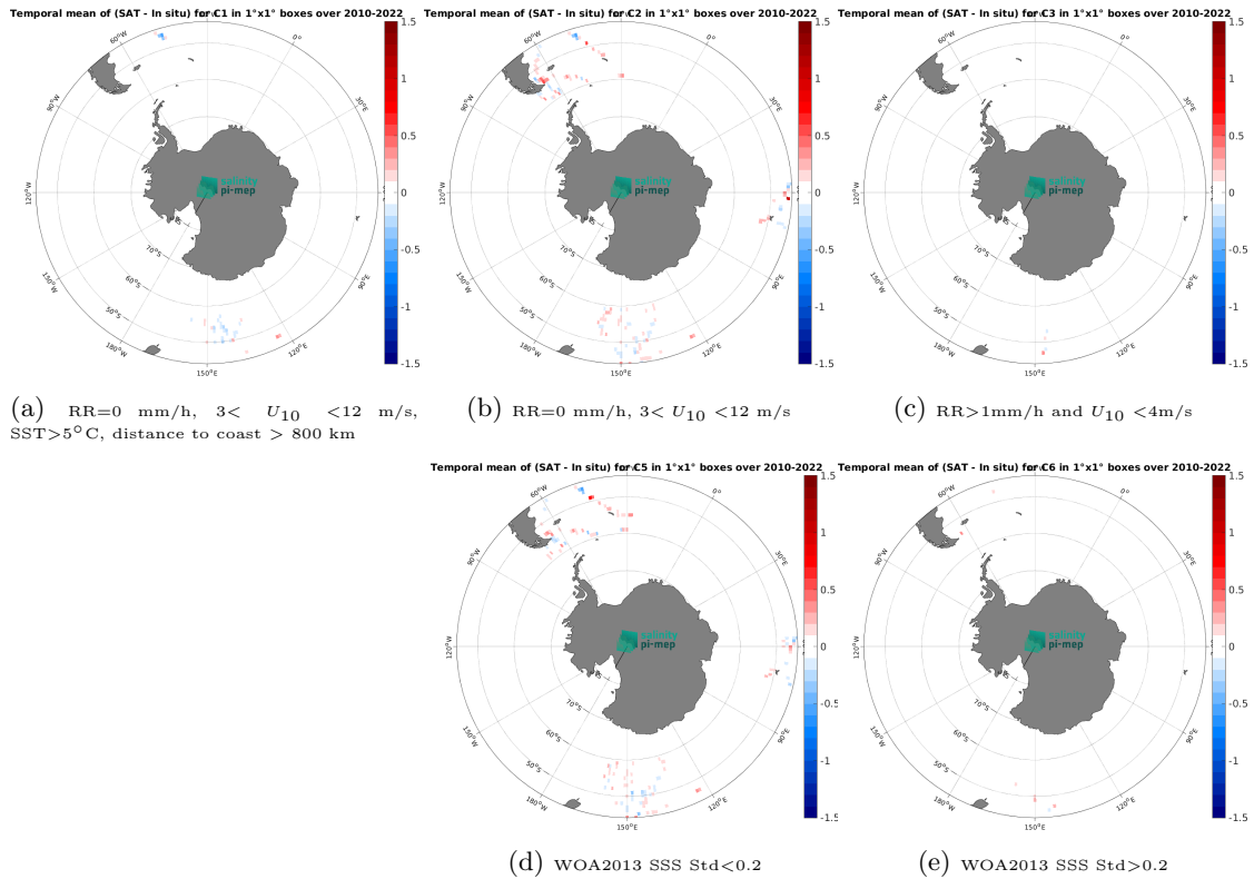
Figure 12: Temporal mean gridded over spatial boxes of size 1^{\circ}\times 1^{\circ} of \Delta\text{SSS} (CCI SSS L4 POLAR SH Merged-OI v4.4 - 7-day running (ESA) - TSG (LEGOS-DM)) for 5 different subdatasets corresponding to:RR=0 mm/h, 3 < U_{10} < 12 m/s, SST >5^{\circ}\text{C} , distance to coast > 800 km (a), RR=0 mm/h, 3 < U_{10} < 12 m/s (b), RR >1 mm/h and U_{10} < 4 m/s (c), WOA2013 SSS Std <0.2 (d), WOA2013 SSS Std >0.2 (e).
