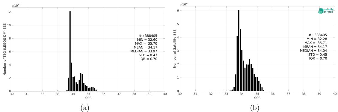
Figure 2: Histograms of SSS from TSG (LEGOS-DM) (a) and CCI SSS L4 POLAR SH Merged-OI v4.4 - 7-day running (ESA) (b) considering all match-up pairs per bins of 0.1 over the Roaring Forties and Furious Fifties Pi-MEP region and for the full satellite product period.
