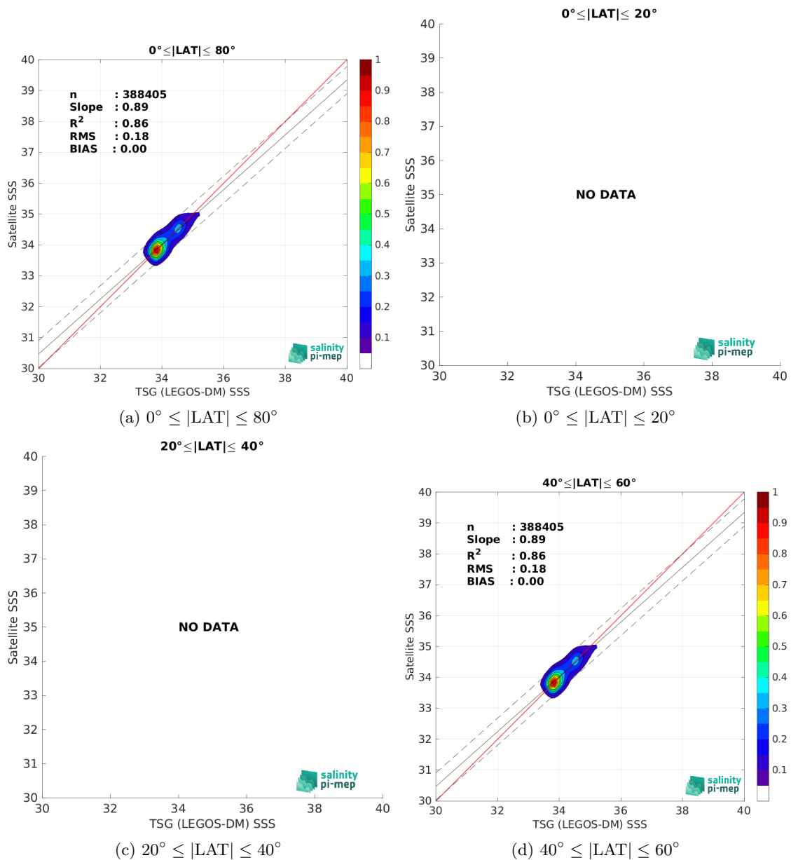
Figure 9: Contour maps of the concentration of CCI SSS L4 POLAR SH Merged-OI v4.4 - 7-day running (ESA) SSS (y-axis) versus TSG (LEGOS-DM) SSS (x-axis) at match-up pairs for different latitude bands. For each plot, the red line shows x=y . The black thin and dashed lines indicate a linear fit through the data cloud and the \pm 95\% confidence levels, respectively. The number match-up pairs n , the slope and R^2 coefficient of the linear fit, the root mean square (RMS) and the mean bias between satellite and in situ data are indicated for each latitude band in each plots.
