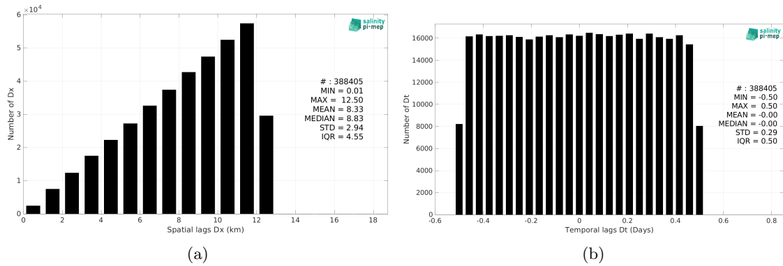
Figure 5: Histograms of the spatial (a) and temporal (b) lags between the location/time of the TSG (LEGOS-DM) measurement and the date of the corresponding CCI SSS L4 POLAR SH Merged-OI v4.4 - 7-day running (ESA) SSS pixel.
