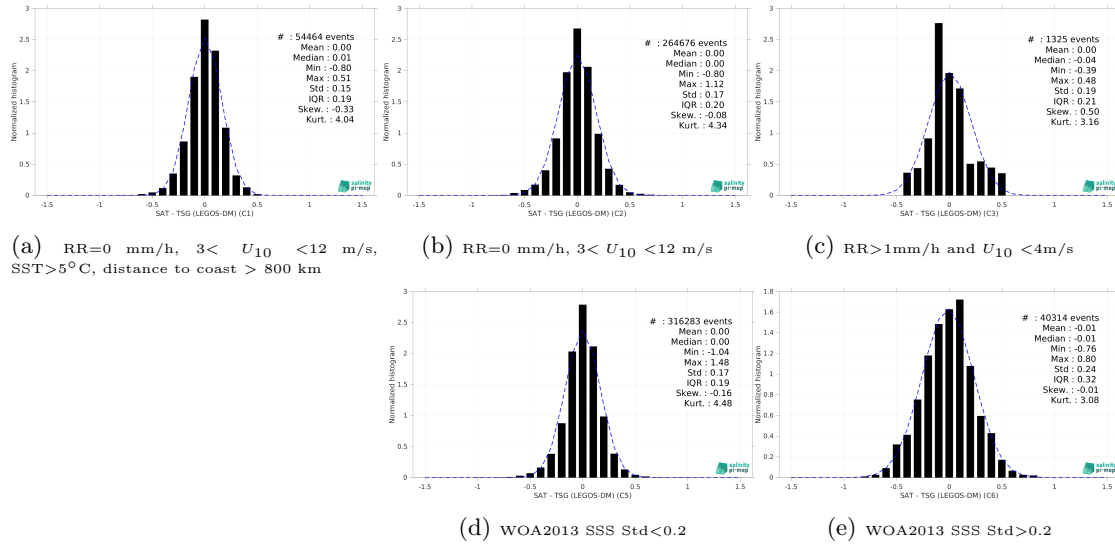
Figure 13: Normalized histogram of \Delta SSS (CCI SSS L4 POLAR SH Merged-OI v4.4 - 7-day running (ESA) - TSG (LEGOS-DM)) for 5 different subdatasets corresponding to: RR=0 mm/h, 3 < U_{10} < 12 m/s, SST>5°C, distance to coast > 800 km (a), RR=0 mm/h, 3 < U_{10} < 12 m/s (b), RR>1mm/h and U_{10} < 4 m/s (c), WOA2013 SSS Std<0.2 (d), WOA2013 SSS Std>0.2 (e).
