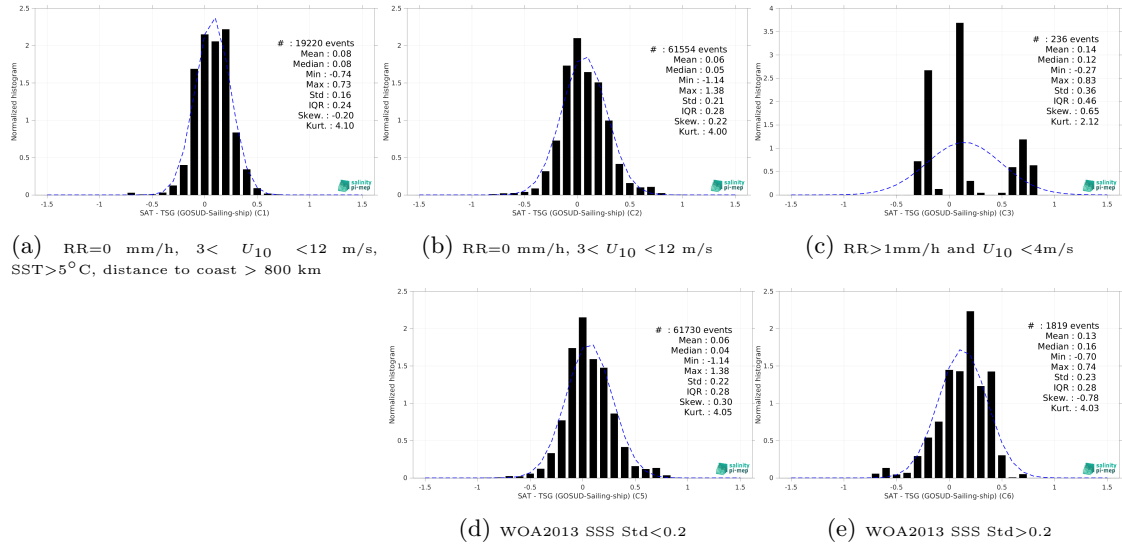
Figure 13: Normalized histogram of \Delta\text{SSS} (CCI SSS L4 POLAR SH Merged-OI v4.4 - 7-day running (ESA) - TSG (GOSUD-Sailing-ship)) for 5 different subdatasets corresponding to: RR=0 mm/h, 3 < U_{10} < 12 m/s, SST>5°C, distance to coast > 800 km (a), RR=0 mm/h, 3 < U_{10} < 12 m/s (b), RR>1mm/h and U_{10} < 4 m/s (c), WOA2013 SSS Std<0.2 (d), WOA2013 SSS Std>0.2 (e).
