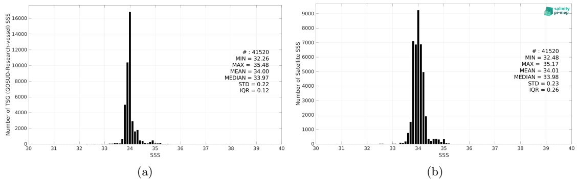
Figure 2: Histograms of SSS from TSG (GOSUD-Research-vessel) (a) and CCI SSS L4 POLAR SH Merged-OI v4.4 - 7-day running (ESA) (b) considering all match-up pairs per bins of 0.1 over the Roaring Forties and Furious Fifties Pi-MEP region and for the full satellite product period.
