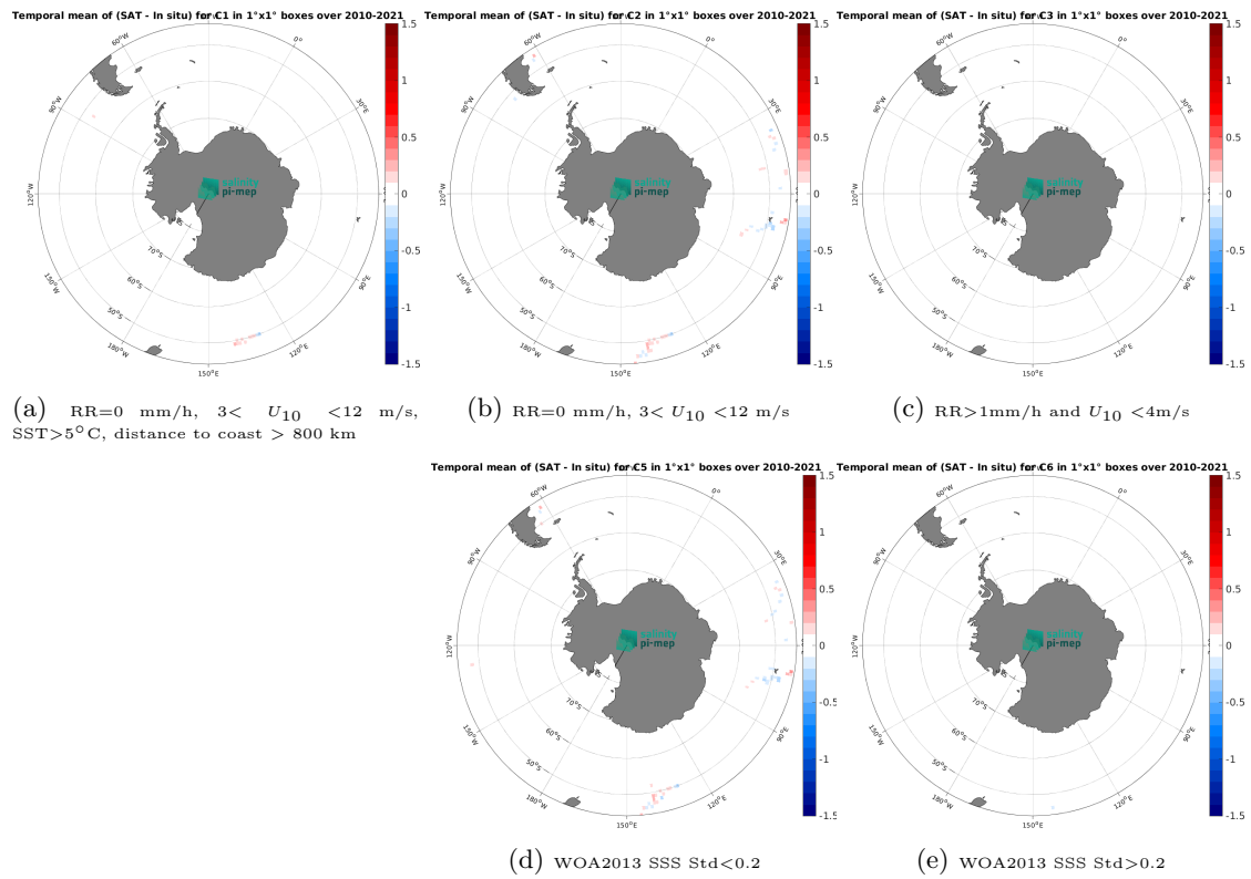
Figure 12: Temporal mean gridded over spatial boxes of size 1^\circ \times 1^\circ of \Delta SSS (CCI SSS L4 POLAR SH Merged-OI v4.4 - 7-day running (ESA) - TSG (GOSUD-Research-vessel)) for 5 different subdatasets corresponding to: RR=0 mm/h, 3 < U_{10} < 12 m/s, SST>5°C, distance to coast > 800 km (a), RR=0 mm/h, 3 < U_{10} < 12 m/s (b), RR>1mm/h and U_{10} < 4 m/s (c), WOA2013 SSS Std<0.2 (d), WOA2013 SSS Std>0.2 (e).
