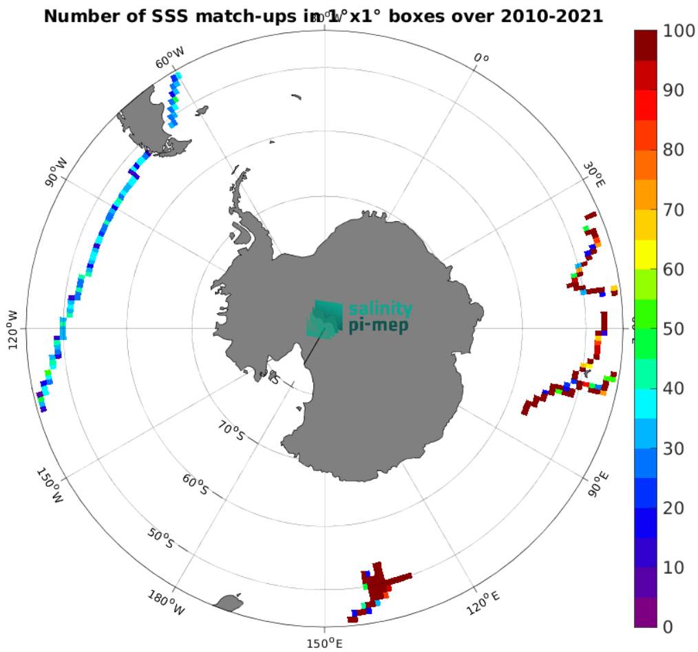
Figure 4: Number of SSS match-ups between TSG (GOSUD-Research-vessel) SSS and the CCI SSS L4 POLAR SH Merged-OI v4.4 - 7-day running (ESA) SSS product for the Roaring Forties and Furious Fifties Pi-MEP region over 1^{\circ} \times 1^{\circ} boxes and for the full satellite product period.
