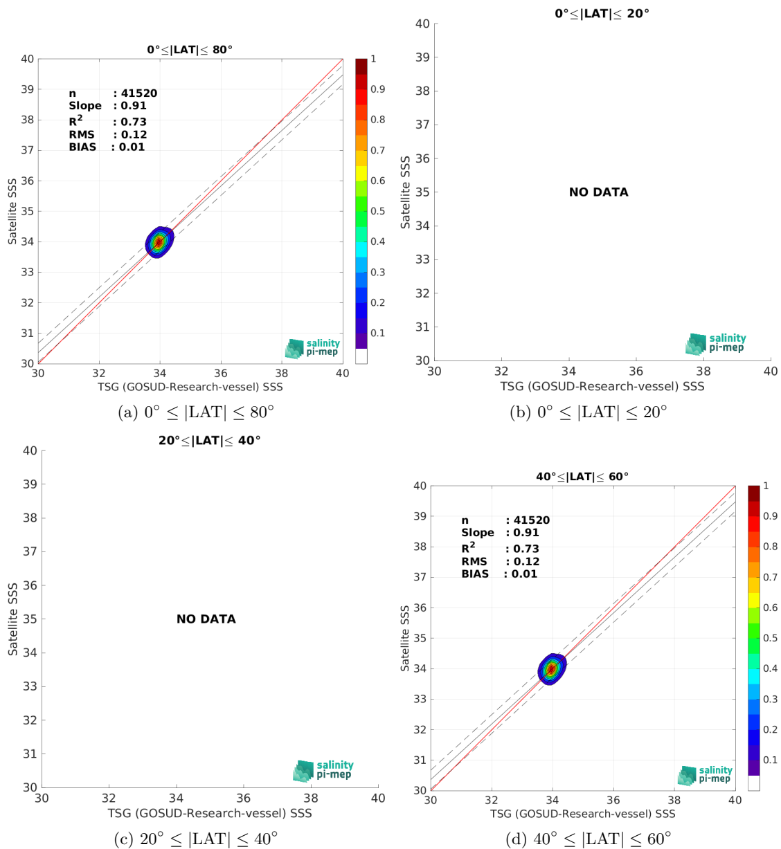
Figure 9: Contour maps of the concentration of CCI SSS L4 POLAR SH Merged-OI v4.4 - 7-day running (ESA) SSS (y-axis) versus TSG (GOSUD-Research-vessel) SSS (x-axis) at match-up pairs for different latitude bands. For each plot, the red line shows x=y . The black thin and dashed lines indicate a linear fit through the data cloud and the \pm 95\% confidence levels, respectively. The number match-up pairs n , the slope and R^2 coefficient of the linear fit, the root mean square (RMS) and the mean bias between satellite and in situ data are indicated for each latitude band in each plots.
