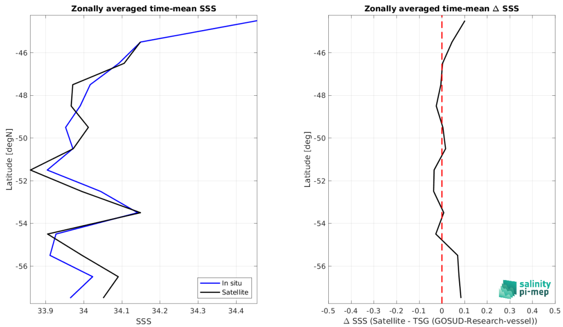
Figure 8: Left panel: Zonal mean SSS from CCI SSS L4 POLAR SH Merged-OI v4.4 - 7-day running (ESA) satellite product (black) and from TSG (GOSUD-Research-vessel) (blue). Right panel: Zonal mean of \Delta SSS (Satellite - TSG (GOSUD-Research-vessel)) for all the collected Pi-MEP match-up pairs estimated over the full satellite product period.
