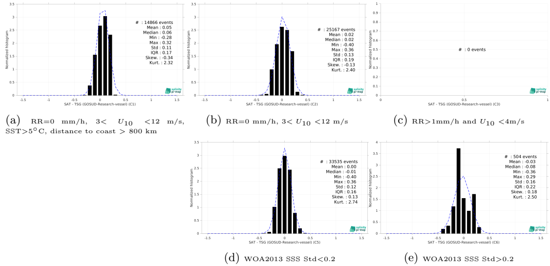
Figure 13: Normalized histogram of \Delta SSS (CCI SSS L4 POLAR SH Merged-OI v4.4 - 7-day running (ESA) - TSG (GOSUD-Research-vessel)) for 5 different subdatasets corresponding to: RR=0 mm/h, 3 < U_{10} < 12 m/s, SST>5°C, distance to coast > 800 km (a), RR=0 mm/h, 3 < U_{10} < 12 m/s (b), RR>1mm/h and U_{10} < 4 m/s (c), WOA2013 SSS Std<0.2 (d), WOA2013 SSS Std>0.2 (e).
