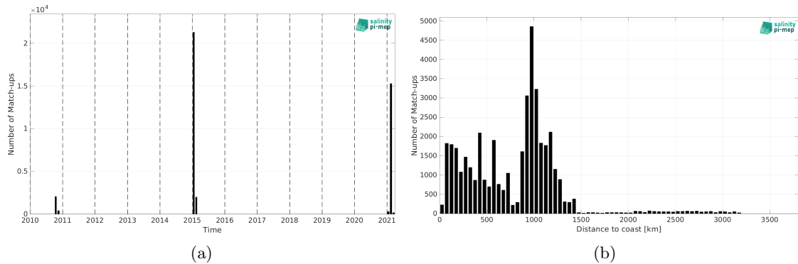
Figure 1: Number of match-ups between TSG (GOSUD-Research-vessel) and CCI SSS L4 POLAR SH Merged-OI v4.4 - 7-day running (ESA) SSS as a function of time (a) and as function of the distance to coast (b) over the Roaring Forties and Furious Fifties Pi-MEP region and for the full satellite product period.
