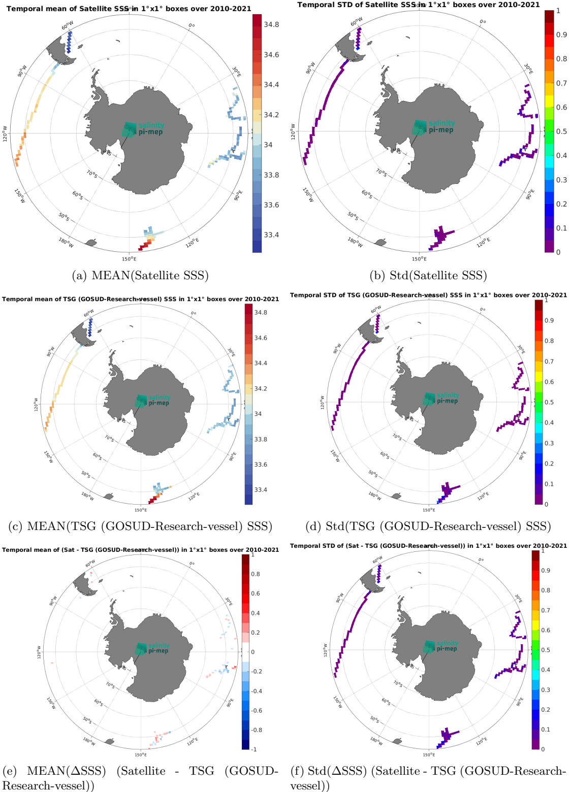
Figure 6: Temporal mean (left) and Std (right) of SSS from CCI SSS L4 POLAR SH Merged-OI v4.4 - 7-day running (ESA) (top), TSG (GOSUD-Research-vessel) (middle), and of \Delta SSS (Satellite - TSG (GOSUD-Research-vessel)). Only match-up pairs are used to generate these maps.
