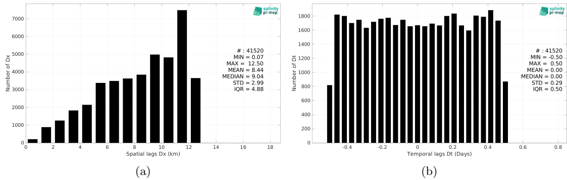
Figure 5: Histograms of the spatial (a) and temporal (b) lags between the location/time of the TSG (GOSUD-Research-vessel) measurement and the date of the corresponding CCI SSS L4 POLAR SH Merged-OI v4.4 - 7-day running (ESA) SSS pixel.
