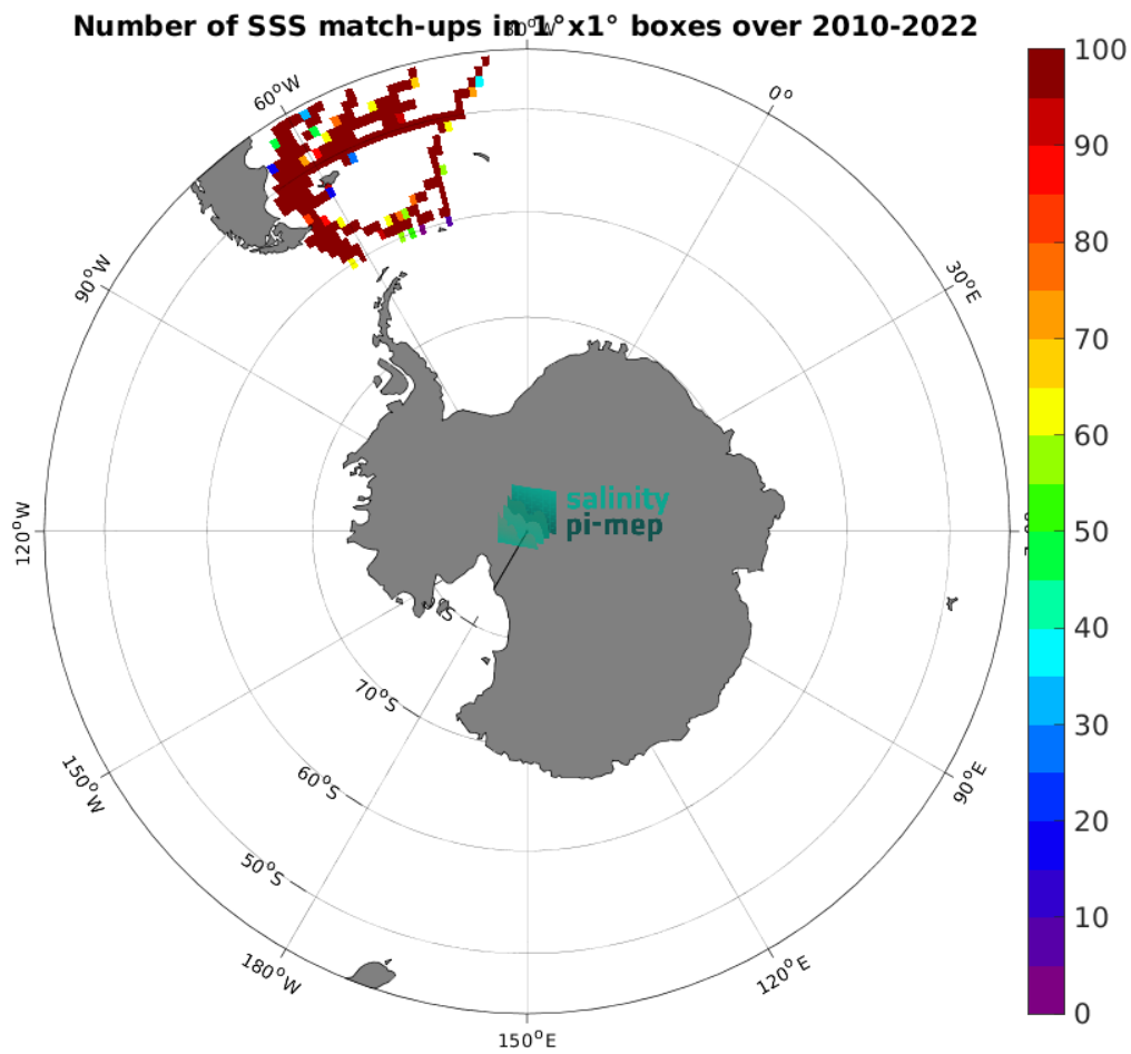
Figure 4: Number of SSS match-ups between TSG (CSIC-UTM) SSS and the CCI SSS L4 POLAR SH Merged-OI v4.4 - 7-day running (ESA) SSS product for the Roaring Forties and Furious Fifties Pi-MEP region over 1^\circ \times 1^\circ boxes and for the full satellite product period.
