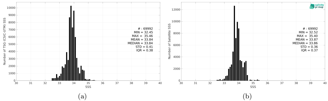
Figure 2: Histograms of SSS from TSG (CSIC-UTM) (a) and CCI SSS L4 POLAR SH Merged-OI v4.4 - 7-day running (ESA) (b) considering all match-up pairs per bins of 0.1 over the Roaring Forties and Furious Fifties Pi-MEP region and for the full satellite product period.
