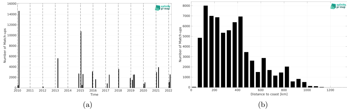
Figure 1: Number of match-ups between TSG (CSIC-UTM) and CCI SSS L4 POLAR SH Merged-OI v4.4 - 7-day running (ESA) SSS as a function of time (a) and as function of the distance to coast (b) over the Roaring Forties and Furious Fifties Pi-MEP region and for the full satellite product period.
