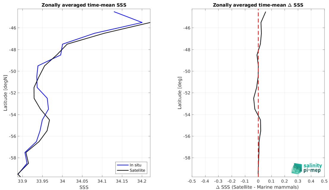
Figure 8: Left panel: Zonal mean SSS from CCI SSS L4 POLAR SH Merged-OI v4.4 - 7-day running (ESA) satellite product (black) and from Marine mammals (blue). Right panel: Zonal mean of \Delta SSS (Satellite - Marine mammals) for all the collected Pi-MEP match-up pairs estimated over the full satellite product period.
