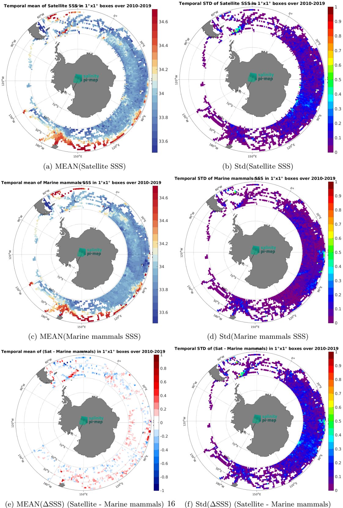
Figure 6: Temporal mean (left) and Std (right) of SSS from CCI SSS L4 POLAR SH Merged-OI v4.4 - 7-day running (ESA) (top), Marine mammals (middle), and of \Delta SSS (Satellite - Marine mammals). Only match-up pairs are used to generate these maps.
