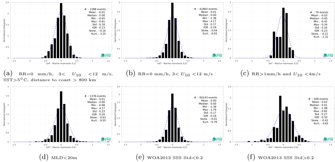
Figure 13: Normalized histogram of \Delta SSS (CCI SSS L4 POLAR SH Merged-OI v4.4 - 7-day running (ESA) - Marine mammals) for 6 different subdatasets corresponding to: RR=0 mm/h, 3 < U_{10} < 12 m/s, SST>5°C, distance to coast > 800 km (a), RR=0 mm/h, 3 < U_{10} < 12 m/s (b), RR>1mm/h and U_{10} < 4 m/s (c), MLD<20m (d), WOA2013 SSS Std<0.2 (e), WOA2013 SSS Std>0.2 (f).
