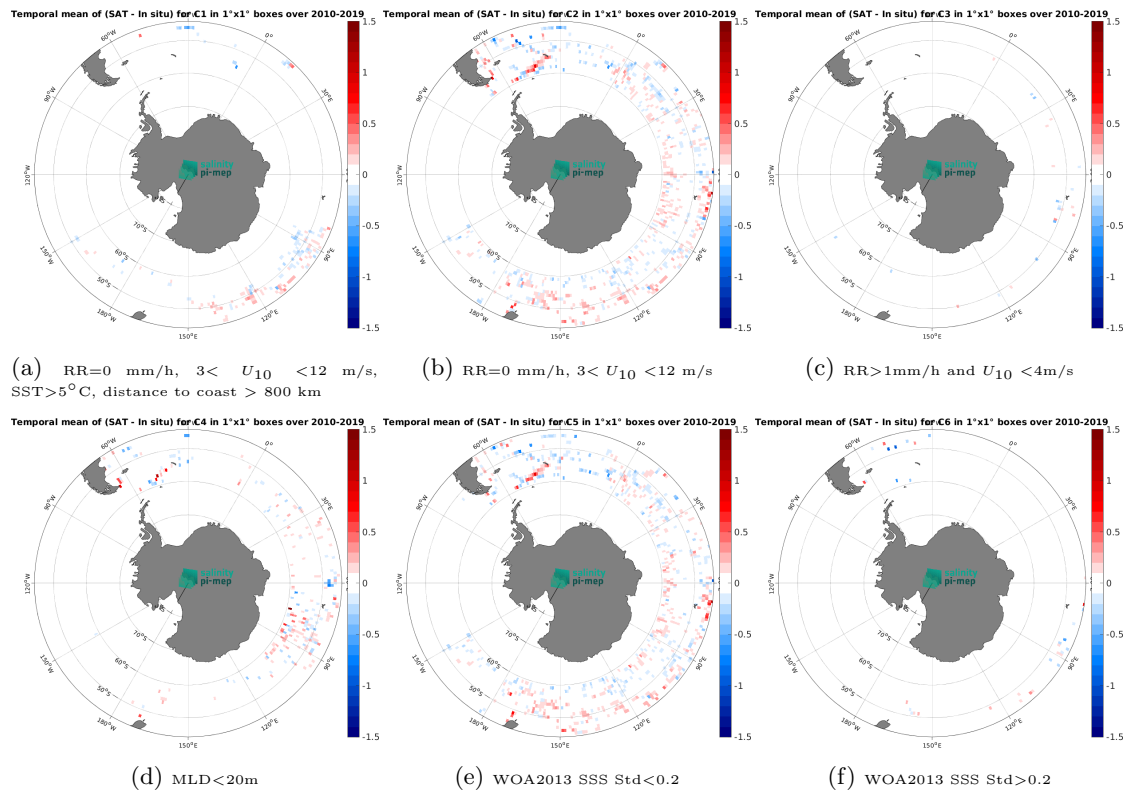
Figure 12: Temporal mean gridded over spatial boxes of size 1^{\circ}\times 1^{\circ} of \Delta\text{SSS} (CCI SSS L4 POLAR SH Merged-OI v4.4 - 7-day running (ESA) - Marine mammals) for 6 different subdatasets corresponding to:RR=0 mm/h, 3 < U_{10} < 12 m/s, SST > 5^{\circ}\text{C} , distance to coast > 800 km (a), RR=0 mm/h, 3 < U_{10} < 12 m/s (b), RR > 1\text{mm/h} and U_{10} < 4\text{m/s} (c),MLD < 20\text{m} (d),WOA2013 SSS Std < 0.2 (e),WOA2013 SSS Std > 0.2 (f).
