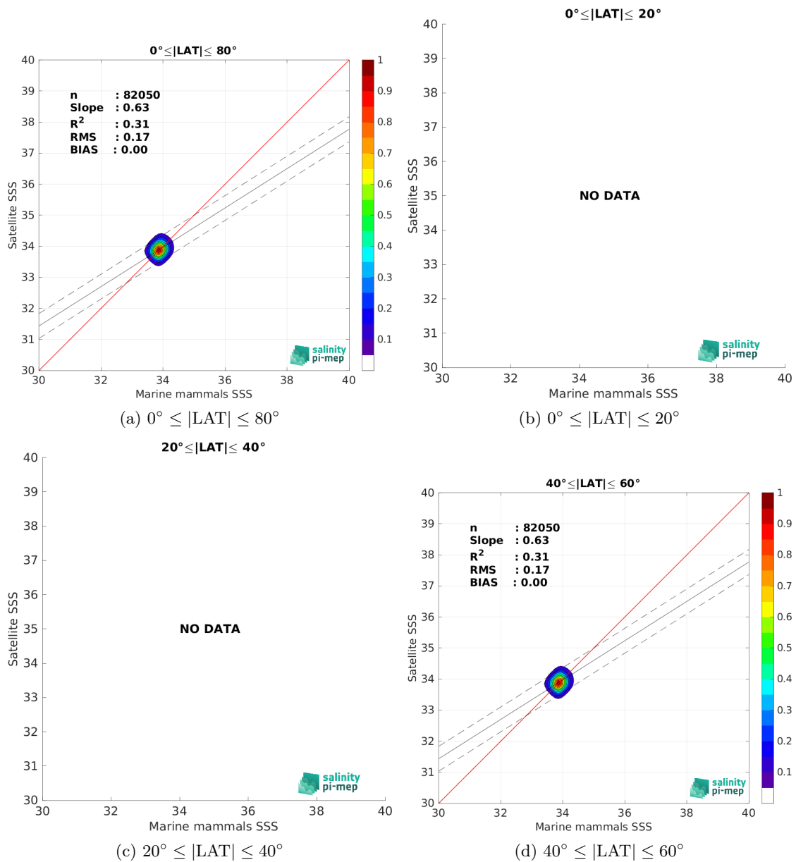
Figure 9: Contour maps of the concentration of CCI SSS L4 POLAR SH Merged-OI v4.4 - 7-day running (ESA) SSS (y-axis) versus Marine mammals SSS (x-axis) at match-up pairs for different latitude bands. For each plot, the red line shows x=y . The black thin and dashed lines indicate a linear fit through the data cloud and the \pm 95\% confidence levels, respectively. The number match-up pairs n , the slope and R^2 coefficient of the linear fit, the root mean square (RMS) and the mean bias between satellite and in situ data are indicated for each latitude band in each plots.
