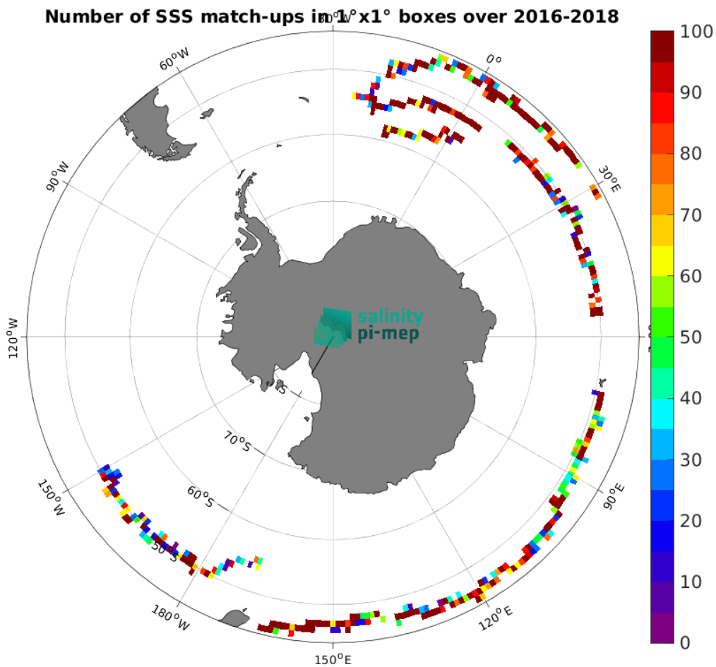
Figure 3: Number of SSS match-ups between Surface drifters SSS and the CCI SSS L4 POLAR SH Merged-OI v4.4 - 7-day running (ESA) SSS product for the Roaring Forties and Furious Fifties Pi-MEP region over 1^\circ \times 1^\circ boxes and for the full satellite product period.
