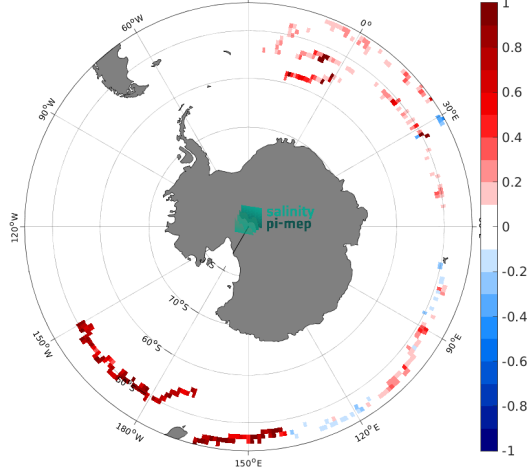
(e) MEAN( \Delta SSS) (Satellite - Surface drifters) 14
