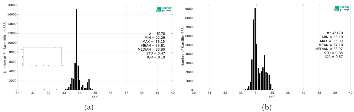
Figure 2: Histograms of SSS from Surface drifters (a) and CCI SSS L4 POLAR SH Merged-OI v4.4 - 7-day running (ESA) (b) considering all match-up pairs per bins of 0.1 over the Roaring Forties and Furious Fifties Pi-MEP region and for the full satellite product period.
