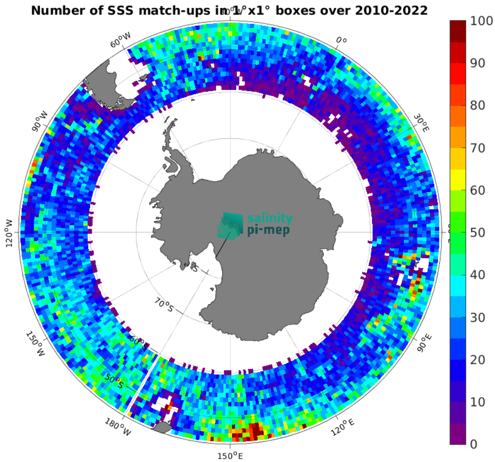
Figure 4: Number of SSS match-ups between Argo SSS and the CCI SSS L4 POLAR SH Merged-OI v4.4 - 7-day running (ESA) SSS product for the Roaring Forties and Furious Fifties Pi-MEP region over 1^\circ \times 1^\circ boxes and for the full satellite product period.
