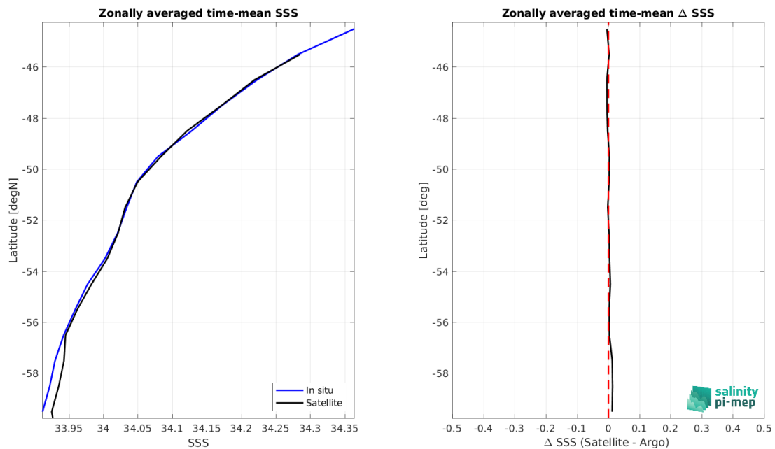
Figure 8: Left panel: Zonal mean SSS from CCI SSS L4 POLAR SH Merged-OI v4.4 - 7-day running (ESA) satellite product (black) and from Argo (blue). Right panel: Zonal mean of \Delta SSS (Satellite - Argo) for all the collected Pi-MEP match-up pairs estimated over the full satellite product period.
