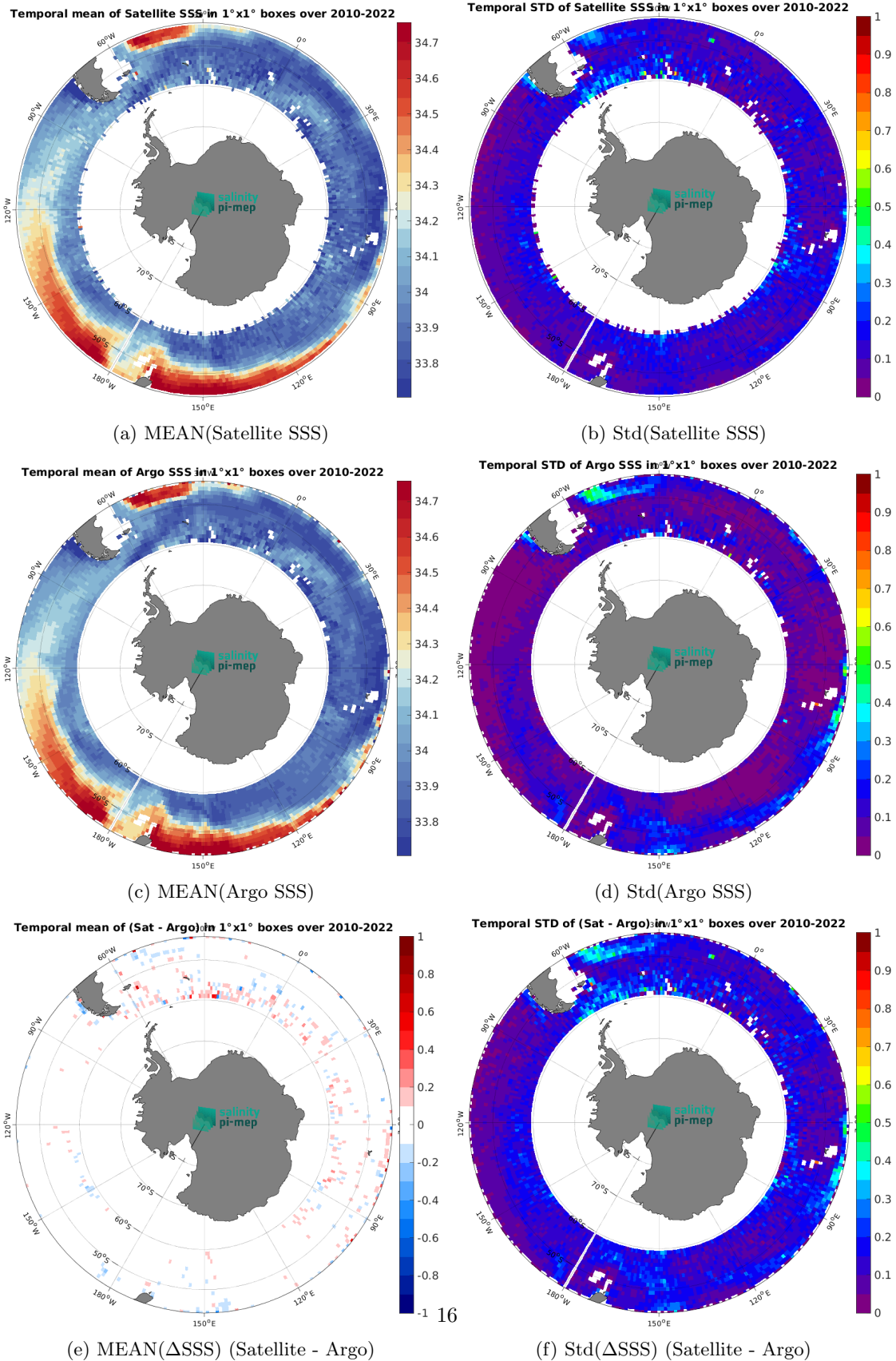
Figure 6: Temporal mean (left) and Std (right) of SSS from CCI SSS L4 POLAR SH Merged-OI v4.4 - 7-day running (ESA) (top), Argo (middle), and of \Delta SSS (Satellite - Argo). Only match-up pairs are used to generate these maps.
