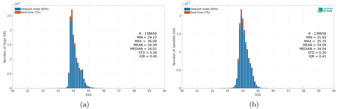
Figure 2: Histograms of SSS from Argo (a) and CCI SSS L4 POLAR SH Merged-OI v4.4 - 7-day running (ESA) (b) considering all match-up pairs per bins of 0.1 over the Roaring Forties and Furious Fifties Pi-MEP region and for the full satellite product period.
