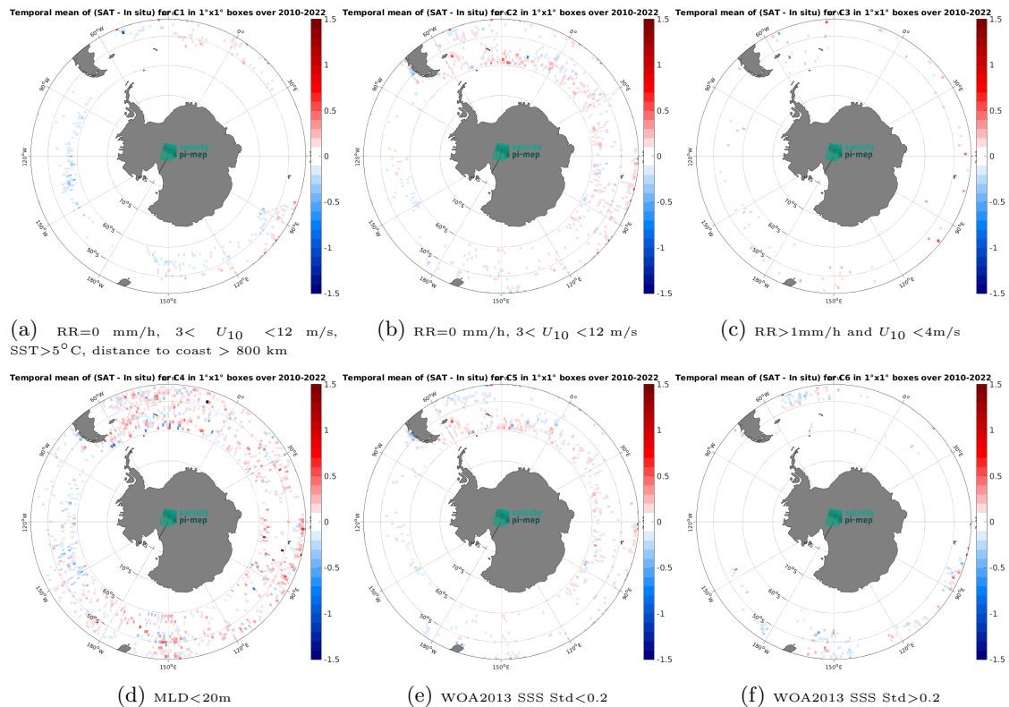
Figure 12: Temporal mean gridded over spatial boxes of size 1^{\circ}\times 1^{\circ} of \Delta\text{SSS} (CCI SSS L4 POLAR SH Merged-OI v4.4 - 7-day running (ESA) - Argo) for 6 different subdatasets corresponding to:RR=0 mm/h, 3 < U_{10} < 12 m/s, SST >5^{\circ}\text{C} , distance to coast > 800 km (a), RR=0 mm/h, 3 < U_{10} < 12 m/s (b), RR >1 mm/h and U_{10} < 4 m/s (c),MLD <20 m (d),WOA2013 SSS Std <0.2 (e),WOA2013 SSS Std >0.2 (f).
