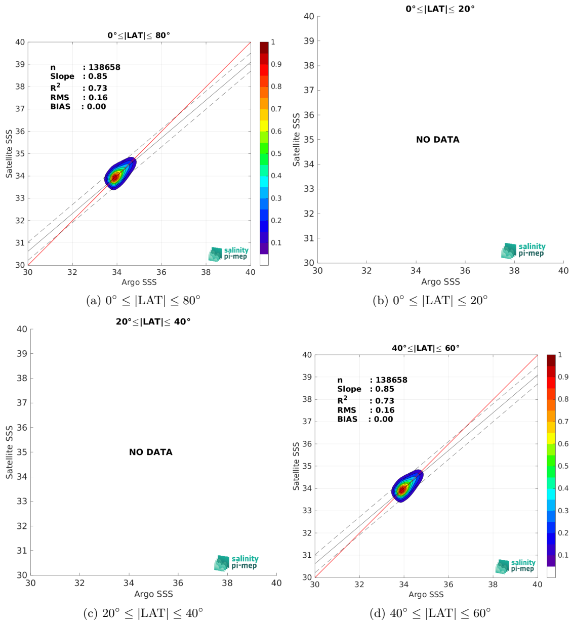
Figure 9: Contour maps of the concentration of CCI SSS L4 POLAR SH Merged-OI v4.4 - 7-day running (ESA) SSS (y-axis) versus Argo SSS (x-axis) at match-up pairs for different latitude bands. For each plot, the red line shows x=y . The black thin and dashed lines indicate a linear fit through the data cloud and the \pm 95\% confidence levels, respectively. The number match-up pairs n , the slope and R^2 coefficient of the linear fit, the root mean square (RMS) and the mean bias between satellite and in situ data are indicated for each latitude band in each plots.
