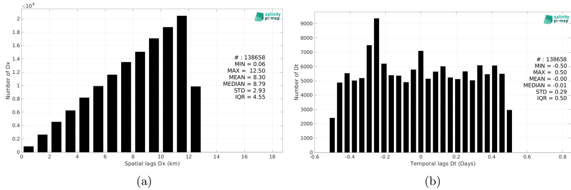
Figure 5: Histograms of the spatial (a) and temporal (b) lags between the location/time of the Argo measurement and the date of the corresponding CCI SSS L4 POLAR SH Merged-OI v4.4 - 7-day running (ESA) SSS pixel.
