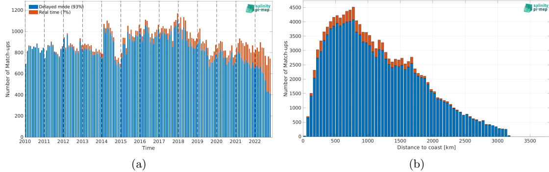
Figure 1: Number of match-ups between Argo and CCI SSS L4 POLAR SH Merged-OI v4.4 - 7-day running (ESA) SSS as a function of time (a) and as function of the distance to coast (b) over the Roaring Forties and Furious Fifties Pi-MEP region and for the full satellite product period.
