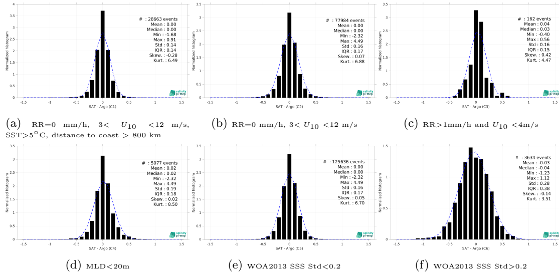
Figure 13: Normalized histogram of \Delta SSS (CCI SSS L4 POLAR SH Merged-OI v4.4 - 7-day running (ESA) - Argo) for 6 different subdatasets corresponding to: RR=0 mm/h, 3 < U_{10} < 12 m/s, SST>5°C, distance to coast > 800 km (a), RR=0 mm/h, 3 < U_{10} < 12 m/s (b), RR>1mm/h and U_{10} < 4 m/s (c), MLD<20m (d), WOA2013 SSS Std<0.2 (e), WOA2013 SSS Std>0.2 (f).
