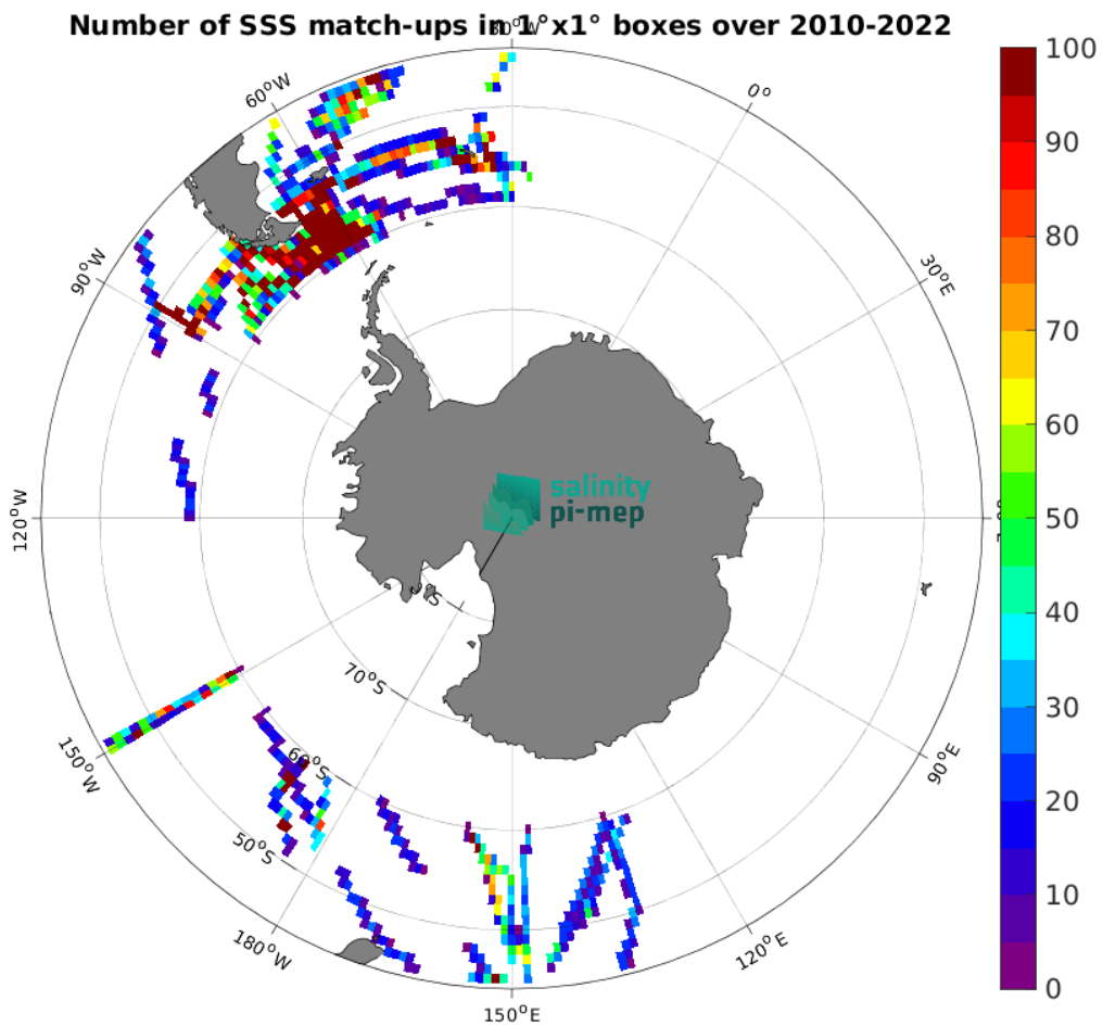
Figure 4: Number of SSS match-ups between TSG (SAMOS) SSS and the CCI SSS L4 POLAR SH Merged-OI v4.4 - 30-day running (ESA) SSS product for the Roaring Forties and Furious Fifties Pi-MEP region over 1^\circ \times 1^\circ boxes and for the full satellite product period.
