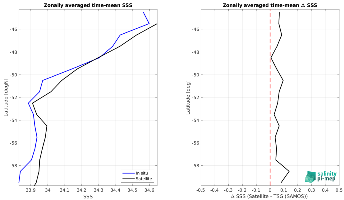
Figure 8: Left panel: Zonal mean SSS from CCI SSS L4 POLAR SH Merged-OI v4.4 - 30-day running (ESA) satellite product (black) and from TSG (SAMOS) (blue). Right panel: Zonal mean of \Delta SSS (Satellite - TSG (SAMOS)) for all the collected Pi-MEP match-up pairs estimated over the full satellite product period.
