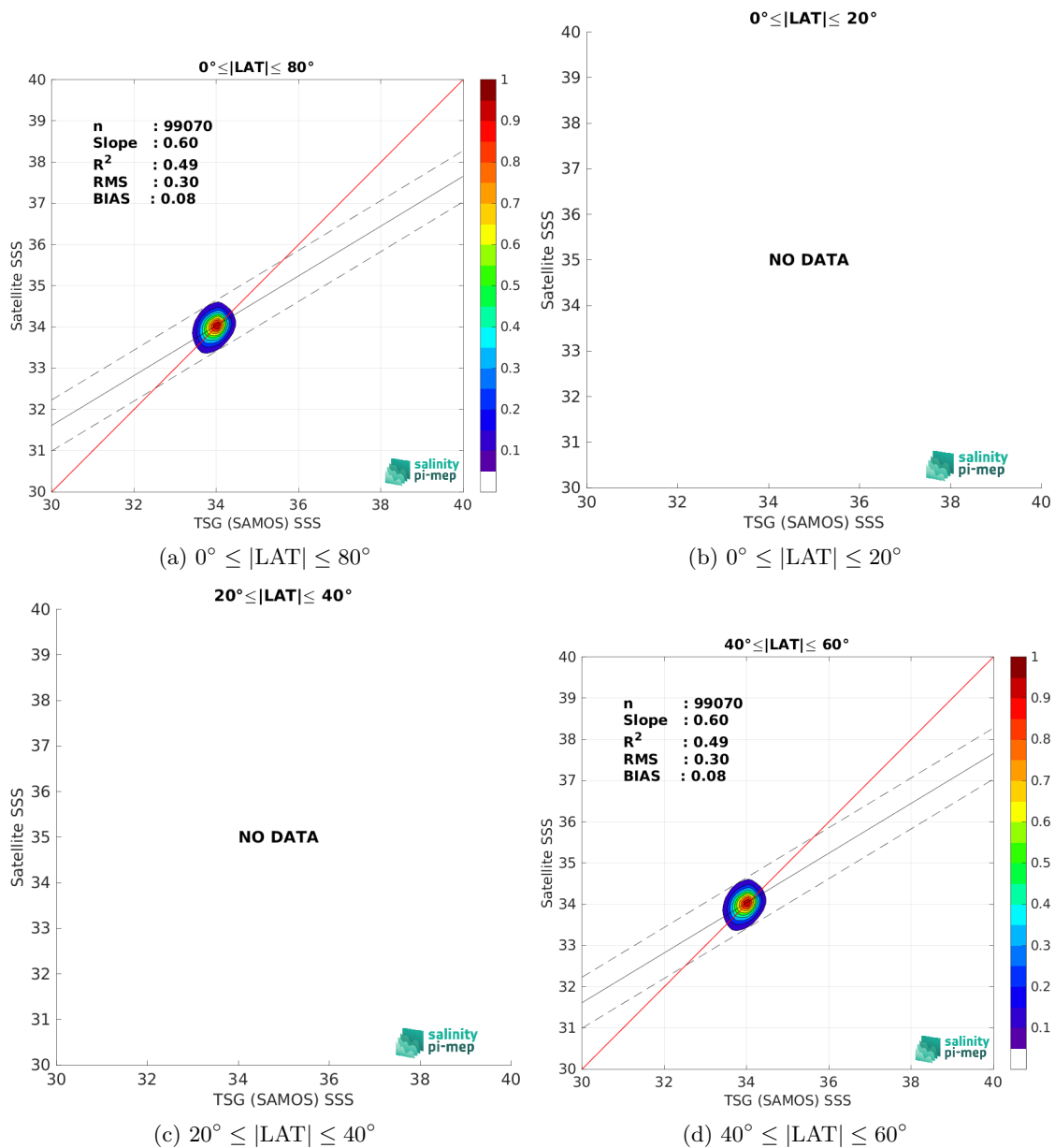
Figure 9: Contour maps of the concentration of CCI SSS L4 POLAR SH Merged-OI v4.4 - 30-day running (ESA) SSS (y-axis) versus TSG (SAMOS) SSS (x-axis) at match-up pairs for different latitude bands. For each plot, the red line shows x=y . The black thin and dashed lines indicate a linear fit through the data cloud and the \pm 95\% confidence levels, respectively. The number match-up pairs n , the slope and R^2 coefficient of the linear fit, the root mean square (RMS) and the mean bias between satellite and in situ data are indicated for each latitude band in each plots.
