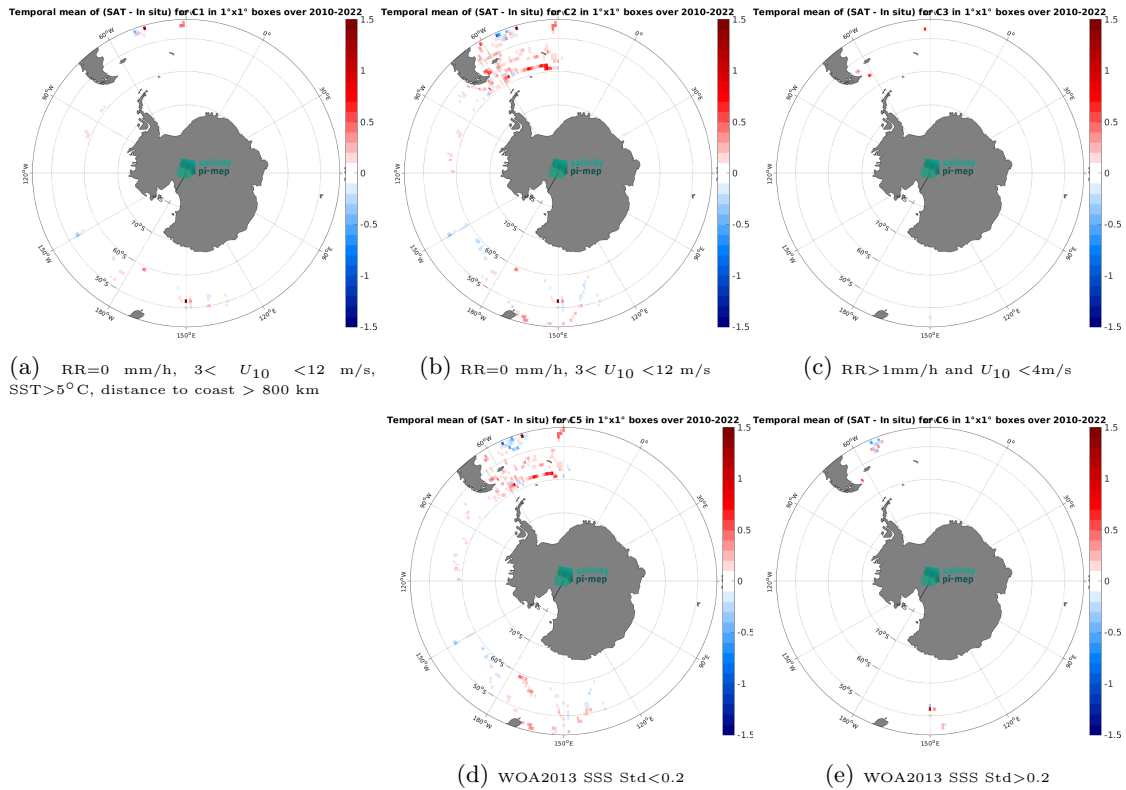
Figure 12: Temporal mean gridded over spatial boxes of size 1^{\circ}\times 1^{\circ} of \Delta\text{SSS} (CCI SSS L4 POLAR SH Merged-OI v4.4 - 30-day running (ESA) - TSG (SAMOS)) for 5 different subdatasets corresponding to: RR=0 mm/h, 3 < U_{10} < 12 m/s, SST > 5^{\circ}\text{C} , distance to coast > 800 km (a), RR=0 mm/h, 3 < U_{10} < 12 m/s (b), RR > 1 mm/h and U_{10} < 4 m/s (c), WOA2013 SSS Std < 0.2 (d), WOA2013 SSS Std > 0.2 (e).
