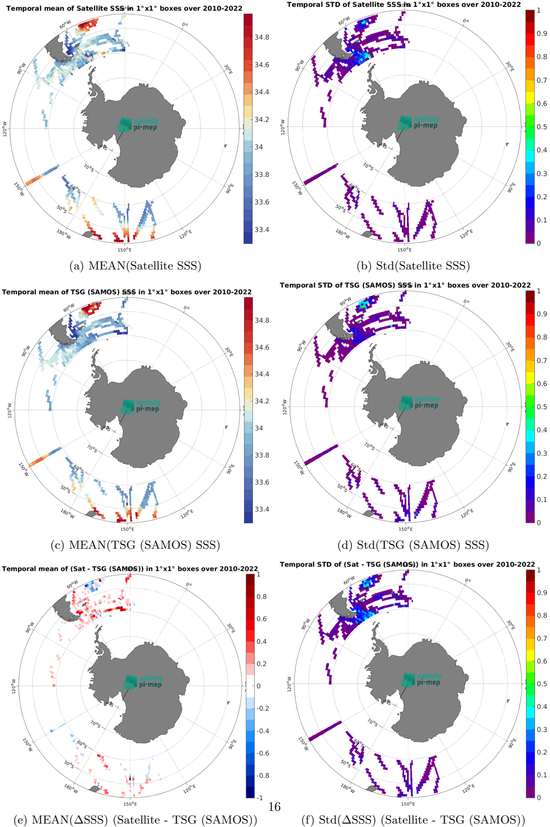
Figure 6: Temporal mean (left) and Std (right) of SSS from CCI SSS L4 POLAR SH Merged-OI v4.4 - 30-day running (ESA) (top), TSG (SAMOS) (middle), and of \Delta SSS (Satellite - TSG (SAMOS)). Only match-up pairs are used to generate these maps.
