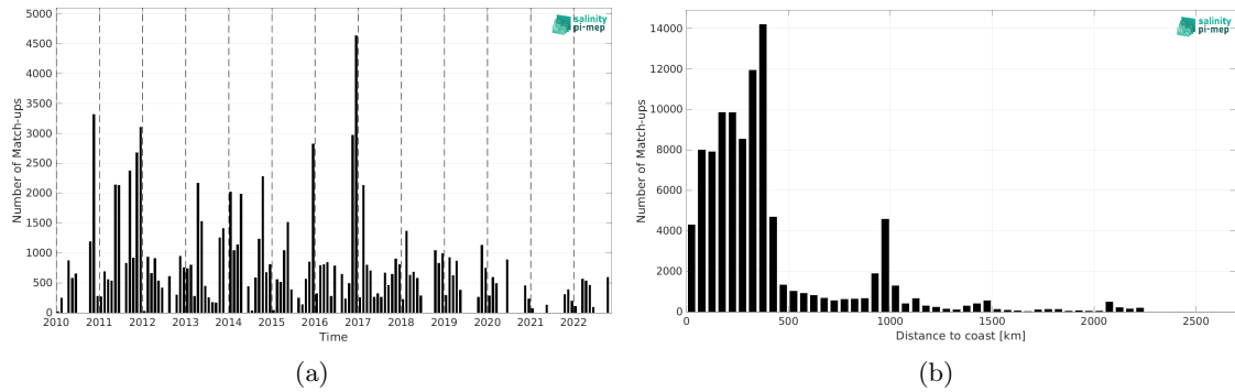
Figure 1: Number of match-ups between TSG (SAMOS) and CCI SSS L4 POLAR SH Merged-OI v4.4 - 30-day running (ESA) SSS as a function of time (a) and as function of the distance to coast (b) over the Roaring Forties and Furious Fifties Pi-MEP region and for the full satellite product period.
