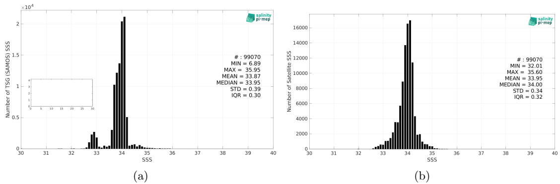
Figure 2: Histograms of SSS from TSG (SAMOS) (a) and CCI SSS L4 POLAR SH Merged-OI v4.4 - 30-day running (ESA) (b) considering all match-up pairs per bins of 0.1 over the Roaring Forties and Furious Fifties Pi-MEP region and for the full satellite product period.
