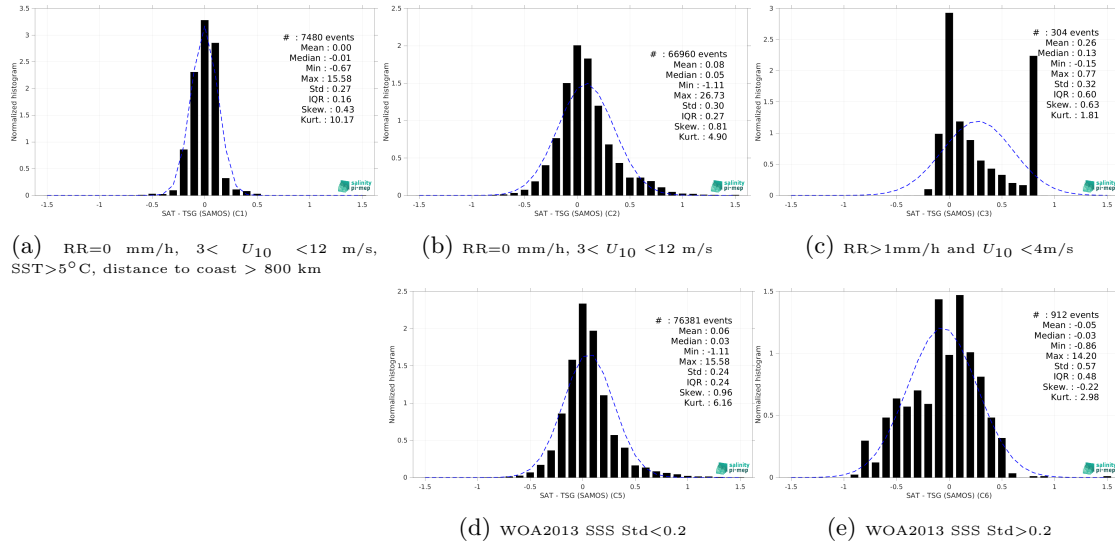
Figure 13: Normalized histogram of \Delta SSS (CCI SSS L4 POLAR SH Merged-OI v4.4 - 30-day running (ESA) - TSG (SAMOS)) for 5 different subdatasets corresponding to: RR=0 mm/h, 3 < U_{10} < 12 m/s, SST>5°C, distance to coast > 800 km (a), RR=0 mm/h, 3 < U_{10} < 12 m/s (b), RR>1mm/h and U_{10} < 4 m/s (c), WOA2013 SSS Std<0.2 (d), WOA2013 SSS Std>0.2 (e).
