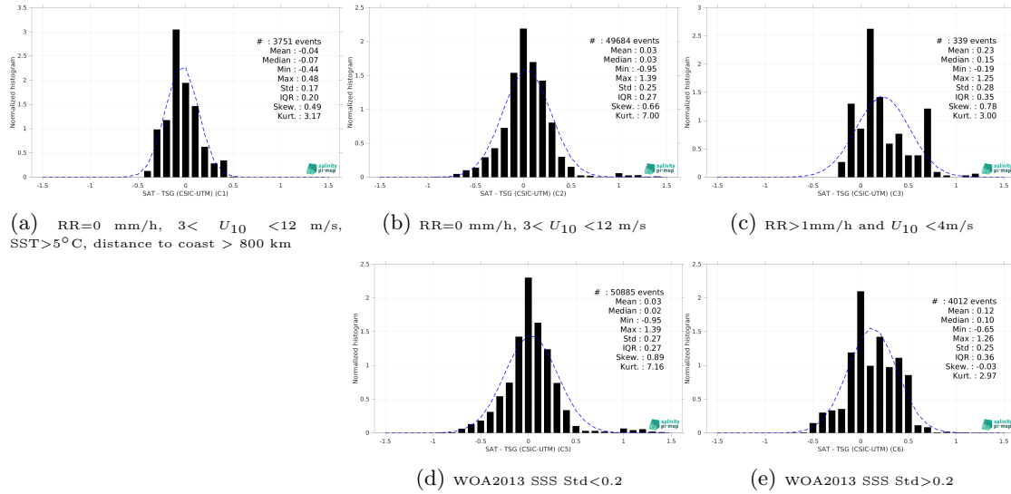
Figure 13: Normalized histogram of \Delta SSS (CCI SSS L4 POLAR SH Merged-OI v4.4 - 30-day running (ESA) - TSG (CSIC-UTM)) for 5 different subdatasets corresponding to: RR=0 mm/h, 3 < U_{10} < 12 m/s, SST >5^{\circ}\text{C} , distance to coast > 800 km (a), RR=0 mm/h, 3 < U_{10} < 12 m/s (b), RR >1 mm/h and U_{10} < 4 m/s (c), WOA2013 SSS Std <0.2 (d), WOA2013 SSS Std >0.2 (e).
