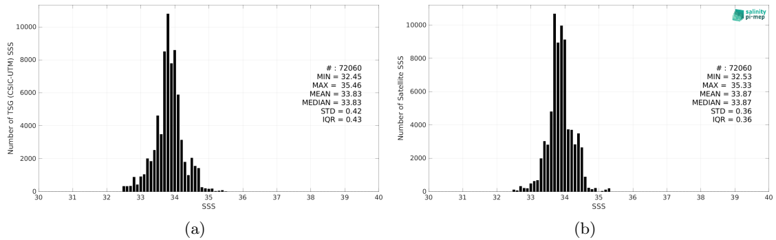
Figure 2: Histograms of SSS from TSG (CSIC-UTM) (a) and CCI SSS L4 POLAR SH Merged-OI v4.4 - 30-day running (ESA) (b) considering all match-up pairs per bins of 0.1 over the Roaring Forties and Furious Fifties Pi-MEP region and for the full satellite product period.
