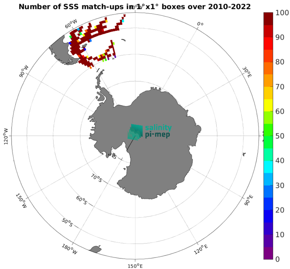
Figure 4: Number of SSS match-ups between TSG (CSIC-UTM) SSS and the CCI SSS L4 POLAR SH Merged-OI v4.4 - 30-day running (ESA) SSS product for the Roaring Forties and Furious Fifties Pi-MEP region over 1^\circ \times 1^\circ boxes and for the full satellite product period.
