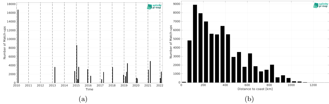
Figure 1: Number of match-ups between TSG (CSIC-UTM) and CCI SSS L4 POLAR SH Merged-OI v4.4 - 30-day running (ESA) SSS as a function of time (a) and as function of the distance to coast (b) over the Roaring Forties and Furious Fifties Pi-MEP region and for the full satellite product period.
