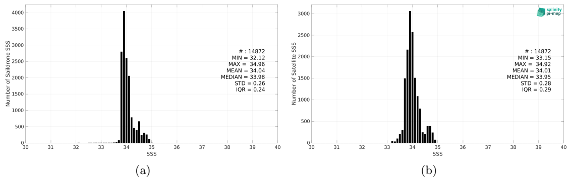
Figure 2: Histograms of SSS from Saildrone (a) and CCI SSS L4 POLAR SH Merged-OI v4.4 - 30-day running (ESA) (b) considering all match-up pairs per bins of 0.1 over the Roaring Forties and Furious Fifties Pi-MEP region and for the full satellite product period.
