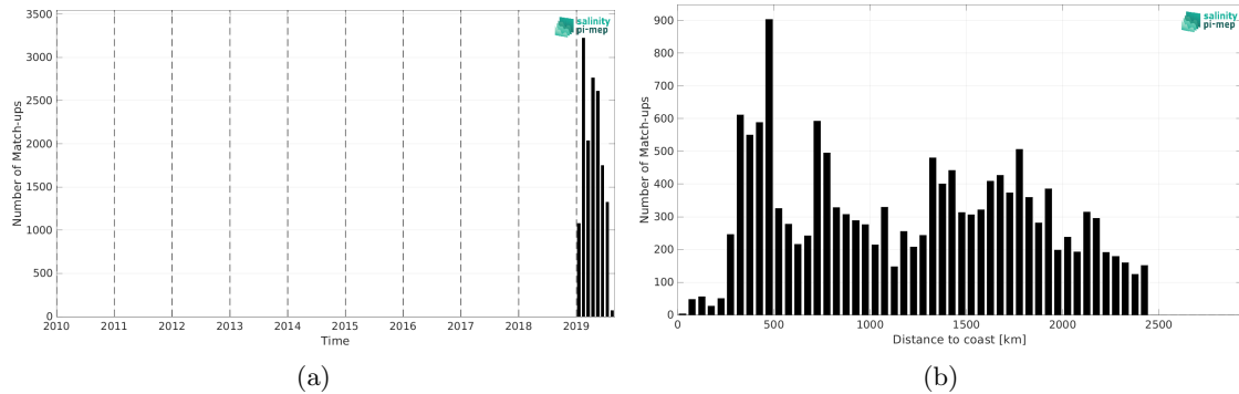
Figure 1: Number of match-ups between Saildrone and CCI SSS L4 POLAR SH Merged-OI v4.4 - 30-day running (ESA) SSS as a function of time (a) and as function of the distance to coast (b) over the Roaring Forties and Furious Fifties Pi-MEP region and for the full satellite product period.
