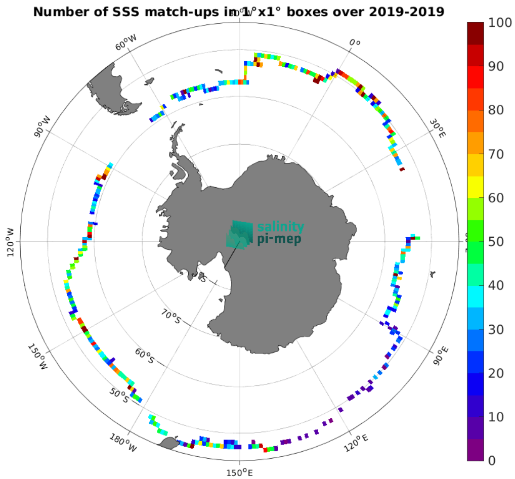
Figure 4: Number of SSS match-ups between Saildrone SSS and the CCI SSS L4 POLAR SH Merged-OI v4.4 - 30-day running (ESA) SSS product for the Roaring Forties and Furious Fifties Pi-MEP region over 1^{\circ} \times 1^{\circ} boxes and for the full satellite product period.
