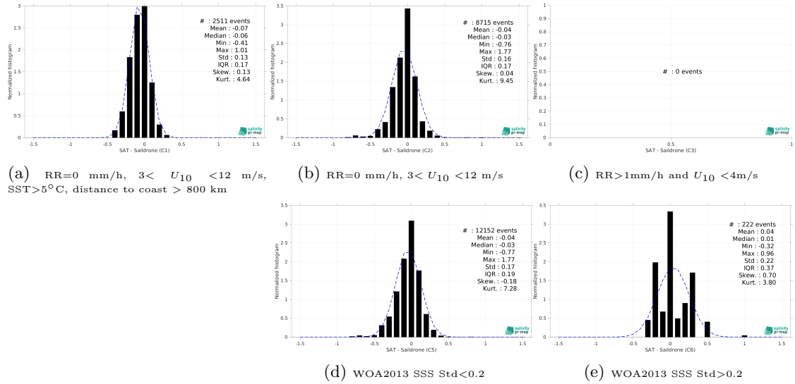
Figure 13: Normalized histogram of \Delta SSS (CCI SSS L4 POLAR SH Merged-OI v4.4 - 30-day running (ESA) - Saiddrone) for 5 different subdatasets corresponding to: RR=0 mm/h, 3 < U_{10} < 12 m/s, SST > 5°C, distance to coast > 800 km (a), RR=0 mm/h, 3 < U_{10} < 12 m/s (b), RR > 1mm/h and U_{10} < 4 m/s (c), WOA2013 SSS Std < 0.2 (d), WOA2013 SSS Std > 0.2 (e).
