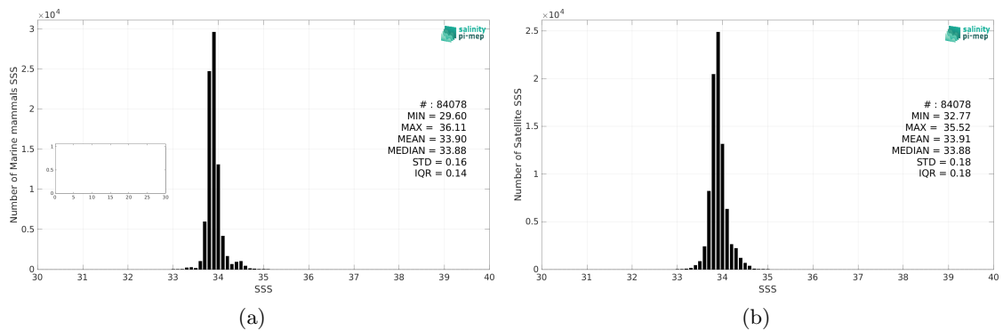
Figure 2: Histograms of SSS from Marine mammals (a) and CCI SSS L4 POLAR SH Merged-OI v4.4 - 30-day running (ESA) (b) considering all match-up pairs per bins of 0.1 over the Roaring Forties and Furious Fifties Pi-MEP region and for the full satellite product period.
