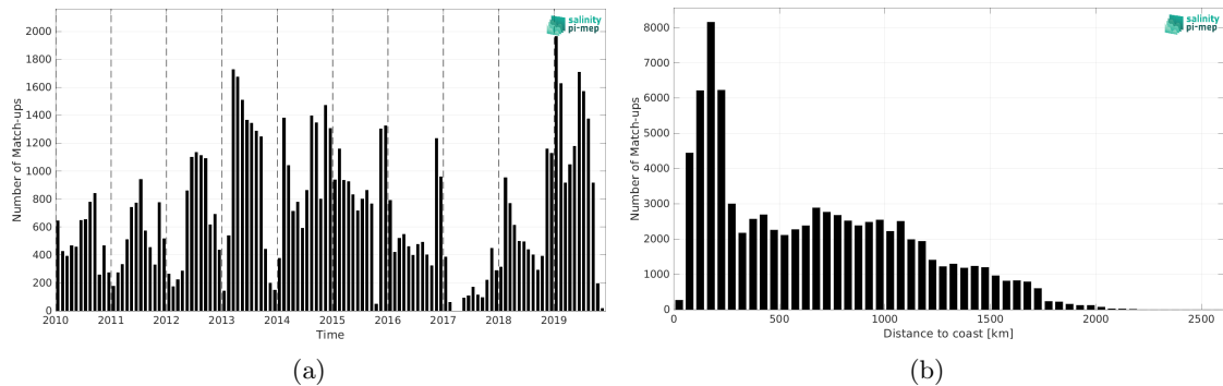
Figure 1: Number of match-ups between Marine mammals and CCI SSS L4 POLAR SH Merged-OI v4.4 - 30-day running (ESA) SSS as a function of time (a) and as function of the distance to coast (b) over the Roaring Forties and Furious Fifties Pi-MEP region and for the full satellite product period.
