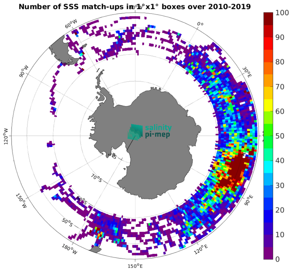
Figure 4: Number of SSS match-ups between Marine mammals SSS and the CCI SSS L4 POLAR SH Merged-OI v4.4 - 30-day running (ESA) SSS product for the Roaring Forties and Furious Fifties Pi-MEP region over 1^\circ \times 1^\circ boxes and for the full satellite product period.
