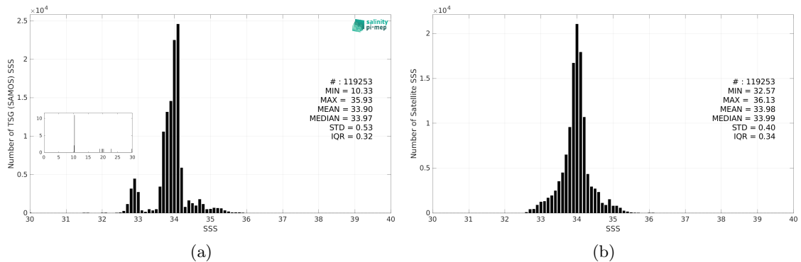
Figure 3: Histograms of SSS from TSG (SAMOS) (a) and CCI SSS L4 Merged-OI v5.5 - 7-day running (ESA) (b) considering all match-up pairs per bins of 0.1 over the Roaring Forties and Furious Fifties Pi-MEP region and for the full satellite product period.
