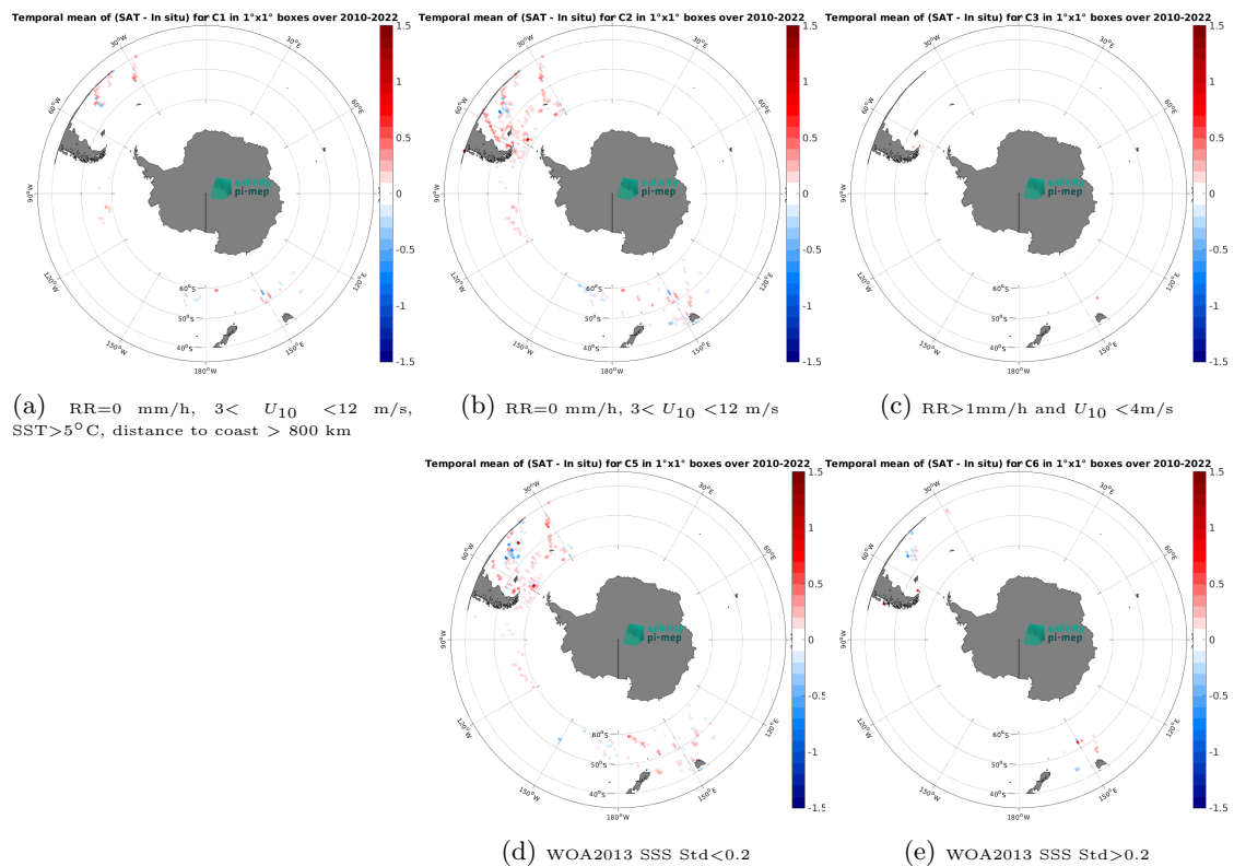
Figure 14: Temporal mean gridded over spatial boxes of size 1^\circ \times 1^\circ of \Delta\text{SSS} (CCI SSS L4 Merged-OI v5.5 - 7-day running (ESA) - TSG (SAMOS)) for 5 different subdatasets corresponding to: RR=0 mm/h, 3 < U_{10} < 12 m/s, SST > 5°C, distance to coast > 800 km (a), RR=0 mm/h, 3 < U_{10} < 12 m/s (b), RR > 1mm/h and U_{10} < 4 m/s (c), WOA2013 SSS Std < 0.2 (d), WOA2013 SSS Std > 0.2 (e).
