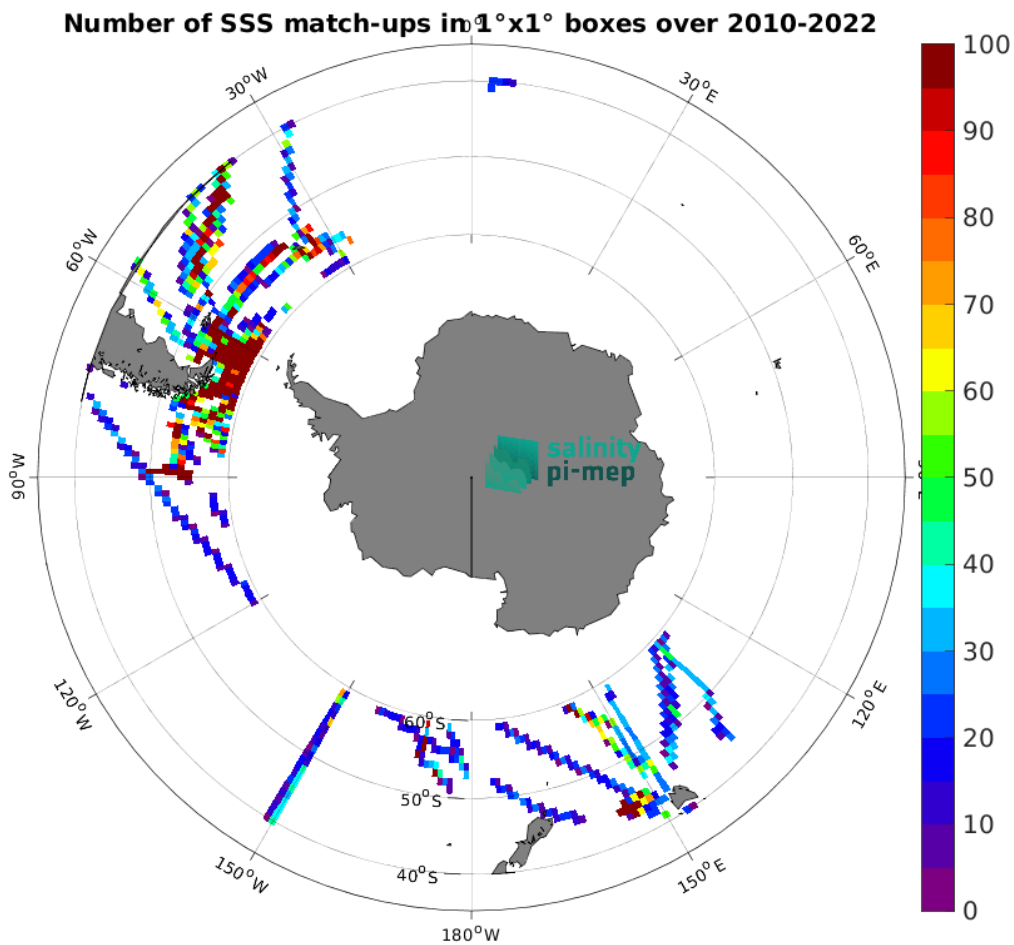
Figure 5: Number of SSS match-ups between TSG (SAMOS) SSS and the CCI SSS L4 Merged-OI v5.5 - 7-day running (ESA) SSS product for the Roaring Forties and Furious Fifties Pi-MEP region over 1^{\circ} \times 1^{\circ} boxes and for the full satellite product period.
