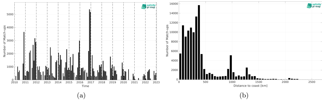
Figure 2: Number of match-ups between TSG (SAMOS) and CCI SSS L4 Merged-OI v5.5 - 7-day running (ESA) SSS as a function of time (a) and as function of the distance to coast (b) over the Roaring Forties and Furious Fifties Pi-MEP region and for the full satellite product period.
