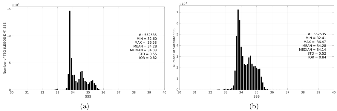
Figure 3: Histograms of SSS from TSG (LEGOS-DM) (a) and CCI SSS L4 Merged-OI v5.5 - 7-day running (ESA) (b) considering all match-up pairs per bins of 0.1 over the Roaring Forties and Furious Fifties Pi-MEP region and for the full satellite product period.
