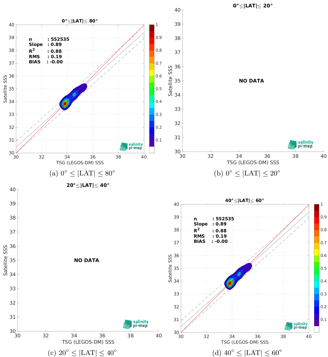
Figure 10: Contour maps of the concentration of CCI SSS L4 Merged-OI v5.5 - 7-day running (ESA) SSS (y-axis) versus TSG (LEGOS-DM) SSS (x-axis) at match-up pairs for different latitude bands. For each plot, the red line shows x=y . The black thin and dashed lines indicate a linear fit through the data cloud and the \pm 95\% confidence levels, respectively. The number of match-up pairs n , the slope and R^2 coefficient of the linear fit, the root mean square (RMS) and the mean bias between satellite and in situ data are indicated for each latitude band in each plot.
