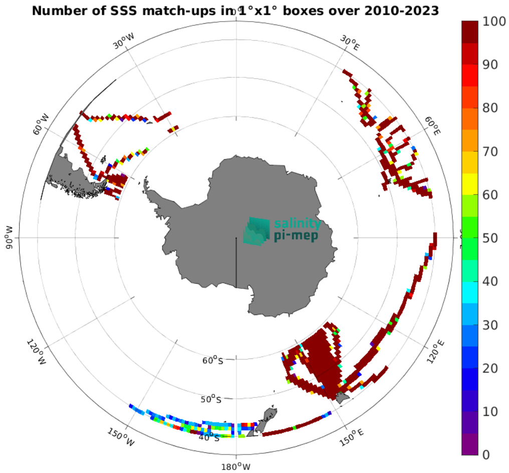
Figure 5: Number of SSS match-ups between TSG (LEGOS-DM) SSS and the CCI SSS L4 Merged-OI v5.5 - 7-day running (ESA) SSS product for the Roaring Forties and Furious Fifties Pi-MEP region over 1^\circ \times 1^\circ boxes and for the full satellite product period.
