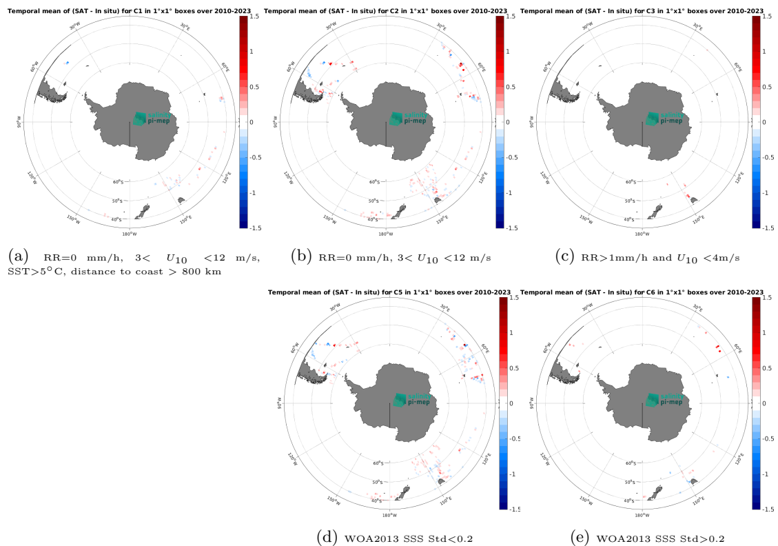
Figure 14: Temporal mean gridded over spatial boxes of size 1^\circ \times 1^\circ of \Delta\text{SSS} (CCI SSS L4 Merged-OI v5.5 - 7-day running (ESA) - TSG (LEGOS-DM)) for 5 different subdatasets corresponding to:RR=0 mm/h, 3 < U_{10} < 12 m/s, SST>5°C, distance to coast > 800 km (a), RR=0 mm/h, 3 < U_{10} < 12 m/s (b), RR>1mm/h and U_{10} < 4 m/s (c), WOA2013 SSS Std<0.2 (d), WOA2013 SSS Std>0.2 (e).
