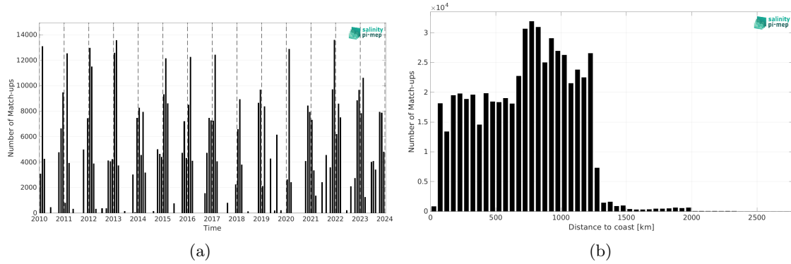
Figure 2: Number of match-ups between TSG (LEGOS-DM) and CCI SSS L4 Merged-OI v5.5 - 7-day running (ESA) SSS as a function of time (a) and as function of the distance to coast (b) over the Roaring Forties and Furious Fifties Pi-MEP region and for the full satellite product period.
