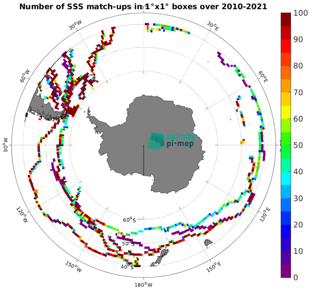
Figure 5: Number of SSS match-ups between TSG (GOSUD-Sailing-ship) SSS and the CCI SSS L4 Merged-OI v5.5 - 7-day running (ESA) SSS product for the Roaring Forties and Furious Fifties Pi-MEP region over 1^\circ \times 1^\circ boxes and for the full satellite product period.
