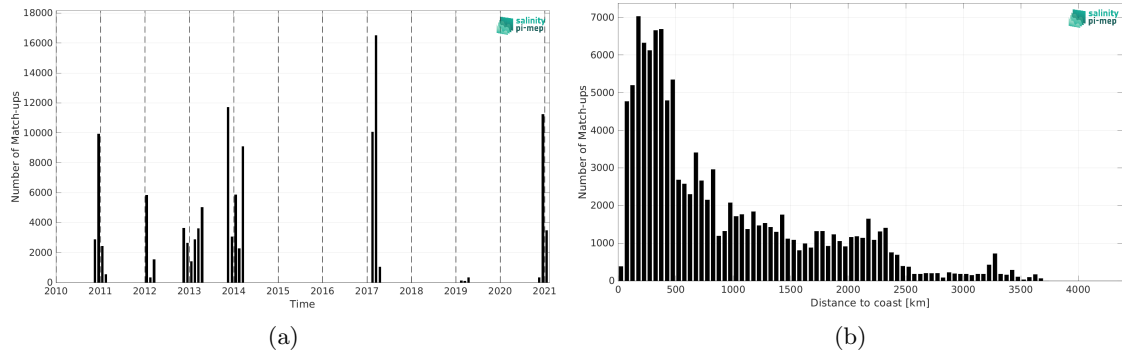
Figure 2: Number of match-ups between TSG (GOSUD-Sailing-ship) and CCI SSS L4 Merged-OI v5.5 - 7-day running (ESA) SSS as a function of time (a) and as function of the distance to coast (b) over the Roaring Forties and Furious Fifties Pi-MEP region and for the full satellite product period.
