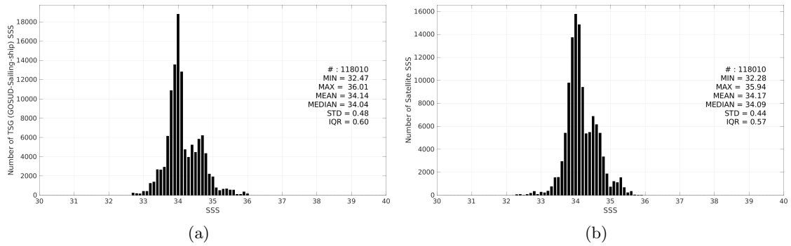
Figure 3: Histograms of SSS from TSG (GOSUD-Sailing-ship) (a) and CCI SSS L4 Merged-OI v5.5 - 7-day running (ESA) (b) considering all match-up pairs per bins of 0.1 over the Roaring Forties and Furious Fifties Pi-MEP region and for the full satellite product period.
