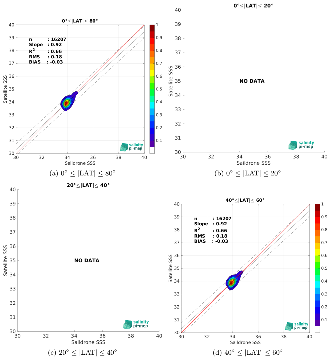
Figure 10: Contour maps of the concentration of CCI SSS L4 Merged-OI v5.5 - 7-day running (ESA) SSS (y-axis) versus Saildrone SSS (x-axis) at match-up pairs for different latitude bands. For each plot, the red line shows x=y . The black thin and dashed lines indicate a linear fit through the data cloud and the \pm 95\% confidence levels, respectively. The number match-up pairs n , the slope and R^2 coefficient of the linear fit, the root mean square (RMS) and the mean bias between satellite and in situ data are indicated for each latitude band in each plots.
