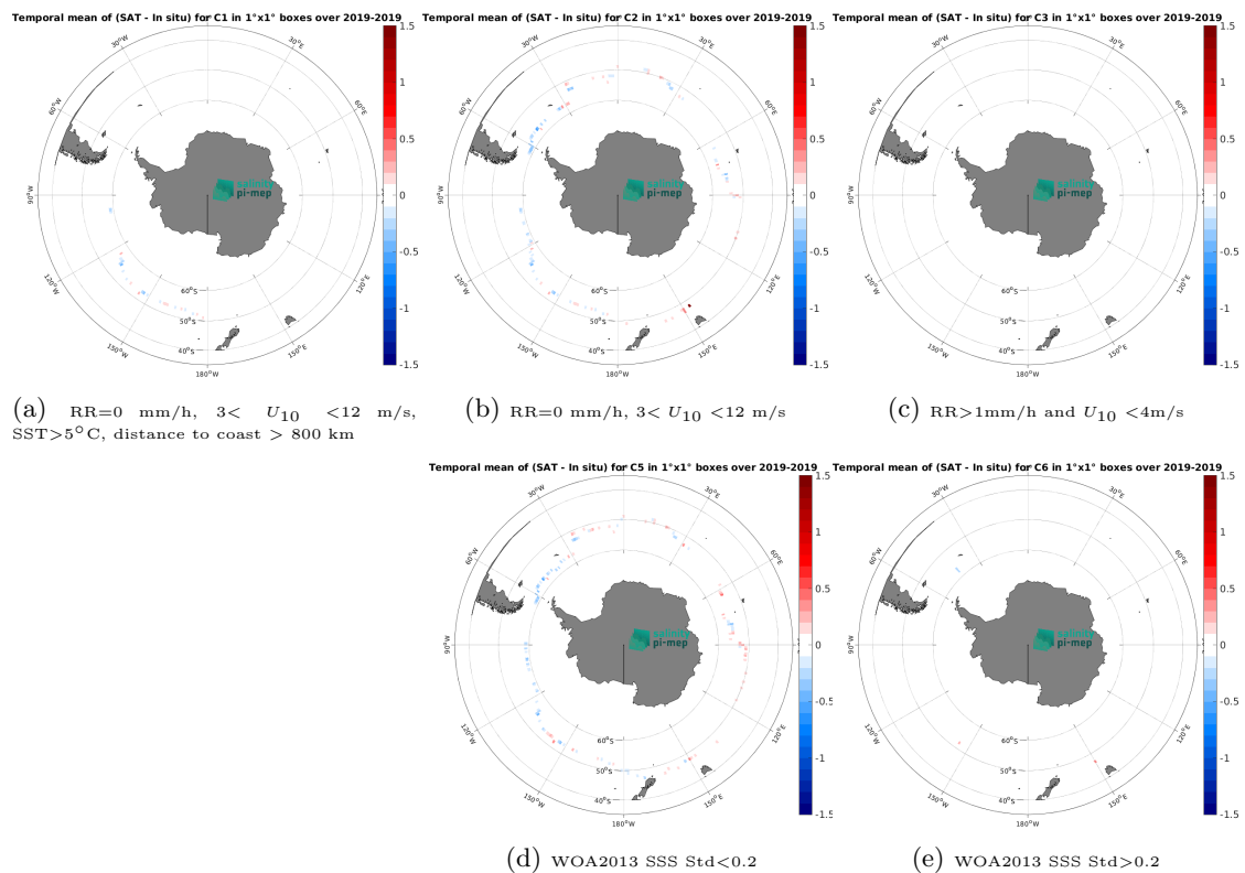
Figure 14: Temporal mean gridded over spatial boxes of size 1^\circ \times 1^\circ of \Delta SSS (CCI SSS L4 Merged-OI v5.5 - 7-day running (ESA) - Saildrone) for 5 different subdatasets corresponding to:RR=0 mm/h, 3 < U_{10} < 12 m/s, SST > 5^\circ\text{C} , distance to coast > 800 km (a), RR=0 mm/h, 3 < U_{10} < 12 m/s (b), RR > 1 mm/h and U_{10} < 4 m/s (c), WOA2013 SSS Std < 0.2 (d), WOA2013 SSS Std > 0.2 (e).
