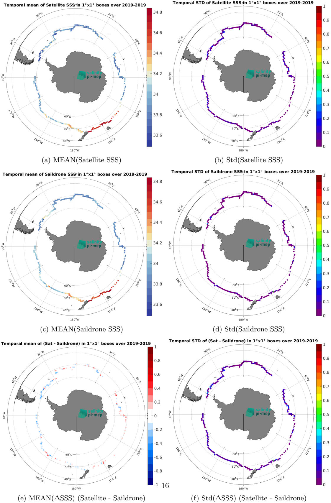
Figure 7: Temporal mean (left) and Std (right) of SSS from CCI SSS L4 Merged-OI v5.5 - 7-day running (ESA) (top), Saildrone (middle), and of \Delta SSS (Satellite - Saildrone). Only match-up pairs are used to generate these maps.
