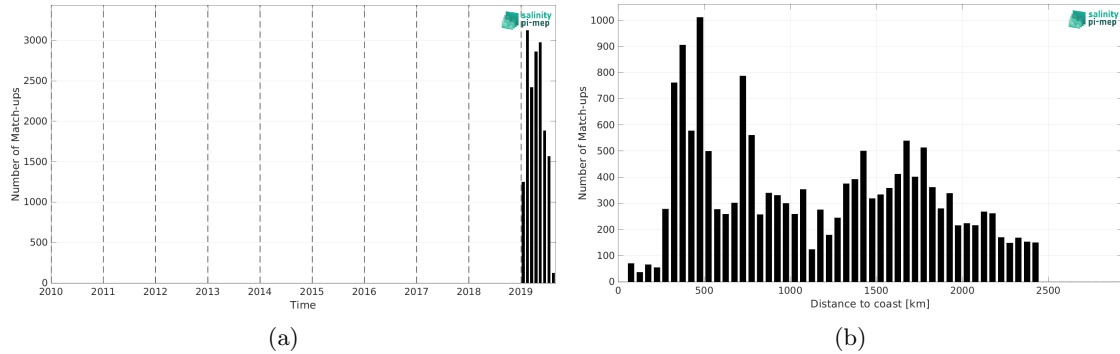
Figure 2: Number of match-ups between Saildrone and CCI SSS L4 Merged-OI v5.5 - 7-day running (ESA) SSS as a function of time (a) and as function of the distance to coast (b) over the Roaring Forties and Furious Fifties Pi-MEP region and for the full satellite product period.
