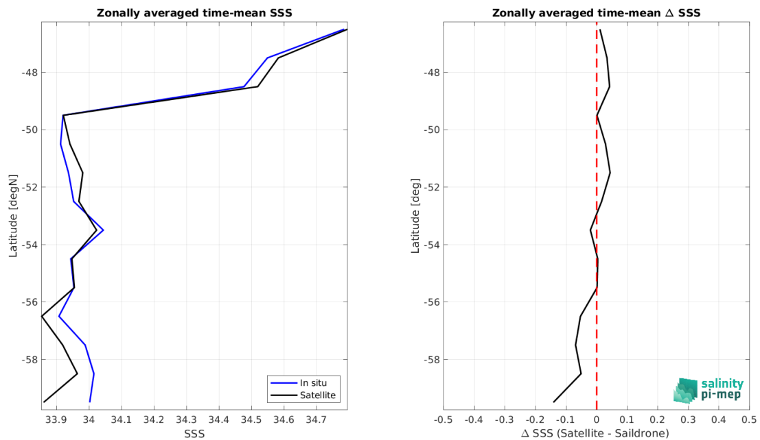
Figure 9: Left panel: Zonal mean SSS from CCI SSS L4 Merged-OI v5.5 - 7-day running (ESA) satellite product (black) and from Sairdron (blue). Right panel: Zonal mean of \Delta SSS (Satellite - Sairdron) for all the collected Pi-MEP match-up pairs estimated over the full satellite product period.
