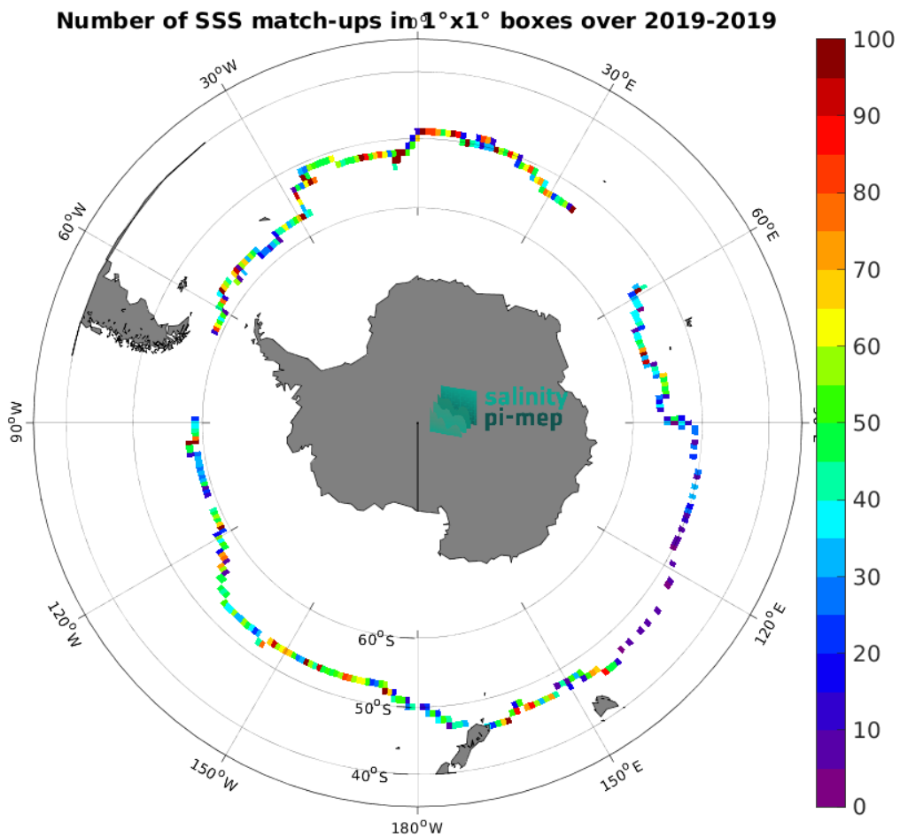
Figure 5: Number of SSS match-ups between Saildrone SSS and the CCI SSS L4 Merged-OI v5.5 - 7-day running (ESA) SSS product for the Roaring Forties and Furious Fifties Pi-MEP region over 1^\circ \times 1^\circ boxes and for the full satellite product period.
