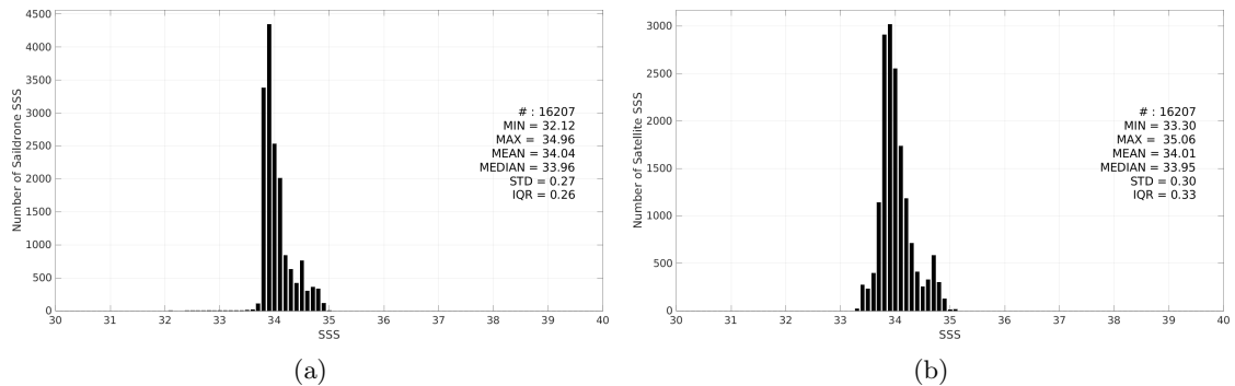
Figure 3: Histograms of SSS from Saildrone (a) and CCI SSS L4 Merged-OI v5.5 - 7-day running (ESA) (b) considering all match-up pairs per bins of 0.1 over the Roaring Forties and Furious Fifties Pi-MEP region and for the full satellite product period.
