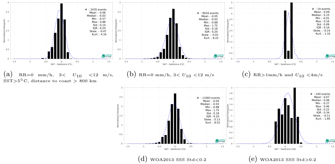
Figure 15: Normalized histogram of \Delta SSS (CCI SSS L4 Merged-OI v5.5 - 7-day running (ESA) - Saildrone) for 5 different subdatasets corresponding to: RR=0 mm/h, 3 < U_{10} < 12 m/s, SST > 5°C, distance to coast > 800 km (a), RR=0 mm/h, 3 < U_{10} < 12 m/s (b), RR > 1mm/h and U_{10} < 4 m/s (c), WOA2013 SSS Std < 0.2 (d), WOA2013 SSS Std > 0.2 (e).
