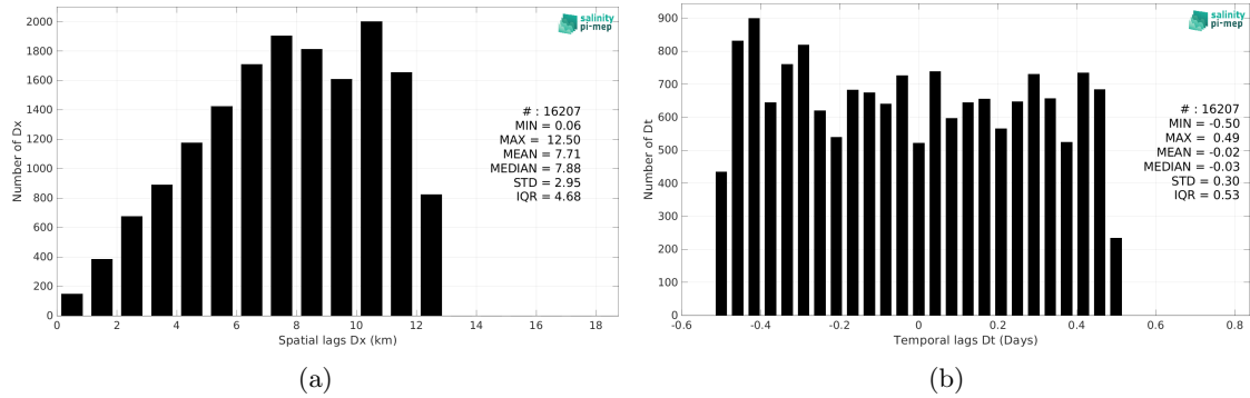
Figure 6: Histograms of the spatial (a) and temporal (b) lags between the location/time of the Saildrone measurement and the date of the corresponding CCI SSS L4 Merged-OI v5.5 - 7-day running (ESA) SSS pixel.
