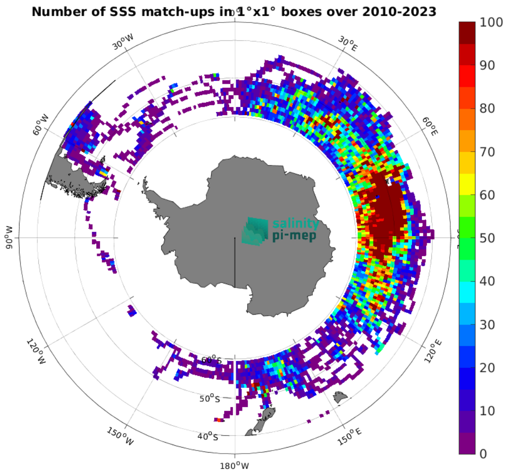
Figure 5: Number of SSS match-ups between Marine mammals SSS and the CCI SSS L4 Merged-OI v5.5 - 7-day running (ESA) SSS product for the Roaring Forties and Furious Fifties Pi-MEP region over 1^\circ \times 1^\circ boxes and for the full satellite product period.
