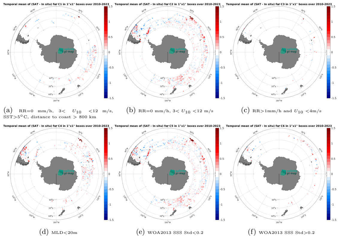
Figure 14: Temporal mean gridded over spatial boxes of size 1^\circ \times 1^\circ of \Delta SSS (CCI SSS L4 Merged-OI v5.5 - 7-day running (ESA) - Marine mammals) for 6 different subdatasets corresponding to:RR=0 mm/h, 3 < U_{10} < 12 m/s, SST >5^\circ C, distance to coast > 800 km (a), RR=0 mm/h, 3 < U_{10} < 12 m/s (b), RR >1 mm/h and U_{10} < 4 m/s (c),MLD <20 m (d),WOA2013 SSS Std <0.2 (e),WOA2013 SSS Std >0.2 (f).
