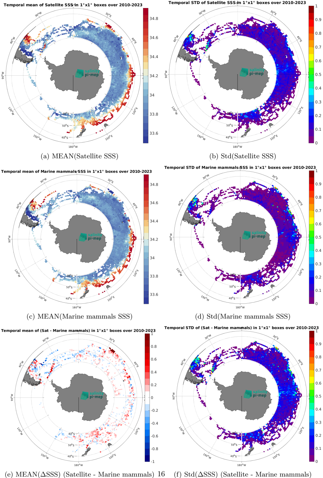
Figure 7: Temporal mean (left) and Std (right) of SSS from CCI SSS L4 Merged-OI v5.5 - 7-day running (ESA) (top), Marine mammals (middle), and of \Delta SSS (Satellite - Marine mammals). Only match-up pairs are used to generate these maps.
