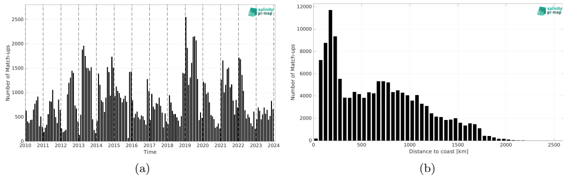
Figure 2: Number of match-ups between Marine mammals and CCI SSS L4 Merged-OI v5.5 - 7-day running (ESA) SSS as a function of time (a) and as function of the distance to coast (b) over the Roaring Forties and Furious Fifties Pi-MEP region and for the full satellite product period.
