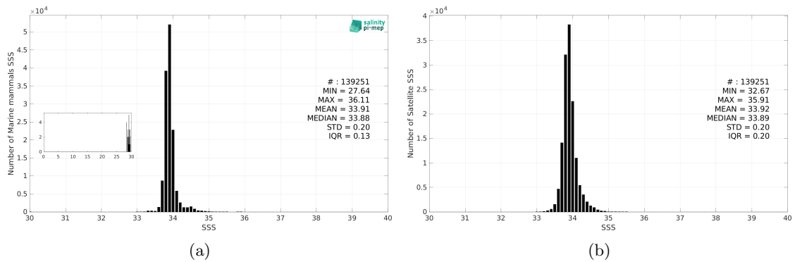
Figure 3: Histograms of SSS from Marine mammals (a) and CCI SSS L4 Merged-OI v5.5 - 7-day running (ESA) (b) considering all match-up pairs per bins of 0.1 over the Roaring Forties and Furious Fifties Pi-MEP region and for the full satellite product period.
