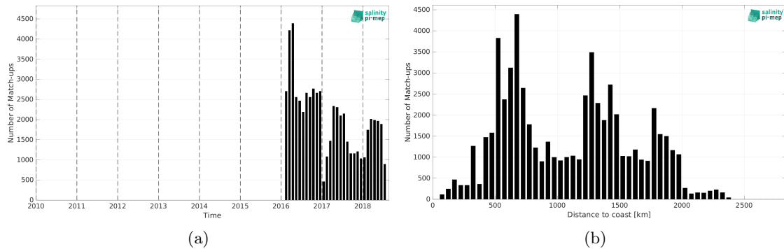
Figure 2: Number of match-ups between Surface drifters and CCI SSS L4 Merged-OI v5.5 - 7-day running (ESA) SSS as a function of time (a) and as function of the distance to coast (b) over the Roaring Forties and Furious Fifties Pi-MEP region and for the full satellite product period.
