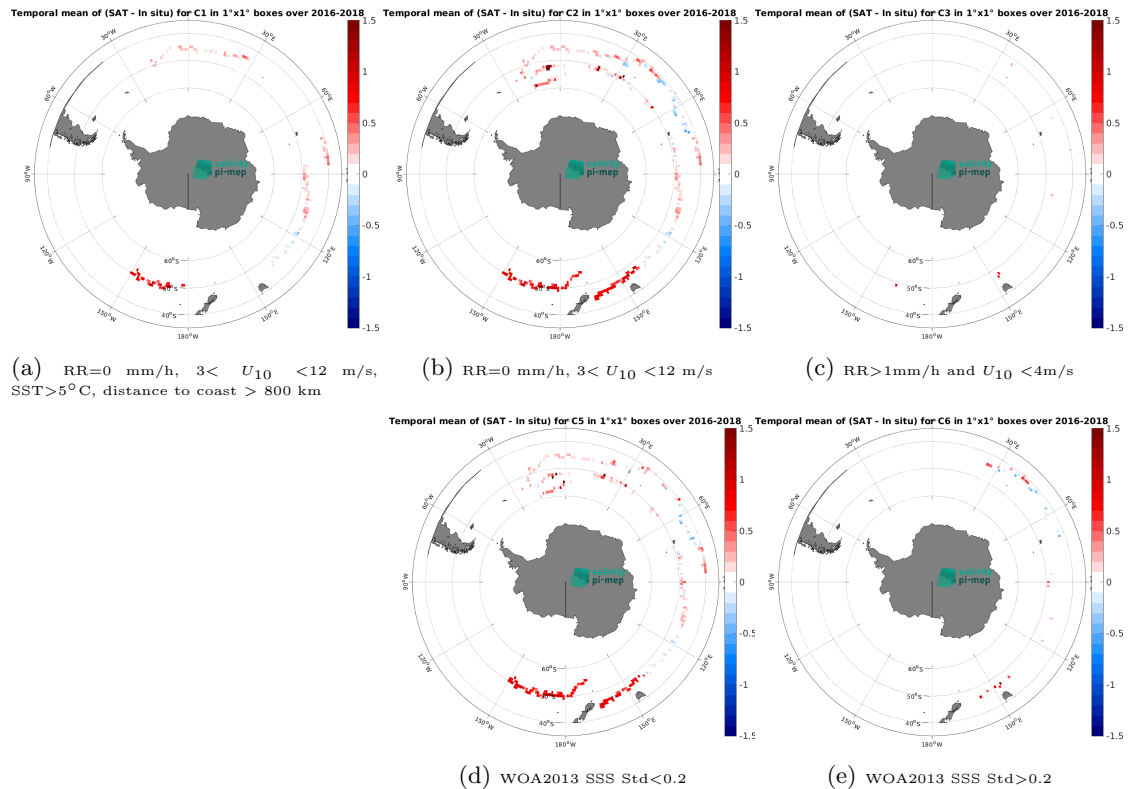
Figure 13: Temporal mean gridded over spatial boxes of size 1^\circ \times 1^\circ of \Delta SSS (CCI SSS L4 Merged-OI v5.5 - 7-day running (ESA) - Surface drifters) for 5 different subdatasets corresponding to:RR=0 mm/h, 3 < U_{10} < 12 m/s, SST >5^\circ C, distance to coast > 800 km (a), RR=0 mm/h, 3 < U_{10} < 12 m/s (b), RR >1 mm/h and U_{10} < 4 m/s (c), WOA2013 SSS Std <0.2 (d), WOA2013 SSS Std >0.2 (e).
