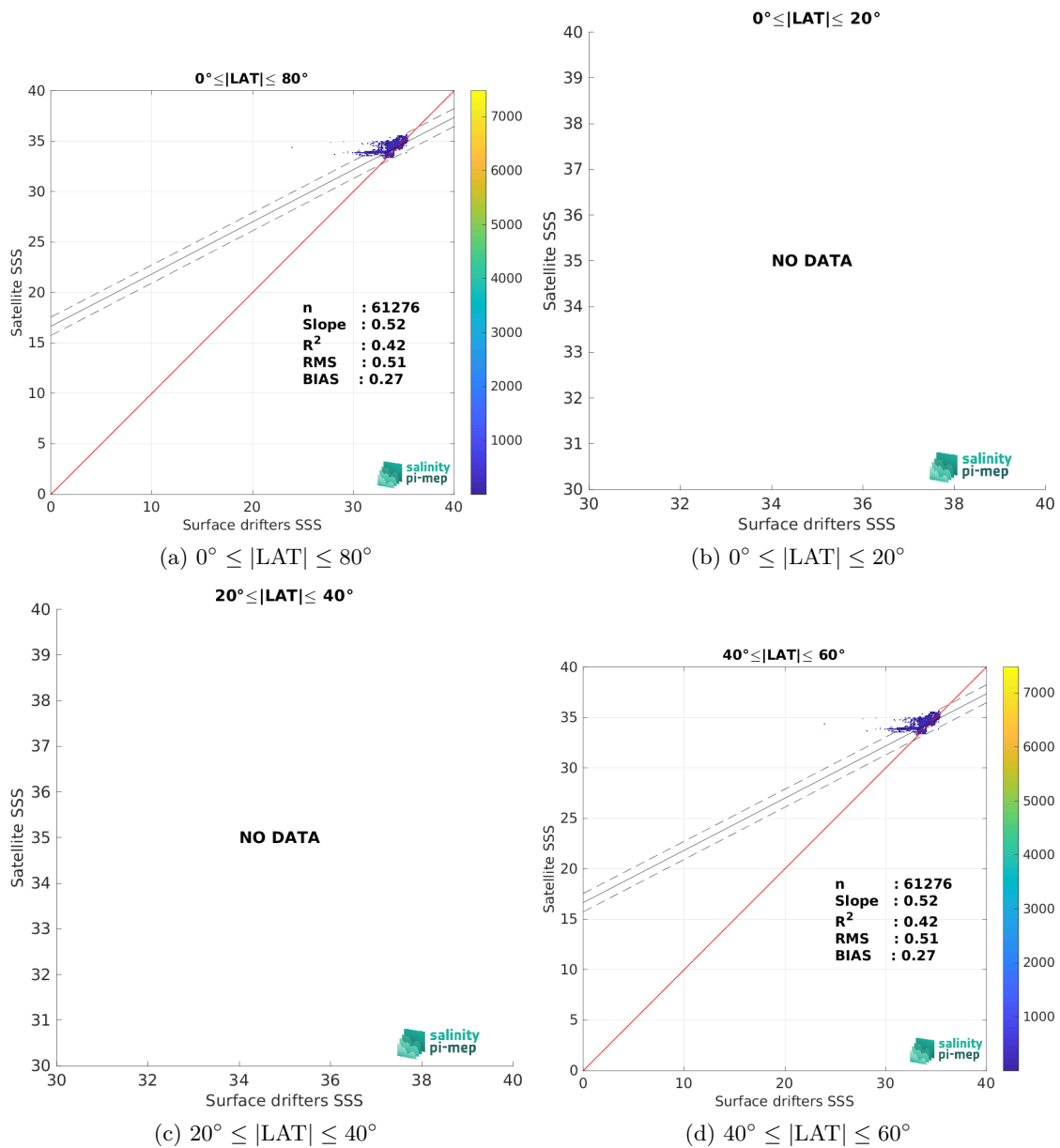
Figure 9: Contour maps of the concentration of CCI SSS L4 Merged-OI v5.5 - 7-day running (ESA) SSS (y-axis) versus Surface drifters SSS (x-axis) at match-up pairs for different latitude bands. For each plot, the red line shows x=y . The black thin and dashed lines indicate a linear fit through the data cloud and the \pm 95\% confidence levels, respectively. The number match-up pairs n , the slope and R^2 coefficient of the linear fit, the root mean square (RMS) and the mean bias between satellite and in situ data are indicated for each latitude band in each plots.
