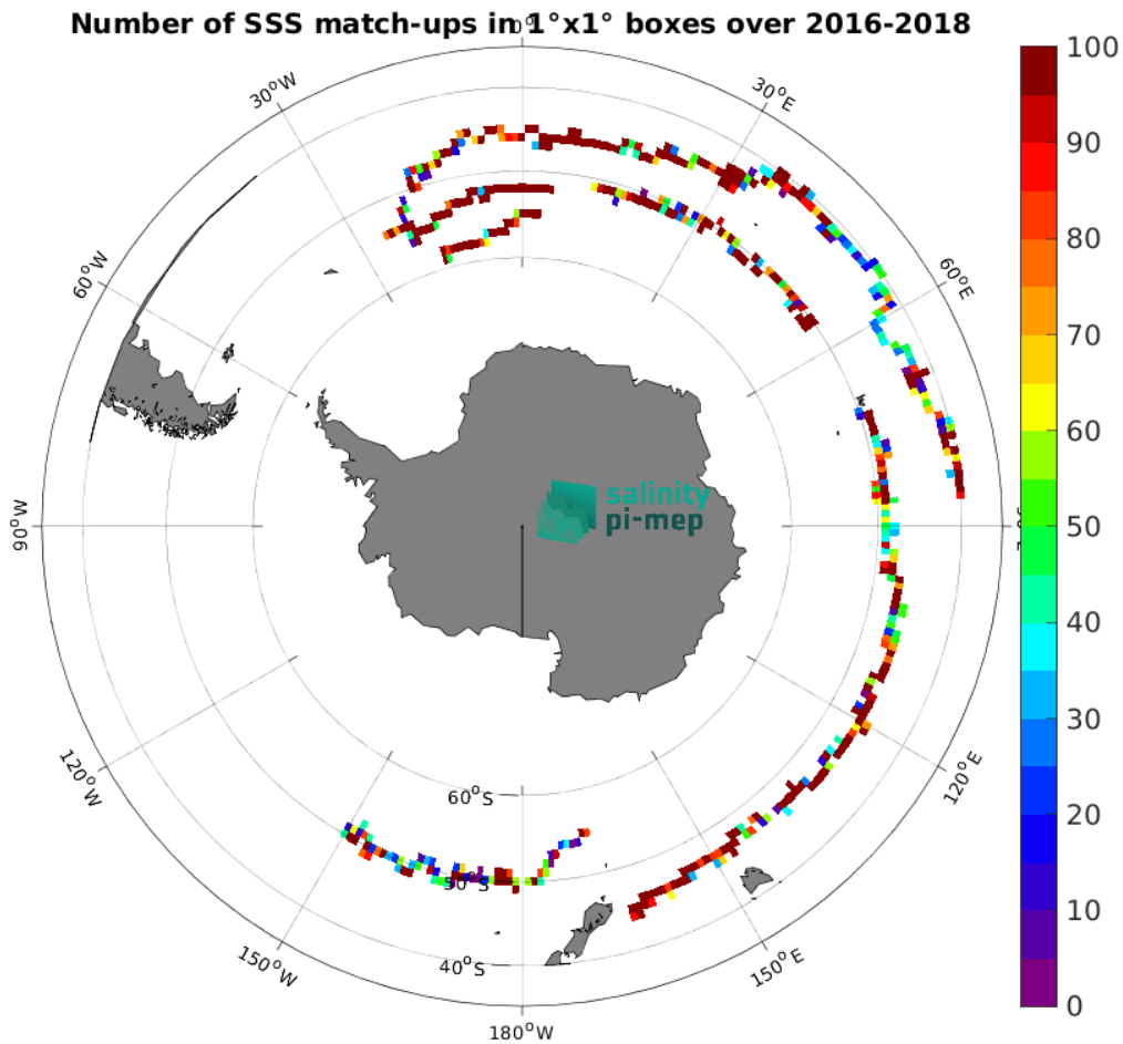
Figure 4: Number of SSS match-ups between Surface drifters SSS and the CCI SSS L4 Merged-OI v5.5 - 7-day running (ESA) SSS product for the Roaring Forties and Furious Fifties Pi-MEP region over 1^\circ \times 1^\circ boxes and for the full satellite product period.
