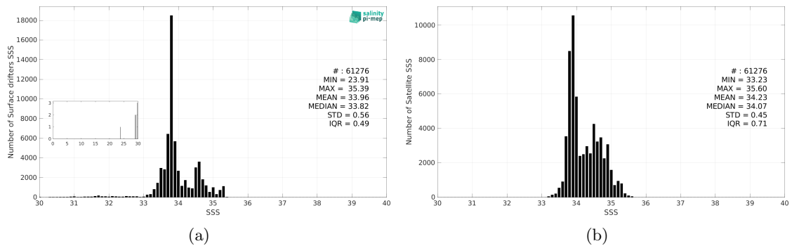
Figure 3: Histograms of SSS from Surface drifters (a) and CCI SSS L4 Merged-OI v5.5 - 7-day running (ESA) (b) considering all match-up pairs per bins of 0.1 over the Roaring Forties and Furious Fifties Pi-MEP region and for the full satellite product period.
