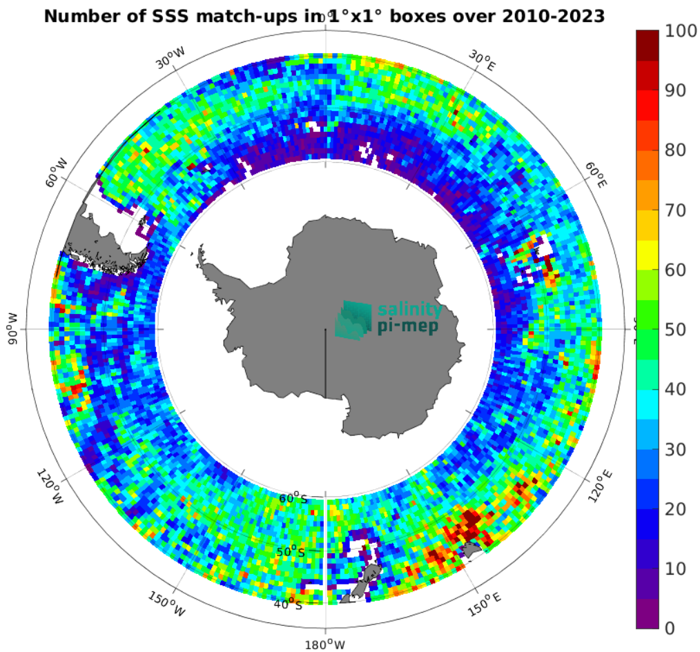
Figure 5: Number of SSS match-ups between Argo SSS and the CCI SSS L4 Merged-OI v5.5 - 7-day running (ESA) SSS product for the Roaring Forties and Furious Fifties Pi-MEP region over 1^\circ \times 1^\circ boxes and for the full satellite product period.
