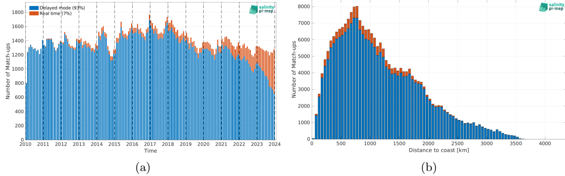
Figure 2: Number of match-ups between Argo and CCI SSS L4 Merged-OI v5.5 - 7-day running (ESA) SSS as a function of time (a) and as function of the distance to coast (b) over the Roaring Forties and Furious Fifties Pi-MEP region and for the full satellite product period.
