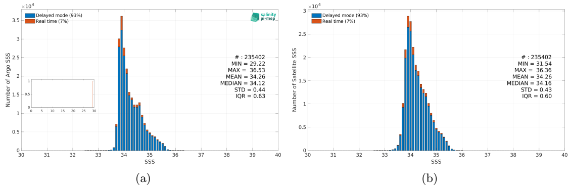
Figure 3: Histograms of SSS from Argo (a) and CCI SSS L4 Merged-OI v5.5 - 7-day running (ESA) (b) considering all match-up pairs per bins of 0.1 over the Roaring Forties and Furious Fifties Pi-MEP region and for the full satellite product period.
